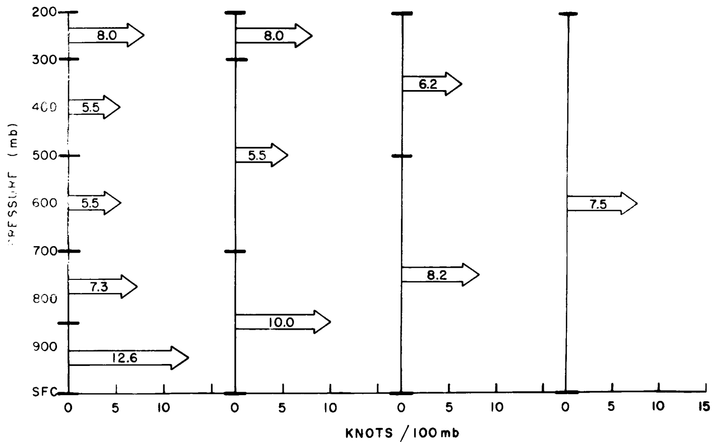
Fig. 3. Average magnitude of the vertical vector wind shear between standard pressure surfaces for the mid-latitude tornado environment. Selected standard pressure surfaces are marked with tick-marks along the vertical axes. The average shear (in knots per 100 mb) between any two consecutive tick-marks (pressure levels) is given by the horizontal arrow centered between the two tick-marks.
