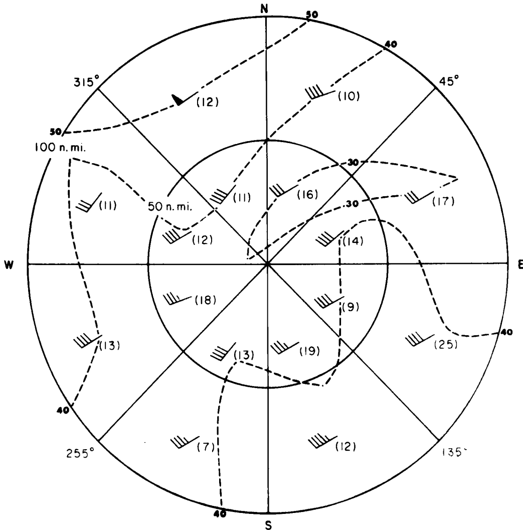
Fig. 16 (above). Compositied 500 mb vector winds (in knots) from 220 Great Plains tornado proximity soundings. The center of the circles is the position where the tornado occurred. The figure in parentheses denotes the number of observations which determined the resultant wind in that region. Isotachs are drawn with dashed lines.
