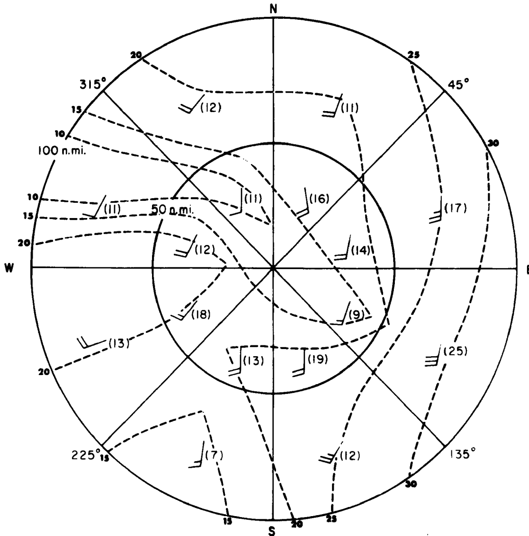
Fig. 10 (above). Compositied 850 mb vector winds (in knots) from 220 Great Plains tornado proximity soundings. The center of the circles is the position where the tornado occurred. The figure in parentheses denotes the number of observations which determined the resultant wind in that region. Isotachs are drawn with dashed lines.
