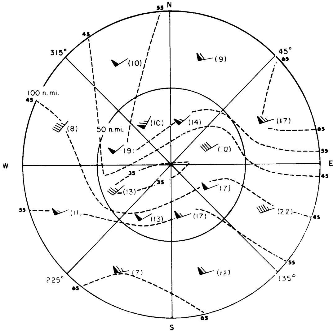
Fig. 22 (above). Compositd 200 mb vector winds (in knots) from 220 Great Plains tornado proximity soundings. The center of the circles is the position where the tornado occurred. The figure in parentheses denotes the number of observations which determined the resultant wind in that region. Isotachs are drawn with dashed lines.
