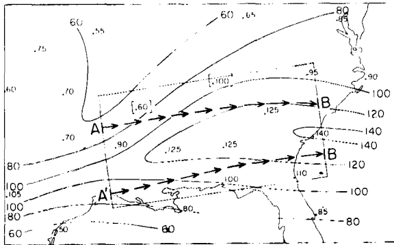
Fig. 12.22 Isotachs (knots) for the isentropic layer 360-370° A, 26 December 1958; bracketed winds extrapolated. Also streamlines north and south of jet axis across the box in fig. 10.12.
