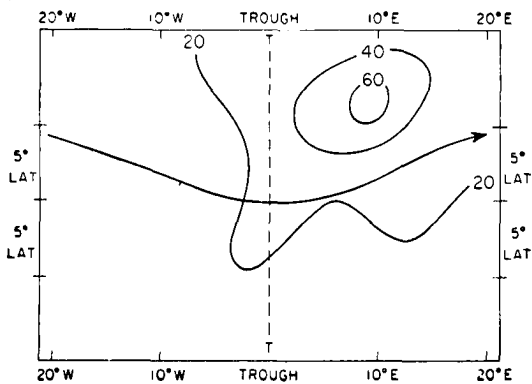
Fig. 8.21 Percent frequency of precipitation over the United States averaged relative to jet stream axis in 300-mb trough line when the hemispheric index of the westerlies is above average in low latitudes, (Jenista, 1953). Period of study: November 1951 through February 1952. Precipitation occurrence defined as measurable amount observed during 6 hours ending at 0630GCT; this interval was centered on the time of the upper-air charts.
