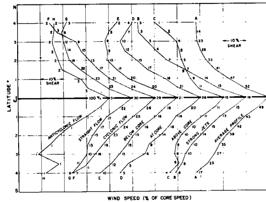
Fig. 2.7 Profiles of distribution of wind speed (in percent of core speed) for different types of jet streams encountered by Project Jet Stream of the U. S. Air Force (Endlich and McLean, 1957).
