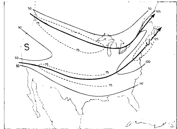
Fig. 7.5 Jet stream axes and isotachs, 20 November 1958, 00GCT.
