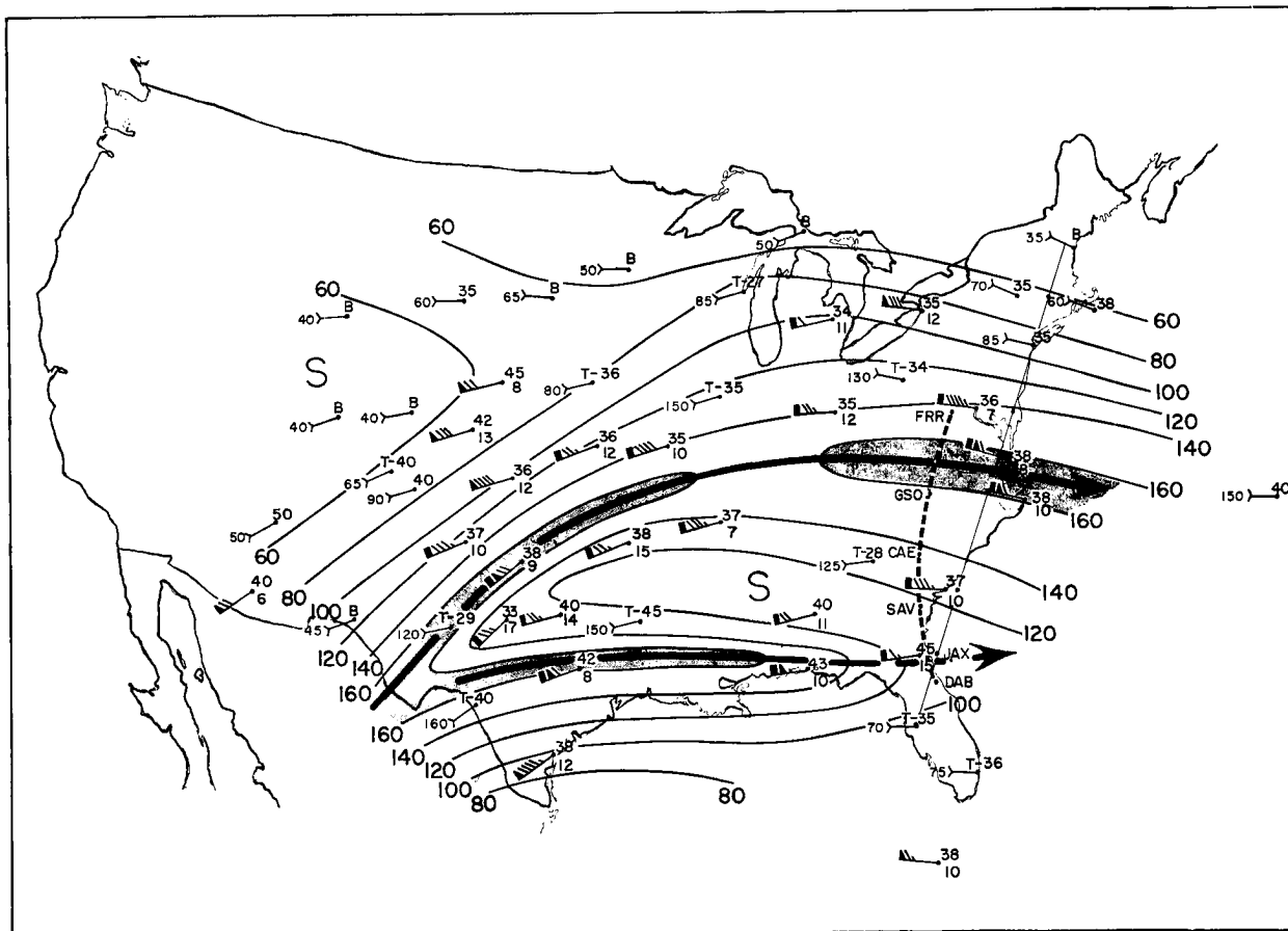
Fig. 4.1 LMW chart for 6 March 1958, 00GCT. Notation as in fig. 2.13. Light solid line along east coast outlines cross section shown in this section, heavy dashed line indicates research airplane track.
