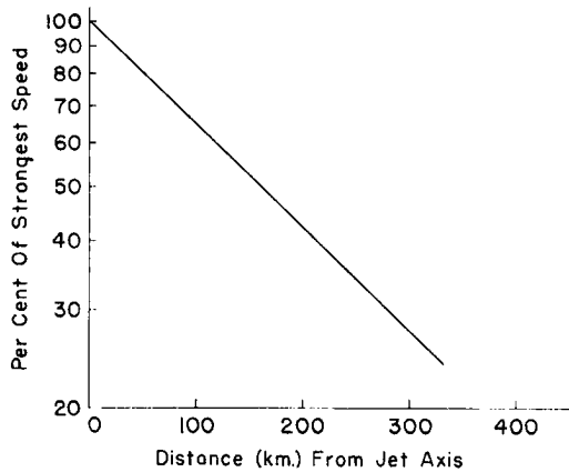
Fig. 2.9 Percent decrease of wind speed normal to jet axis to left of core looking downstream for several strong jet streams obtained by United States research aircraft (Riehl, Berry, Maynard, 1955).
