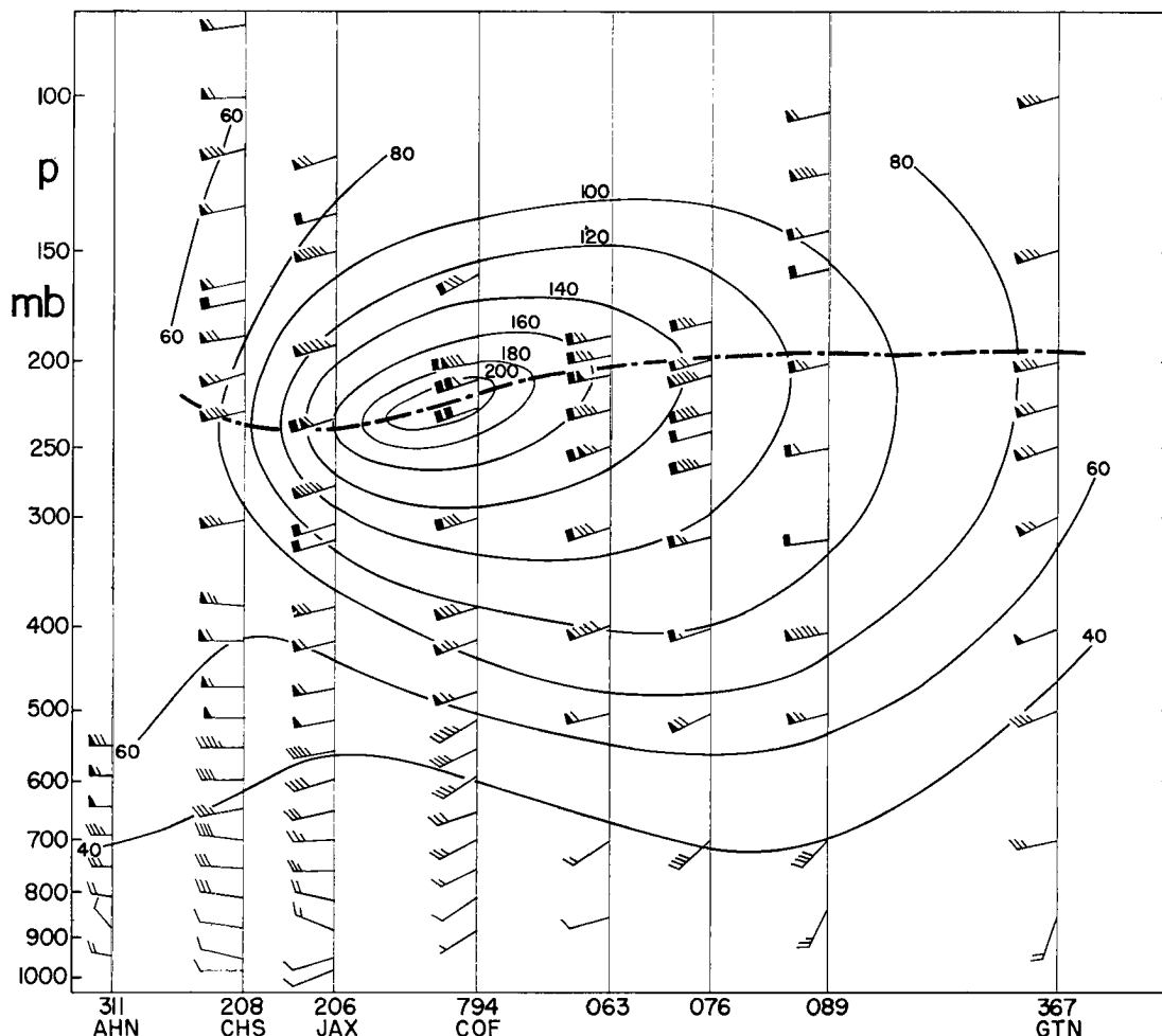
Fig. 5.10 Vertical cross section of wind speed (knots) along cross section marked in fig. 5.7, 11 February 1958, 00GCT. Heavy dash-dotted line indicates level of maximum wind.
