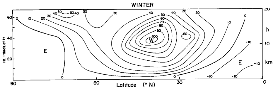
Fig. 9.14 Mean zonal wind speed (knots) at 80^{\circ} W in winter (after Kochanski, 1955).
