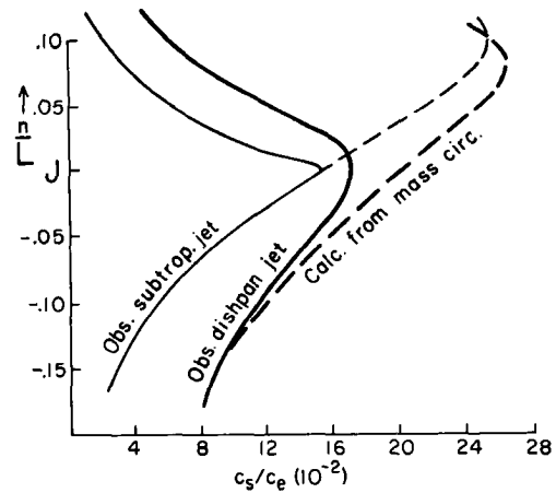
Fig. 12.33 Observed velocity profiles (fraction of equatorial pan speed and equatorial velocity of the earth) for three-wave dishpan experiment and subtropical jet stream of winter (solid) and profiles computed with constant-vorticity-transfer hypothesis (dashed).
