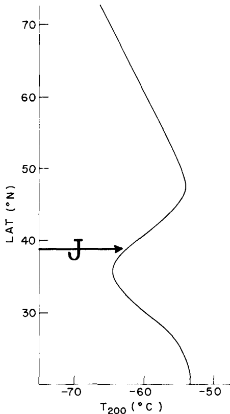
Fig. 3.4 Profile of 200-mb temperatures along section of fig. 3.2.
