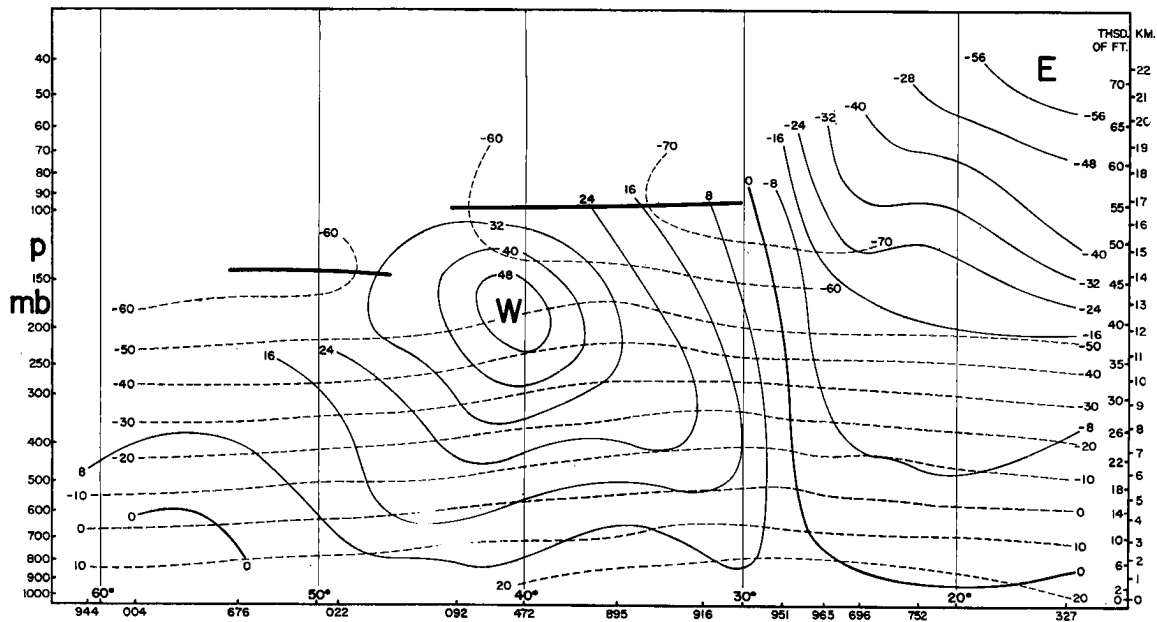
Fig. 9.21 Mean zonal wind speed (knots) and isotherms ( ^{\circ}\text{C} ) along longitude 120^{\circ}\text{E} in summer (Staff members, Academia Sinica, 1957).
