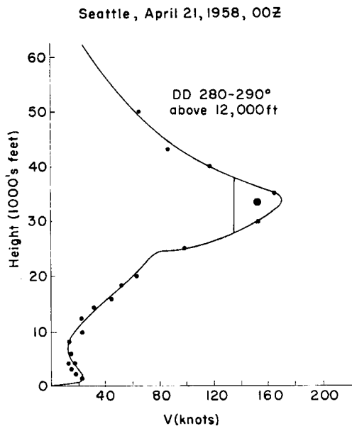
Fig. 2.1 Vertical wind profile at Seattle, Washington, 21 April 1958, 03Z.
