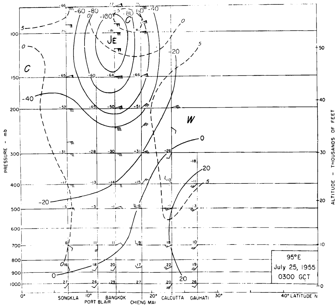
Fig. 5.15 Vertical cross section of easterly wind speed through subtropical jet stream axis at 95°E, 25 July 1955 (Koteswaram, 1958). Solid lines are isotachs (knots), dashed lines are lines of equal temperature anomaly from mean tropical summer atmosphere.
