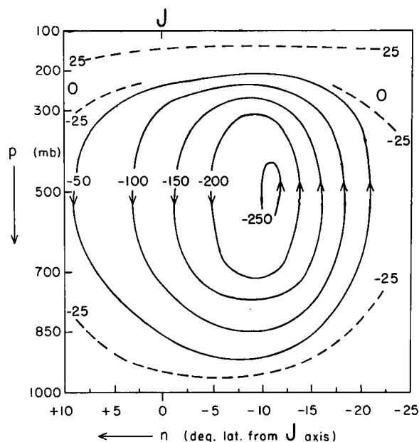
Fig. 5.6 Left: Vertical cross section of wind component normal to subtropical jet axis ( c_n , mps), in coordinate system fixed with respect to subtropical jet axis at 200 mb, for December 1955 (Krishnamurti 1959a). Negative sign denotes equatorward flow, positive sign poleward flow. Right: Stream function of the mass circulation in vertical plane normal to jet axis (multiply by 10^{12} g/sec for mass transport between isolines).
