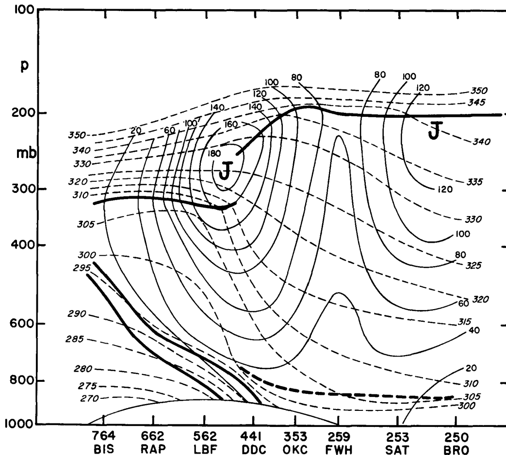
Fig. 3.3. North-south vertical cross section from Bismarck, North Dakota to Brownsville, Texas, 29 January 1947, 03Z (Riehl, 1948). Solid lines denote geostrophic west wind speed (knots), dashed lines isentropes ( ^{\circ} A). Heavy solid lines indicate frontal boundaries and tropopauses, heavy dashed lines subsidence inversions.
