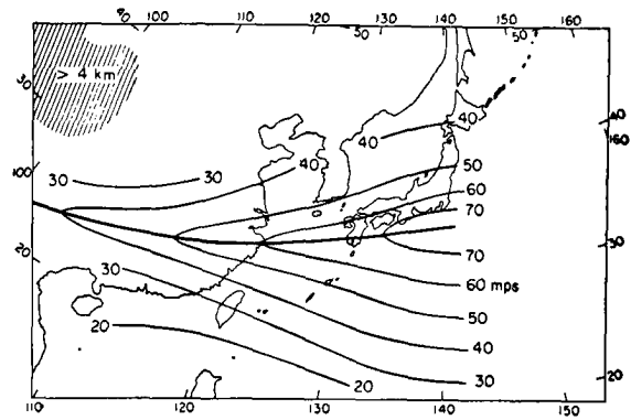
Fig. 9.19 Distribution of mean west wind speed (mps) at 12 kms over the Far East in winter (Mohri, 1953).
