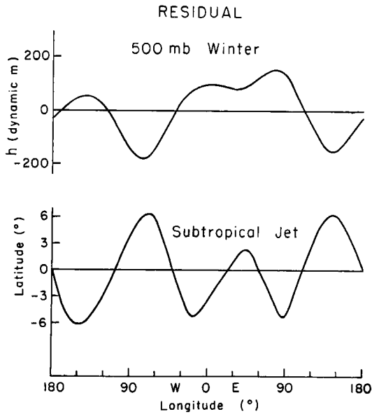
Fig. 9.9 Residual of the curves in figs. 9.6 and 9.7 after removal of mean and first harmonic.
