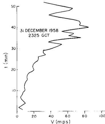
Fig. 10.1 Vertical profile of wind speed at Washington, D. C. in westerly jet stream, 31 December 1958. (Riehl and Mihaljan, 1959).
