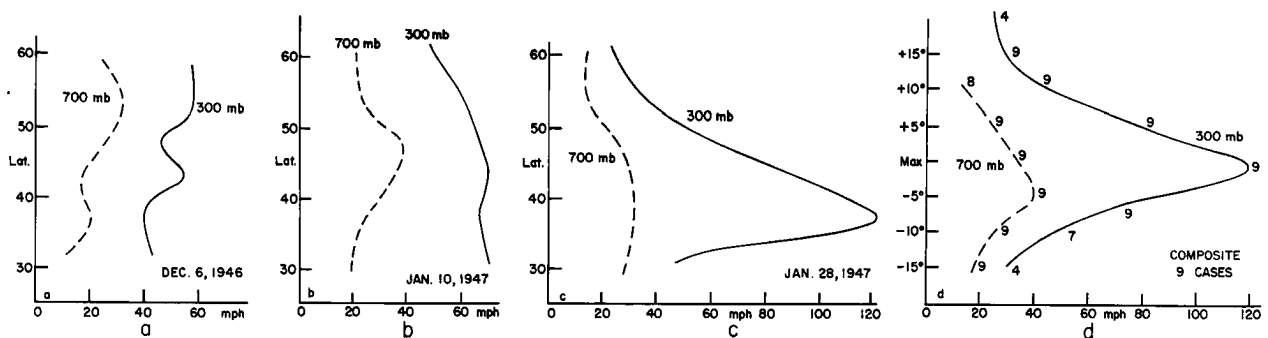
Fig. 8.1 Profiles of the westerlies at 700 mb and 300 mb over North America: a) 6 December 1946; b) 10 January 1947; and d) for nine cases with pronounced jet stream, averaged with respect to wind maximum at 300 mb. Ordinate in drawing (d) gives distance from zone of maximum wind at 300 mb in degrees latitude, numbers along curves indicate number of observations (Riehl, 1948).
