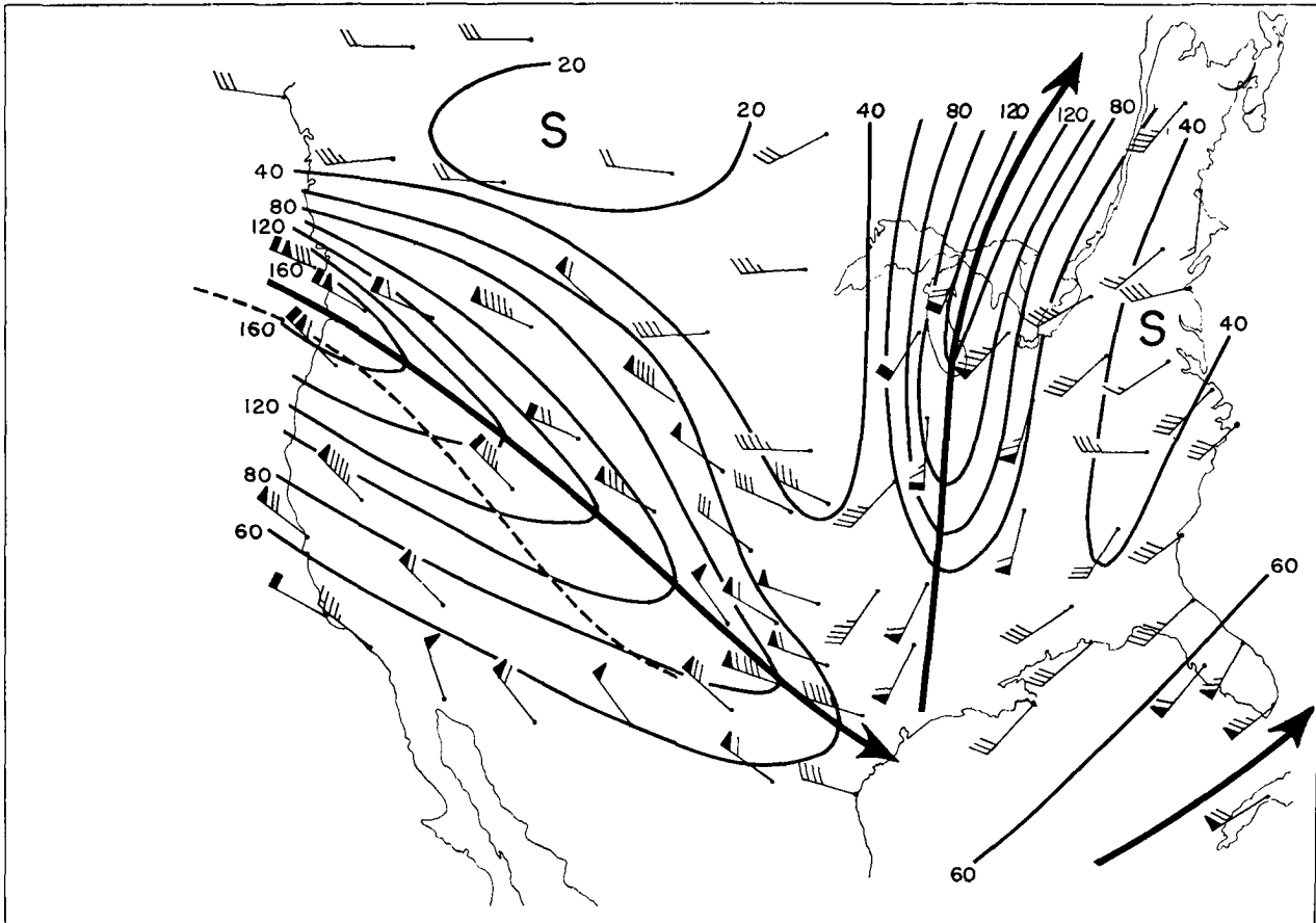
Fig. 2.11 300-mb winds, 21 April 1958, 00Z. Dashed line is previous jet axis position.
