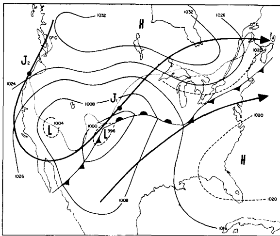
Fig. 8.2 Surface fronts and isobars, 16 November 1958, 0600GCT; also jet stream axes from Section VII. Dotted line is freezing isotherm at ground. Analysis copied from U.S. Weather Bureau chart.
