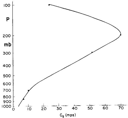
Fig. 5.3 Vertical distribution of wind components parallel to subtropical jet stream axis, ( c_s , mps) averaged around globe following the axis, December 1955 (Krishnamurti, 1959a).
