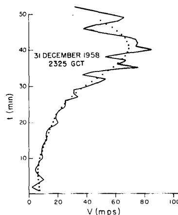
Fig. 10.3 Sounding of fig. 10.1 repeated (solid) and computed winds at one-minute intervals determined from first 5 harmonics.
