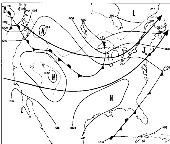
Fig. 8.6 Surface fronts and isobars, also jet axes, 20 November 1958, 0600GCT.
