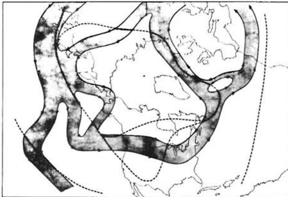
Fig. 7.8 Outline of hemispheric flow concentrations, 21 November 1958.
