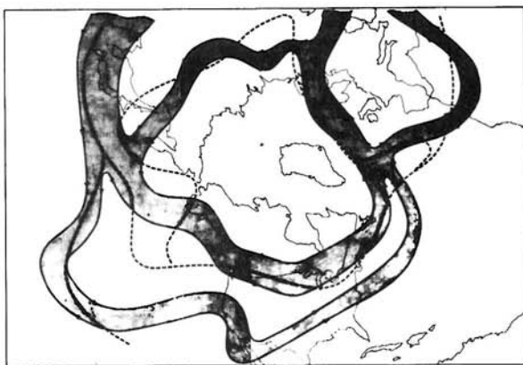
Fig. 7.9 Outline of hemispheric flow concentrations, 24 November 1958.
