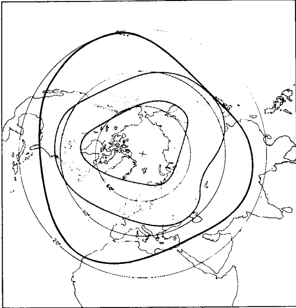
Fig. 1.2 Mean axis of subtropical jet stream during winter (solid), and area of principal activity of polar front jet stream in this season (shaded).
