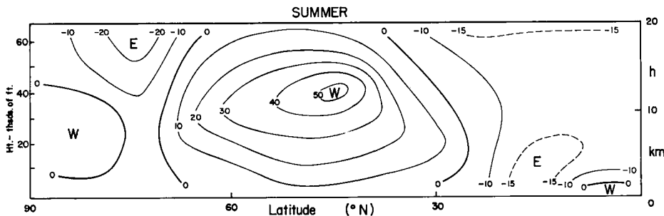
Fig. 9.15 Mean zonal wind speed (knots) at 80^{\circ} W in summer (after Kochanski, 1955).
