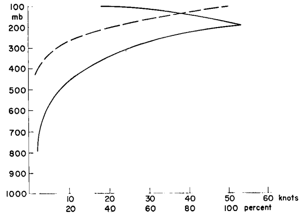
Fig. 5.14 Vertical profile (solid line) of easterly wind component through jet axis at 82^{\circ}W on 1 August 1953, 03GCT. Dashed line represents curve of cumulative percentage of kinetic energy from 1000 to 100 mb; for instance, value at 300 mb is 7 percent which means that 7 percent of the kinetic energy of the whole column from the ground to 100 mb lies below 300 mb, 93 percent above.
