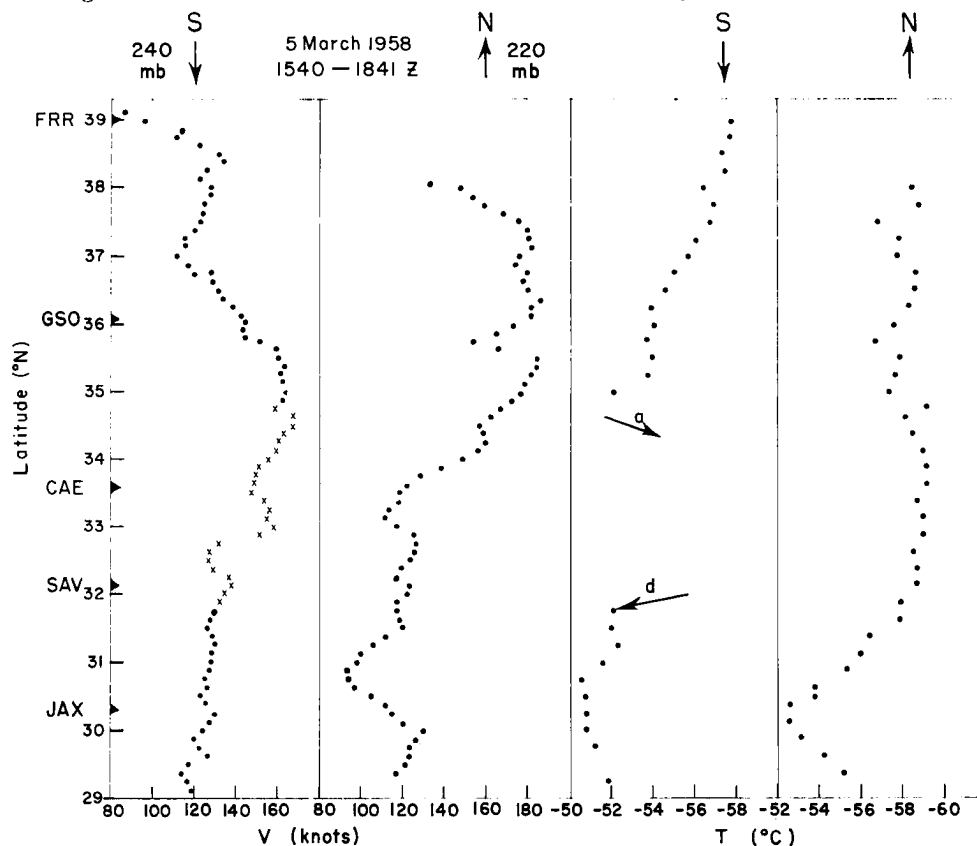
Fig. 4.8 Wind speed (knots) and temperature (°C) measured by A3D aircraft on route indicated in fig. 4.1, 5 March 1958. S southbound leg, N northbound leg. Two-minute mean winds are plotted every minute; crosses indicate data taken while airplane was at higher altitude. The temperatures are also averaged over two minutes, nonoverlapping.
