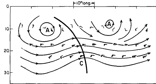
Fig. 10.18 Flow pattern for southern hemisphere, 25 September-5 October 1945, extrapolated eastward from longitudes 160-170°E using steady state assumption for the data of three stations located in the Solomons, Fijis and New Caledonia (Riehl, 1954b).
