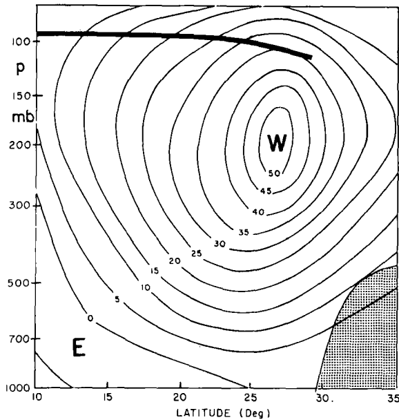
Fig. 9.18 Mean distribution of geostrophic zonal wind component (mps) over India in winter (Koteswaram, 1953).
