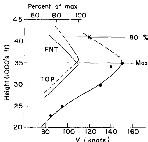
Fig. 10.9 Vertical wind profile at Peoria, Illinois (PIA), 6 March 1958, 0000GMT. Also portions of wind profiles of FNT and TOP, expressed in percent of the maximum wind at these stations. Extrapolated part of wind profile dashed.
