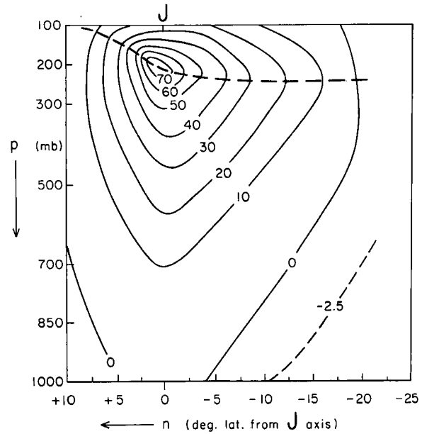
Fig. 5.4 Vertical cross section of wind component parallel to subtropical jet stream axis ( c_s , mps) in coordinate system fixed with respect to the jet axis at 200 mb, for December 1955 (Krishnamurti, 1959a).
