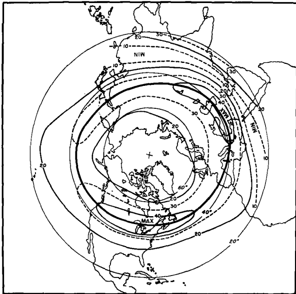
Fig. 9.5 Mean 200-mb isotachs (knots) for July 1949-53 (Wege, 1957).
