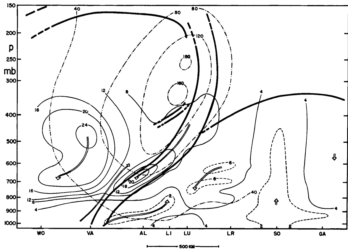
Fig. 3.11 Vertical cross section of dewpoint depression along a line extending NE-SW from Scandinavia across Britain to the ship station Weather Observer (WO) on 7 November 1952, (Vuorela,1957). Frontal boundaries and tropopause are indicated by heavy solid lines when distinct, and by heavy dashed lines when not distinct. Thin dash-dotted lines are observed wind speeds (knots). Thin solid lines are isolines of dewpoint depression ( ^{\circ}\text{C} ) and the arrows indicate the main directions of vertical movement as inferred from the humidity distribution.
