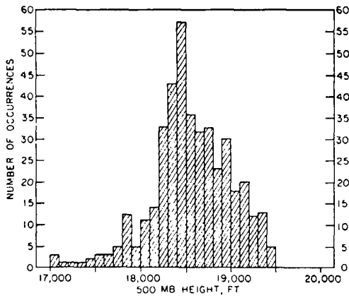
Fig. 10.16 Frequency distribution of 500-mb contour height at axis of strongest 500-mb wind from 255 maps, August-December 1958, over North America (Fletcher, 1953).
