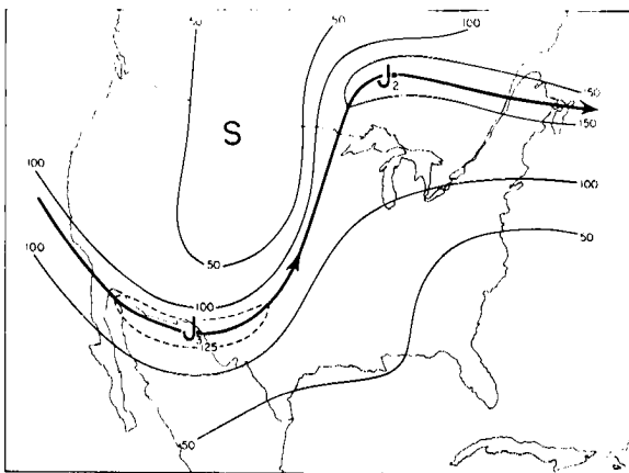
Fig. 7.3 Jet stream axes and isotachs, 18 November 1958, 00GCT.
