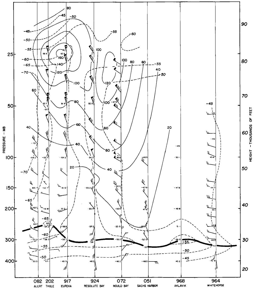
Fig. 6.4 Vertical cross section extending NE-SW from Alert to Whitehorse, 1500 GCT, 26 February 1956 (Lee and Godson, 1957). Solid lines are isotachs (knots), dashed lines isotherms ( ^{\circ}\text{C} ). Heavy solid line is tropopause. International station index used.
