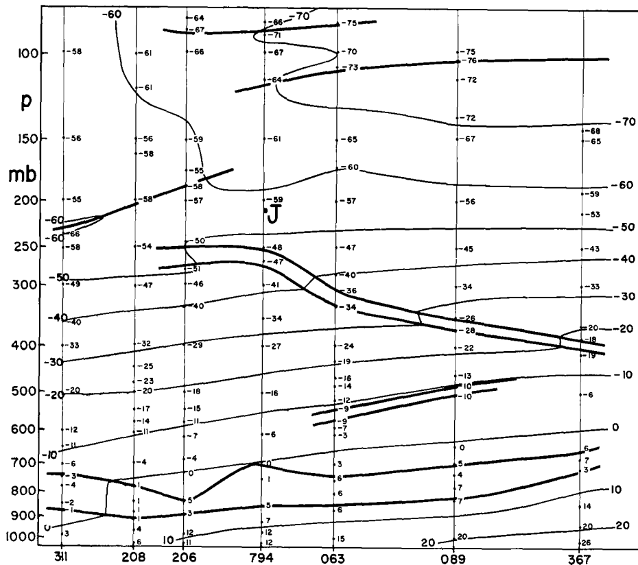
Fig. 5.11 Vertical cross section of temperature along line marked in fig. 5.7. Heavy lines denote subsidence inversions, fronts and tropopauses.
