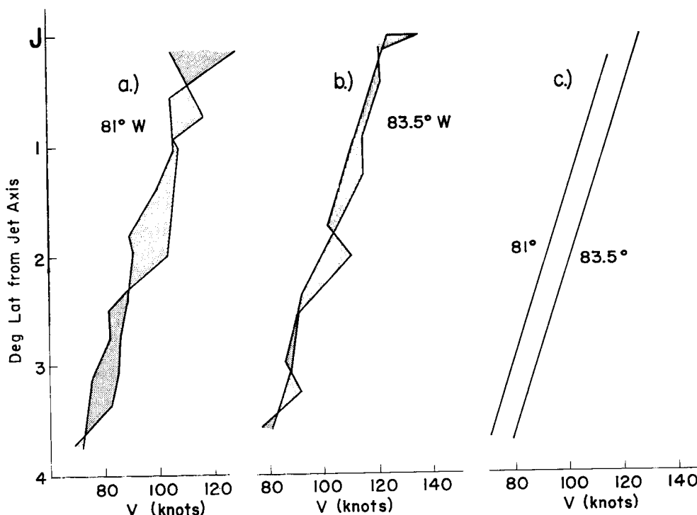
Fig. 10.4 Wind profiles determined on anticyclonic side of westerly jet stream over the United States on 1 November 1954 by U.S. Air Force B-47 research aircraft. Double profiles obtained from two quick round trips, time separation about two hours.
