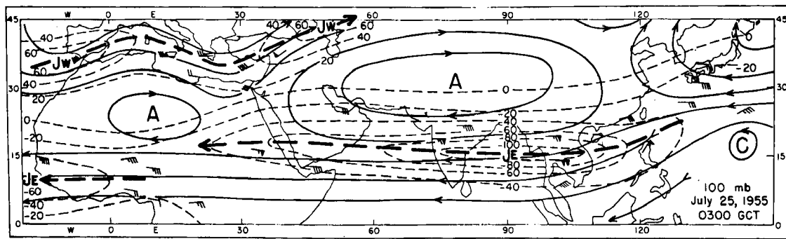
Fig. 5.16 Streamlines and isotachs (knots, negative sign denotes east component) at 300, 200 and 100 mb, 25 July 1955, 03GCT (Koteswaram,1958). A denotes anticyclonic circulation, C cyclonic circulation. Heavy dashed lines are easterly ( J_E ) and westerly ( J_W ) jet stream axes.
