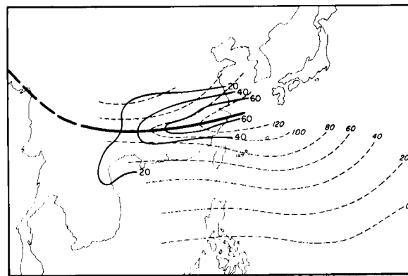
Fig. 8.20 Distribution of mean zonal wind speed (knots, solid lines) at 30,000 feet for December 1945 and January 1946; and mean precipitation (centimeters, dashed lines) over China in winter (Yeh, 1950).
