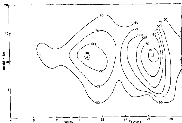
Fig. 11.2 Vertical time section of wind speed (knots) at Portland, Oregon, 25 February to 4 March 1954 (Reiter, 1957).
