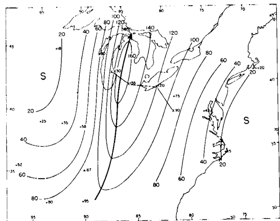
Fig. 12.14 300-mb isotachs (knots), 23 March 1953.
