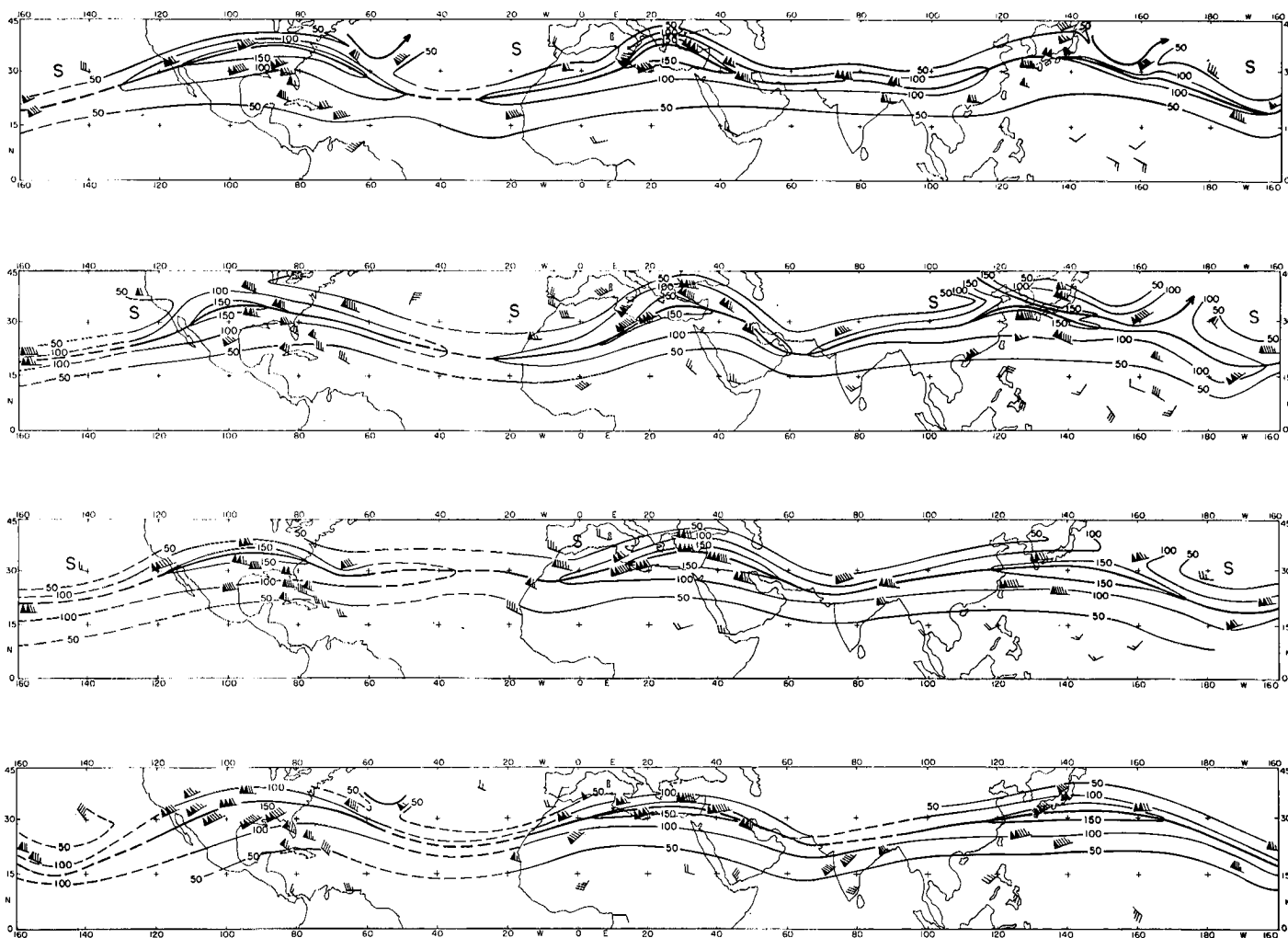
Fig. 5.2 Isotach analysis (knots) of subtropical jet stream at 200 mb, 25-28 February 1956 (top to bottom). Heavy line is jet axis, analyses dashed in areas without observations (Krishnamurti, 1959a).
