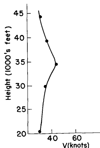
Fig. 10.8 Vertical wind profile at Lander, Wyoming (LND), 6 March 1958, 0000GMT.
