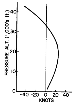
Fig. 11.8 TAS-pressure-altitude curve for maximum continuous power setting of the Boeing 707 with arbitrary zero setting at TAS near the surface.
