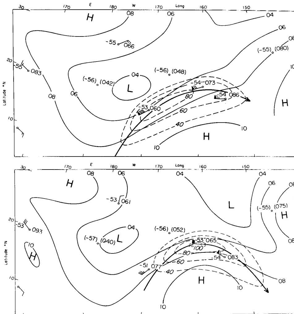
Fig. 5.12 200-mb contours (100's feet) and isotachs (knots) (dashed) for the central tropical Pacific, 24 July 1951 (upper) and 25 July 1951 (lower) (Riehl, 1954b).
