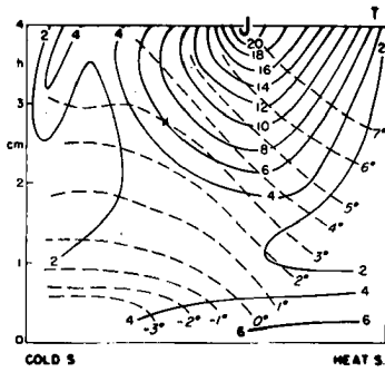
Fig. 12.29 Vertical cross section of wind speed (percent of equatorial pan speed) and temperature (departure from 16°C) for jet stream in steady three-wave experiment at trough line.
