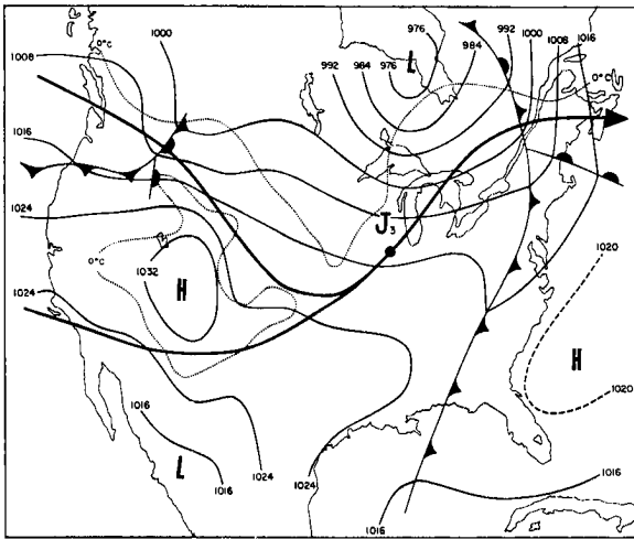
Fig. 8.5 Surface fronts and isobars, also jet axes, 19 November 1958, 0600GCT.
