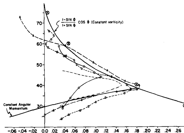
Fig. 12.2 Comparison between theoretical wind profiles observed from vorticity and momentum considerations (heavy lines) and some observed geostrophic wind profiles at the tropopause level (thin lines). Large circles represent solar rotation data. All velocities are expressed in percent of the linear equatorial velocity of the planet (Staff Members, 1947).
