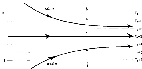
Fig. 12.17 Model of streamlines and patterns in 'confluence' zone (Namias and Clapp, 1949).
