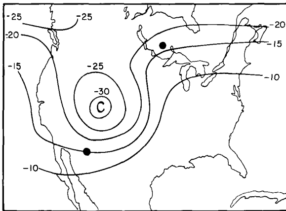
Fig. 8.9 500-mb isotherms ( ^{\circ}\text{C} ), 18 November 1958, 0000GCT.
