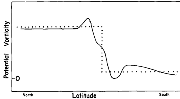
Fig. 12.20 Observed potential-vorticity cross section at level of strongest wind from fig. 12.4 (solid line) (Palmén and Newton, 1948) and two-layer model according to Platzman, 1949 (dotted).
