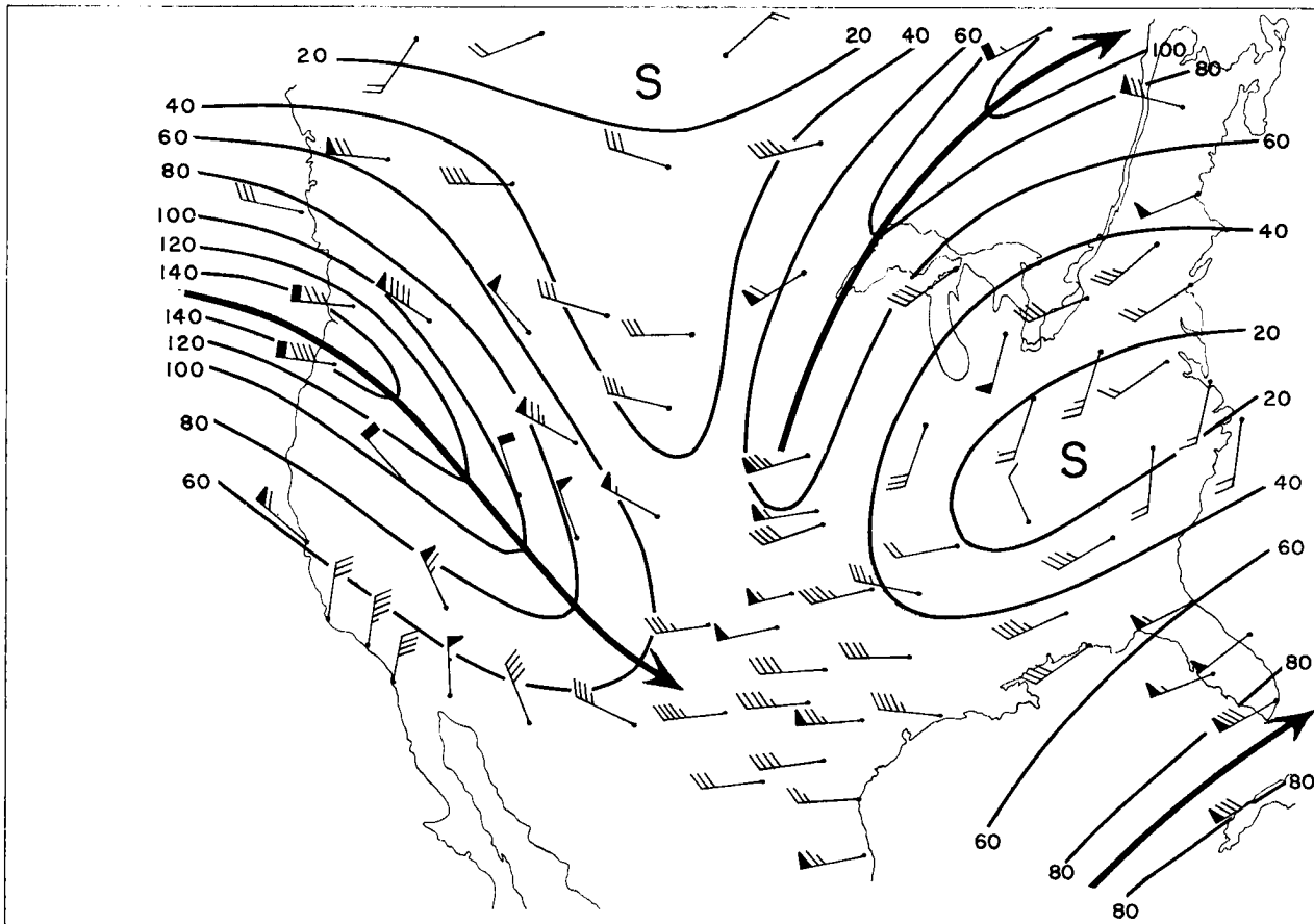
Fig. 2.10 300-mb winds, 20 April 1958, 00Z. Solid lines are jet stream axes, isotach analysis in knots, S denotes slow areas.
