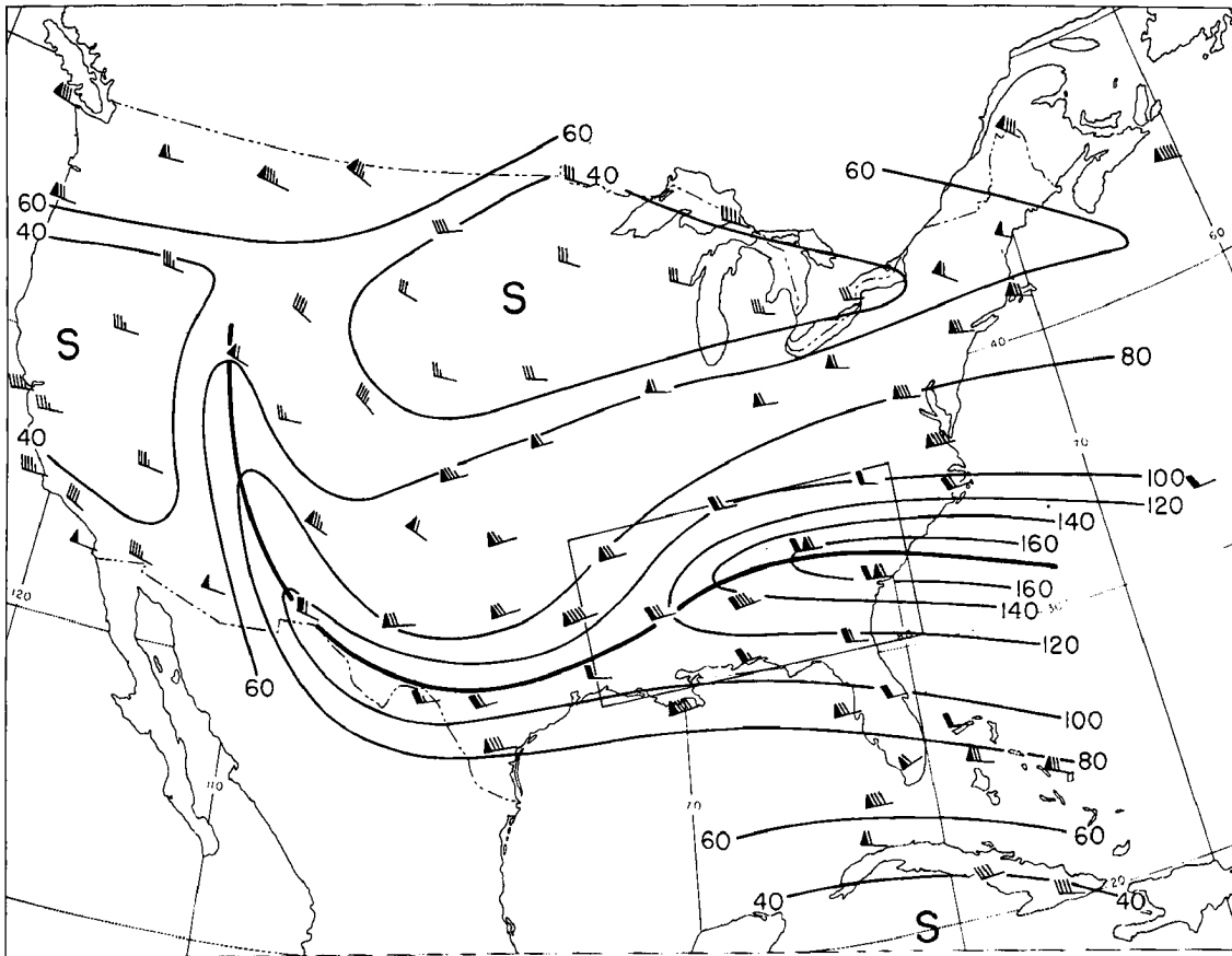
Fig. 10.12 LMW winds and isotach analysis (knots), 26 December 1958, 1200GMT.
