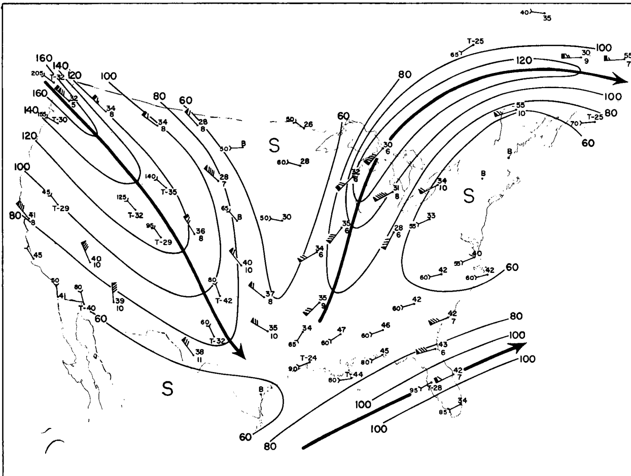
Fig. 2.13 Layer of maximum wind chart, 21 April 1958, 00Z. Wind arrows with barbs denote complete LMW winds. Height of LMW (1000's feet) entered to right of wind arrows, thickness of LMW (1000's feet) underneath. Open arrows indicate incomplete wind sounding, then letter T (top) is entered and height of top of sounding (1000's feet); or complete sounding without LMW. Speed entered in rear of arrow; B denotes barotropic sounding with nearly uniform speed; a height (1000's feet) at head of sounding indicates level of maximum wind.
