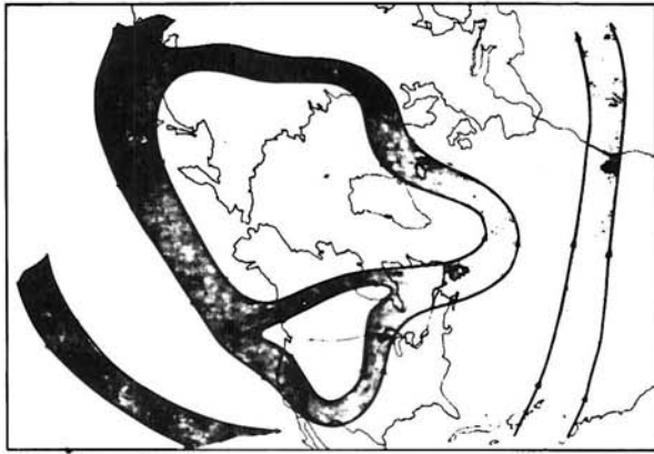
Fig. 7.7 Outline of hemispheric flow concentrations, 18 November 1958.
