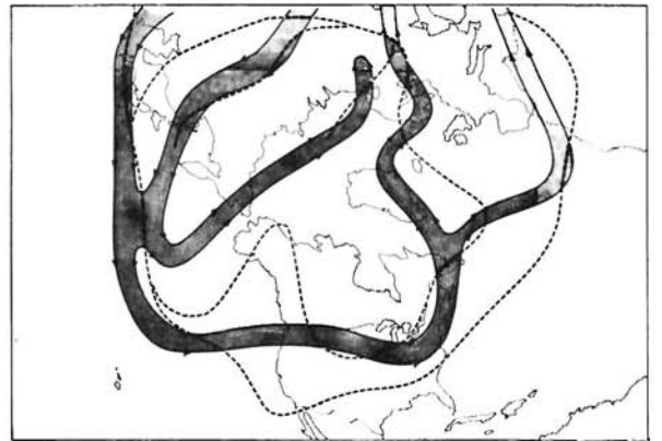
Fig. 7.11 Outline of hemispheric flow concentrations, 30 November 1958.
