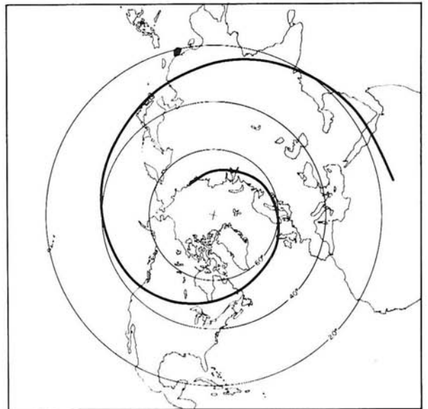
Fig. 7.12 Axis of first harmonic of 300-mb flow during winter (Barrett, 1958).
