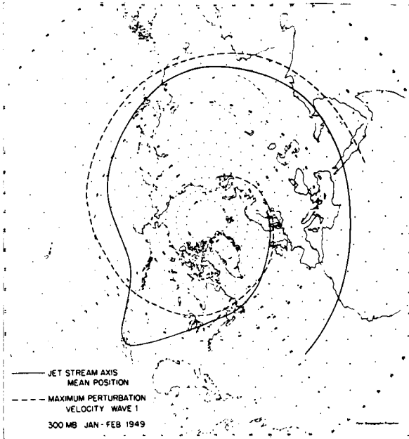
Fig. 9.12 Mean jet stream axis (solid) and axis denoting maximum westerly perturbation velocity from fig. 9.11 at 300 mb, January-February 1949 (Barrett, 1958).
