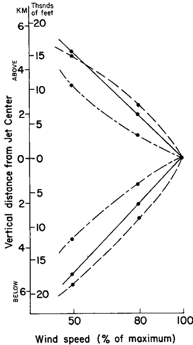
Fig. 2.4 Model of vertical distribution of wind speed assuming that 45 percent of thickness of layer of maximum wind lies above jet axis and 55 percent below. Solid line as in fig. 2.3; dash-dotted: LMW thickness 2200 m; dashed: LMW thickness 5000 m (Reiter, 1958).
