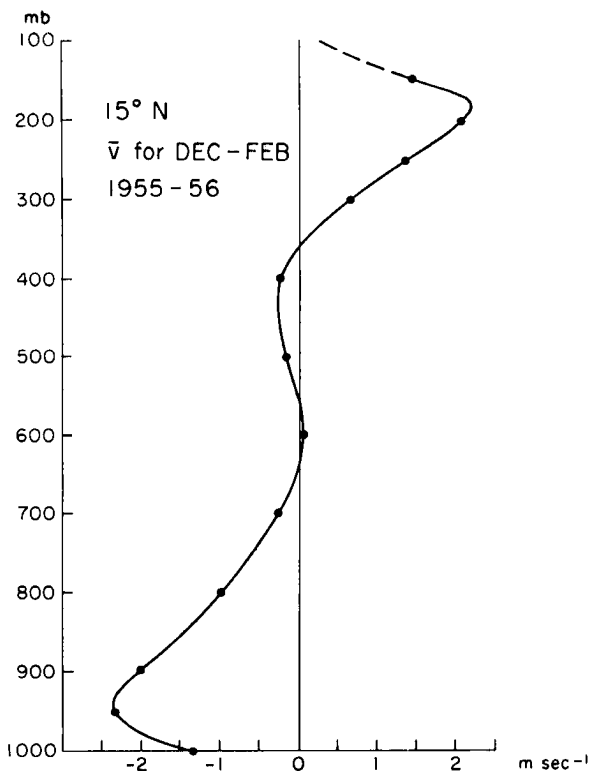
Fig. 12.6 Mean meridional wind component (m/s) for latitude 15^{\circ} N, December 1955 - February 1956, as a function of pressure (Palmén, Riehl, Vuorela, 1958).
