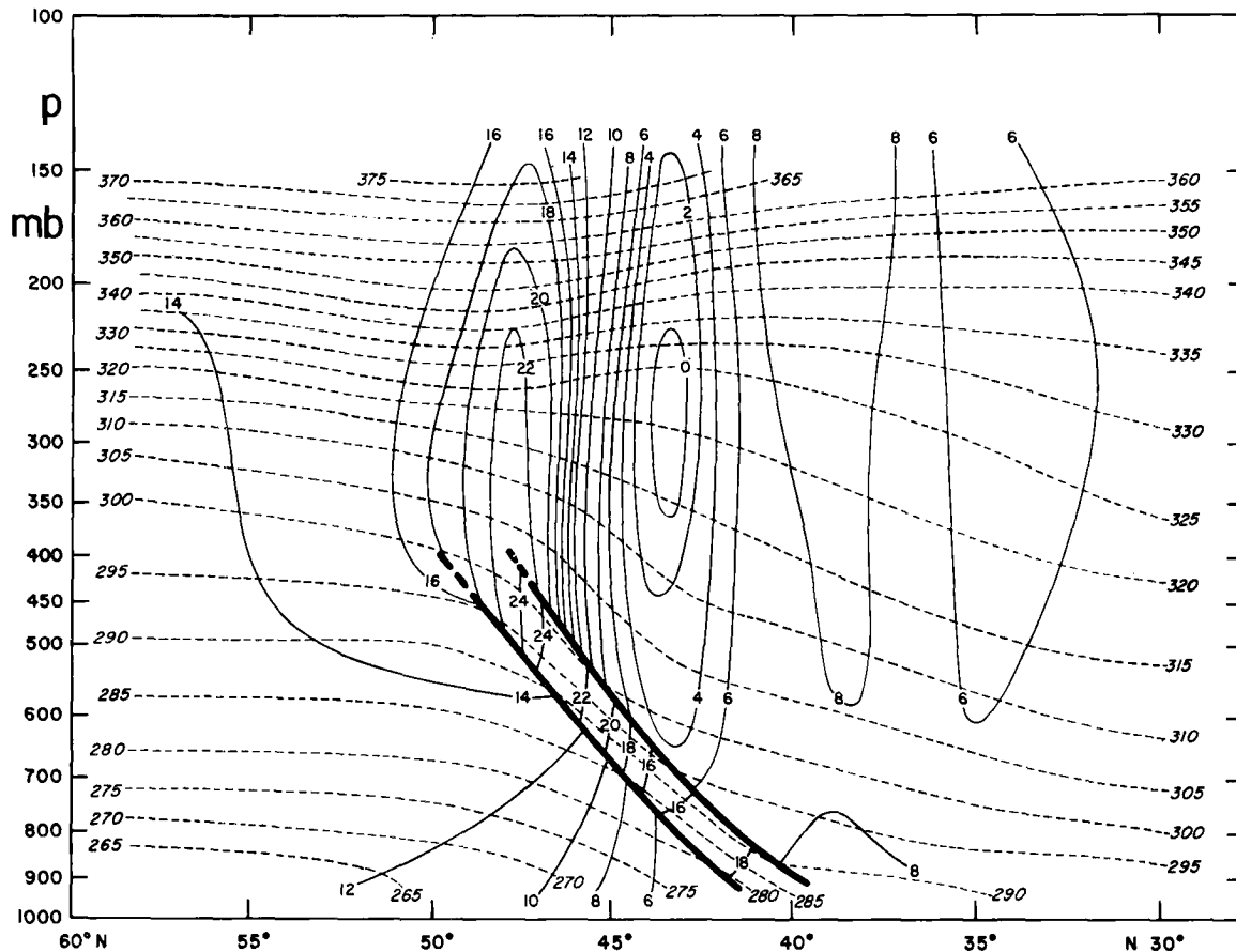
Fig. 12.4 Mean absolute vorticity computed on isobaric surfaces (solid lines, unit 10^{-5} \text{sec}^{-1} ) and potential temperatures (dashed lines, ^{\circ}\text{A} ) for wind field of fig. 3.5 (Palmén and Newton, 1948).
