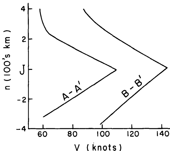
Fig. 12.24 Velocity profiles normal to jet axis in the isentropic layer 360-370° A at western and eastern ends of the box in fig. 12.22.
