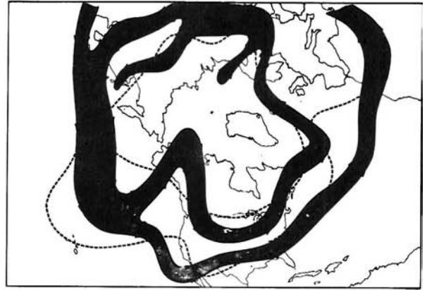
Fig. 7.10 Outline of hemispheric flow concentrations, 27 November 1958.
