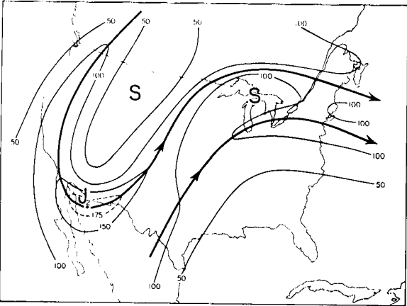
Fig. 7.2 Jet stream axes and isotachs, 17 November 1958, 00GCT.
