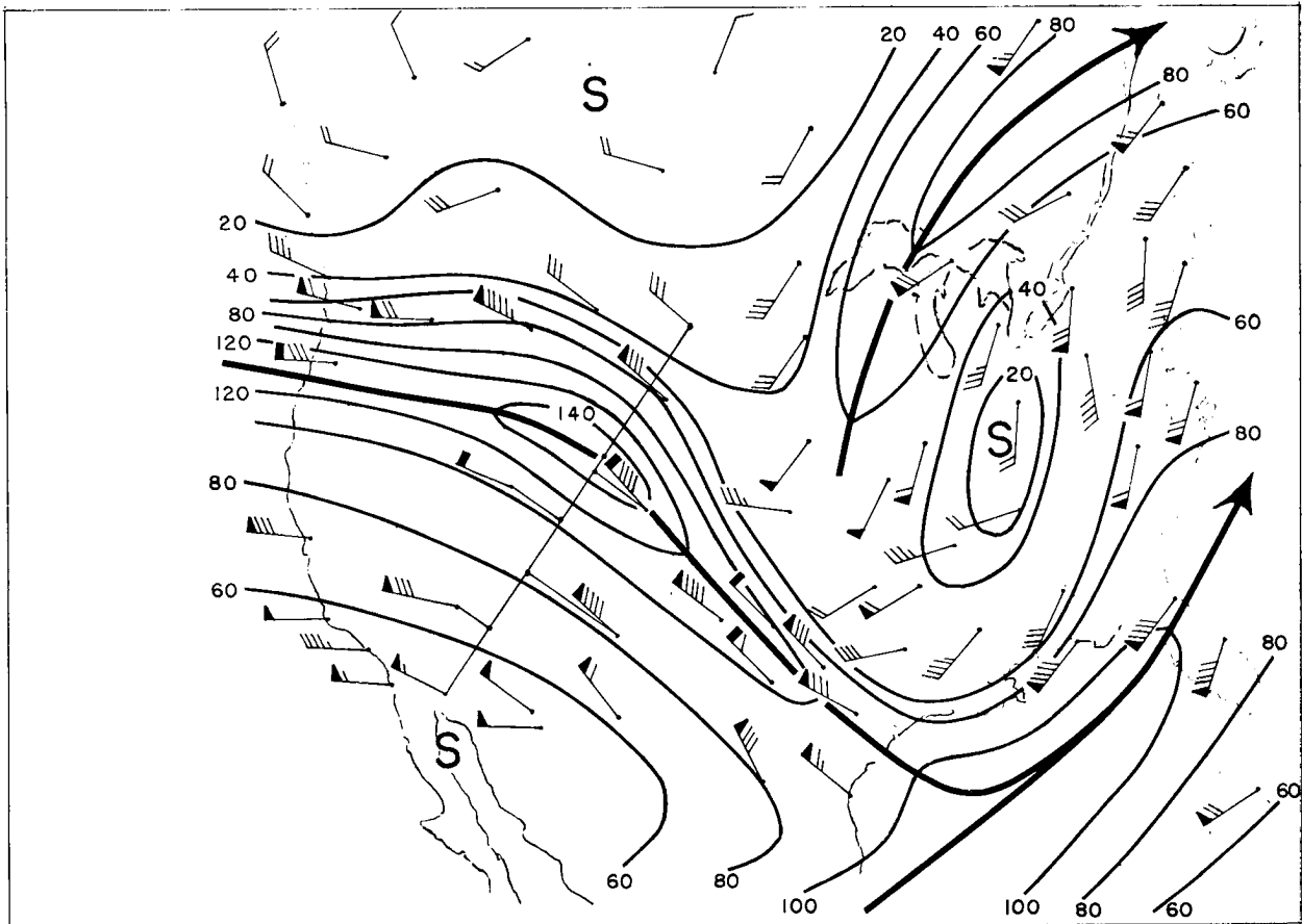
Fig. 2.12 300-mb winds, 22 April 1958, 00Z, and layout of cross section for fig. 2.16.
