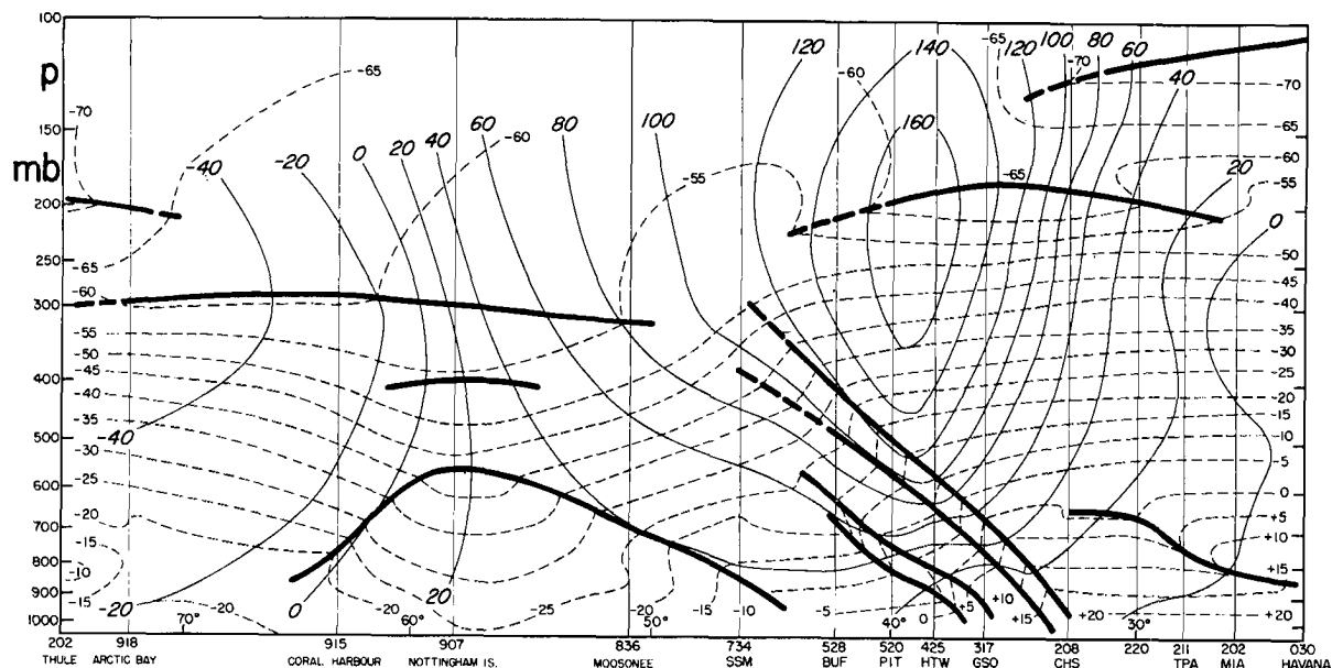
Fig. 3.2 Vertical cross section approximately at 80^\circ W from Havana to Thule, 17 January 1947, 03Z (Palmén, 1948). Frontal boundaries, inversions or tropopause surfaces are indicated by thick solid lines when distinct, and by thick dashed lines when not distinct. Thin solid lines indicate geostrophic wind velocity (knots) perpendicular to the section, dashed lines isotherms ( ^\circ\text{C} ).
