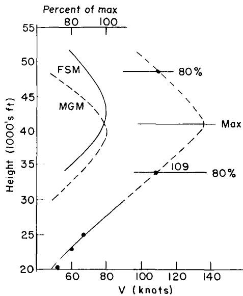
Fig. 10.10 Vertical wind profile at Jackson, Mississippi (JAN), 6 March 1958, 0000GMT. Also portions of wind profiles at FSM and MGM, expressed in percent of the maximum wind at these stations. Extrapolated part of wind profile dashed.
