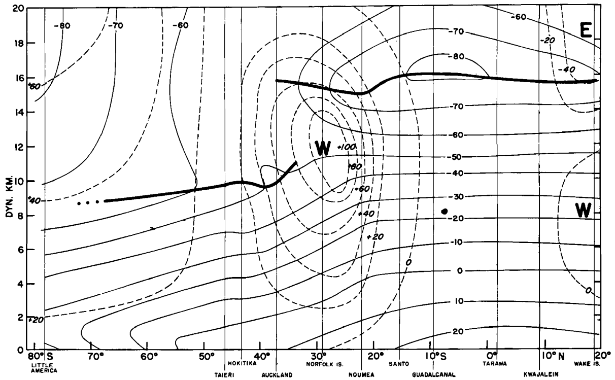
Fig. 9.23 Distribution of mean zonal geostrophic west wind speed (knots) and temperature ( ^{\circ}\text{C} ) along 170^{\circ}\text{E} in southern hemisphere, winter (Hutchings, 1950).
