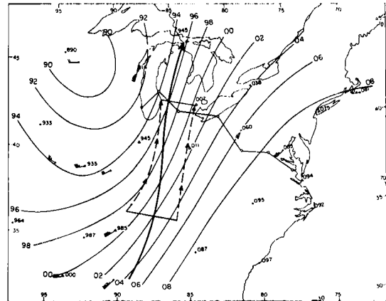
Fig. 12.13 300-mb contours (100's feet, first digit omitted), 23 March 1953 (Riehl, 1954a). Heavy line marks jet axis; line extending from east coast to Lake Michigan is path taken by research aircraft.
