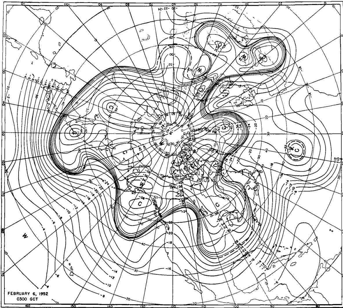
Fig. 3.1 Temperature distribution ( ^{\circ}\text{C} ) at 500 mb, 6 February 1952, 03Z (Bradbury and Palmen, 1953). The heavy line marks the approximate southern limit of the polar air including the frontal zone.
