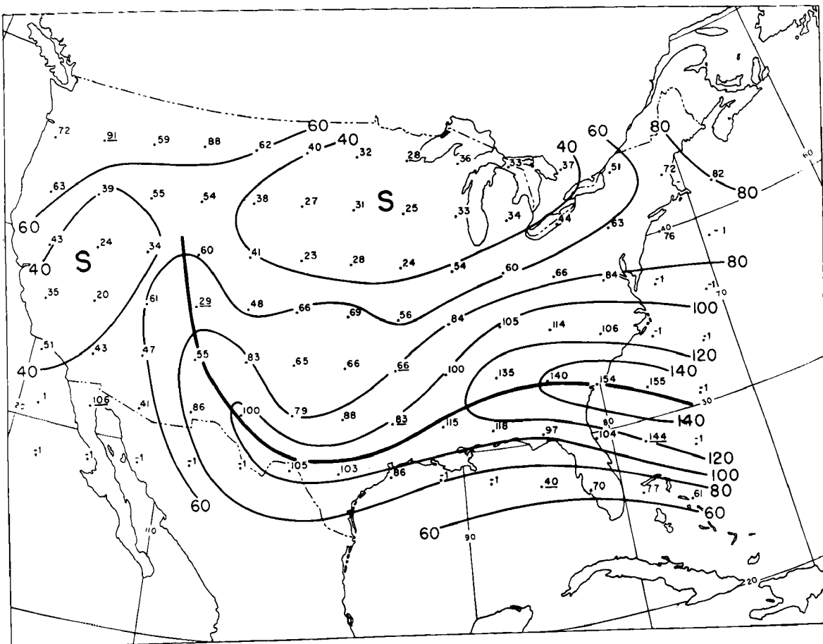
Fig. 10.13 Machine-computed wind speeds and isotachs (knots), 26 December 1958, 1200GMT (Riehl and Mihaljan, 1959). Winds omitted in analysis are underlined.
