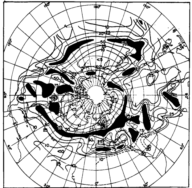
Fig. 9.13 Rate of alternation (percent) between cyclones and anticyclones during the winter season, indicating the distribution of traveling disturbances. The ration of alternation is defined as the ratio (F_c/F_a) when F_c < F_a , or by F_a/F_c when F_c > F_a where F_c and F_a denote the percentage frequencies of occurrences of cyclone and anticyclone centers, respectively, in a given 100,000 km square (Petterssen, 1950).
