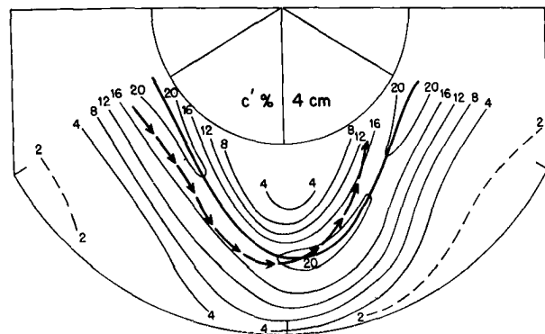
Fig. 12.28 Velocity (in percent of the equatorial pan velocity) at top surface in steady three-wave dishpan case (Riehl and Fultz, 1957). Heavy solid line marks jet axis, dashed line with arrows trajectory crossing over axis.
