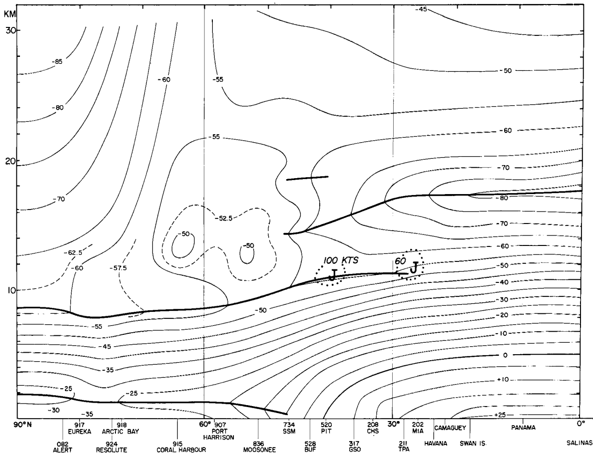
Fig. 6.1 Mean vertical temperature distribution (°C) along 80°W during winter, with tropopauses, ground inversions and location of main jet stream centers (after Kochanski, 1955).
