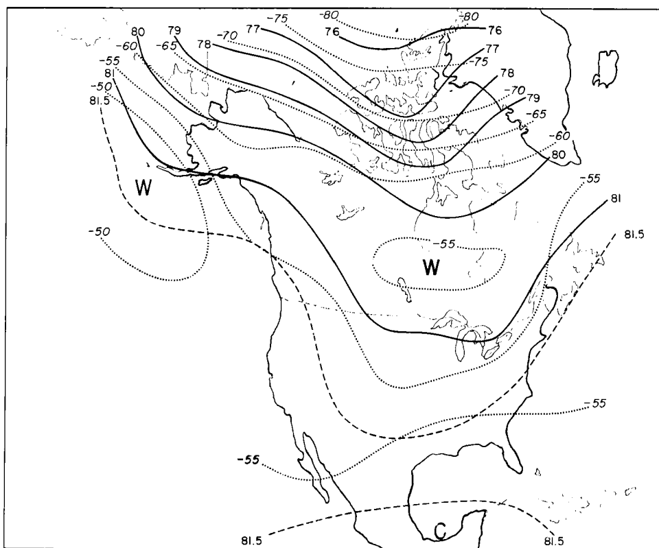
Fig. 6.2 25-mb contours (1000's feet) and isotherms (°C) for winter (after Kochanski, 1955).
