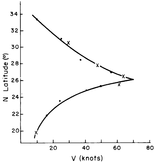
Fig. 5.13 Lateral distribution of easterly wind speed at 200 mb from southeastern United States across Florida and the Bahamas to Cuba, 1-2 August 1953 (Alaka, 1958).
