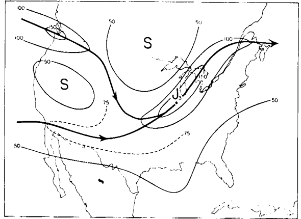
Fig. 7.4 Jet stream axes and isotachs, 19 November 1958, 00GCT.
