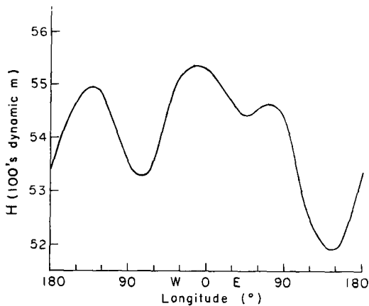
Fig. 9.6 Mean height of the 500-mb surface as a function of longitude at latitude 47.5^\circ\text{N} in winter (from Bryson et al, 1957).
