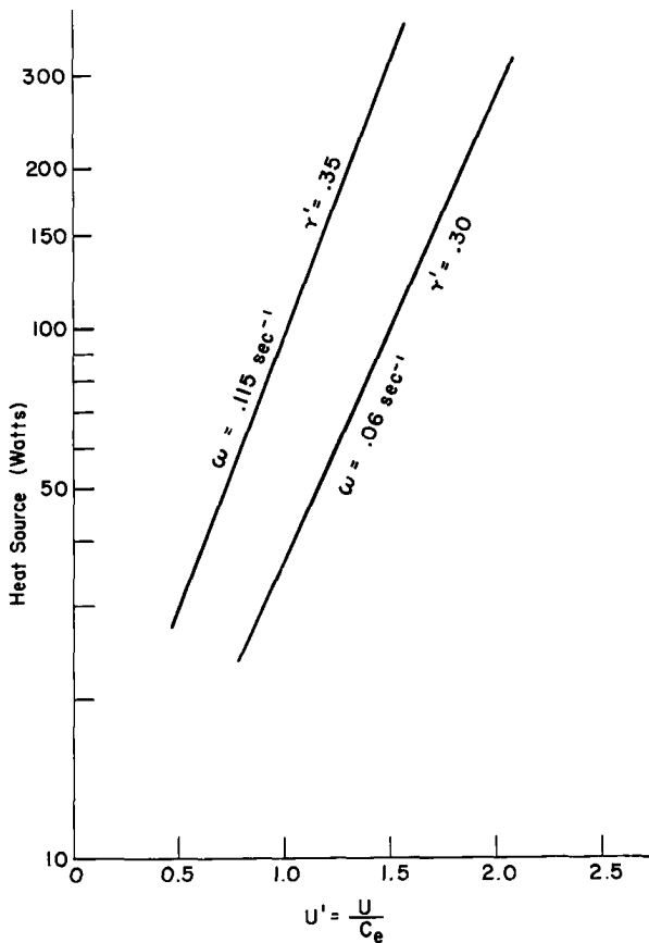
Fig. 12.27 Variation of jet velocity with heating rate at top surface in symmetrical dishpan experiments for two angular-rotation rates of the dishpan. Radius of jet core indicated in fractions of the radius of the pan. Cold-source wall at r' = 0.25 .
