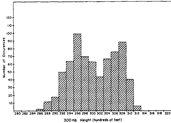
Fig. 11.10 Frequency distribution of the average 300 mb height along which a vertical projection of the LMW jet axis onto the 300 mb surface falls (U.S. Navy, 1959).
