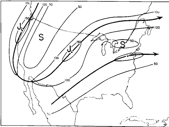
Fig. 7.1 Jet stream axes and isotachs (knots), 16 November 1958, 00GCT. Principal high-speed centers are numbered for continuity. J denotes high-speed center, S slow area.
