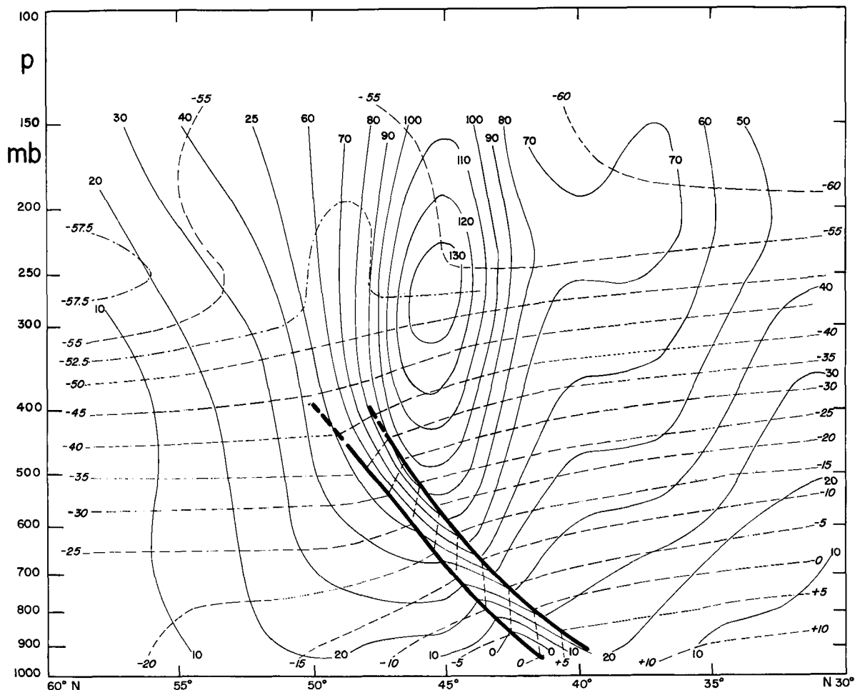
Fig. 3.5 Mean temperature and zonal component of geostrophic wind, computed from 12 cases in December, 1946. The cross section lies along the meridian 80^{\circ} W. Heavy lines indicate mean positions of frontal boundaries. Thin dashed lines are isotherms ( ^{\circ} C, slanting numbers) and solid lines are isolines of westerly component of wind (knots, upright numbers). Means were computed with respect to the polar front (Palmén and Newton, 1948).
