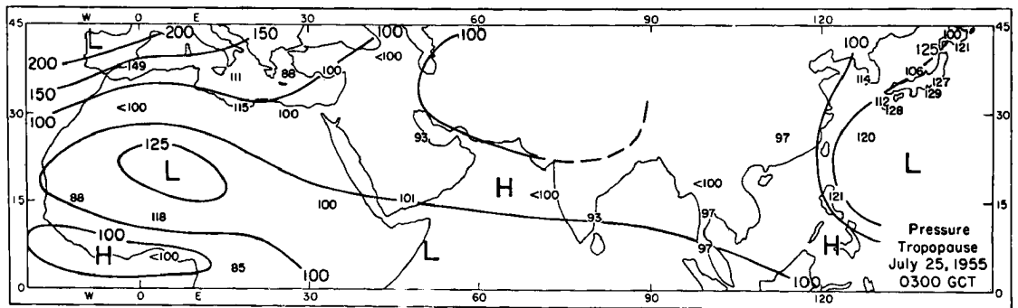
Fig. 5.17 Isotherms ( ^{\circ}\text{C} ) at 200 and 100 mb and isobars of pressure at tropopause (mb), 25 July 1955, 03GCT (Koteswaram, 1958).
