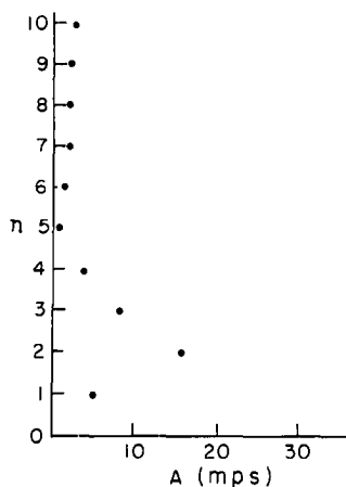
Fig. 10.2 Amplitude of the first 10 harmonics for the sounding of fig. 10.1.
