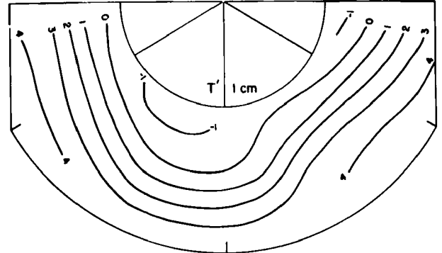
Fig. 12.31 Temperature at 1 cm depth in steady three-wave experiment (departure from 16°C).
