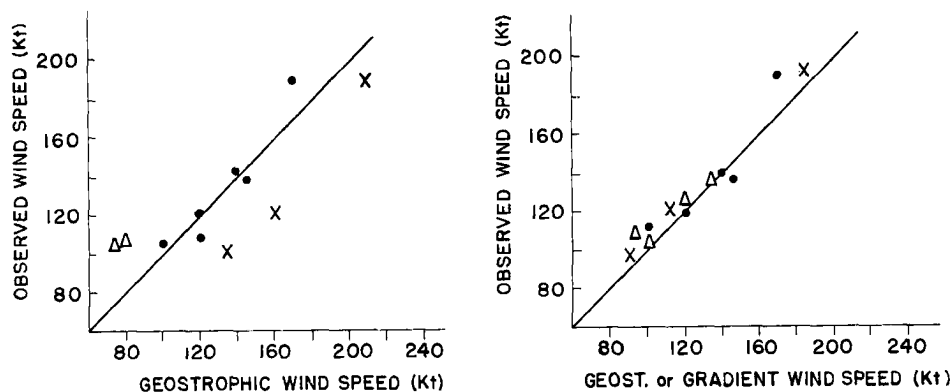
Fig. 10.15 Comparison of computed winds and of winds observed by research aircraft near 300 mb in several jet streams during winter of 1952-53 (Riehl, Berry, Maynard, 1955). Left: geostrophic winds, right: gradient wind correction included. Cases with straight flow marked by dots, with cyclonic flow by crosses and with anticyclonic flow by triangles. Computed and observed winds are means over 300-mb contour intervals of 600 to 1000 feet.
