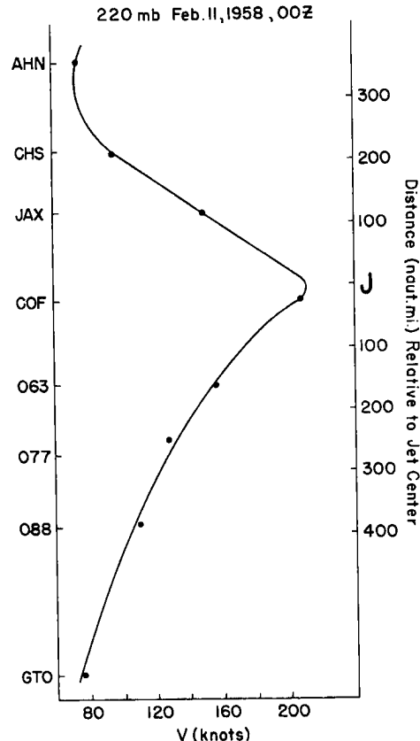
Fig. 5.9 Lateral profile of wind speed at 220 mb, 11 February 1958, 00GCT, along cross section marked in fig. 5.7.
