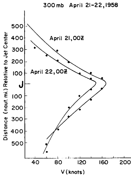
Fig. 2.6 Profiles of wind speed normal to jet axis at 300 mb over western United States. Center of profile taken in high-speed center just east of Pacific coast on 21 April (fig. 2.11); cross section outlined for 22 April in fig. 2.12.
