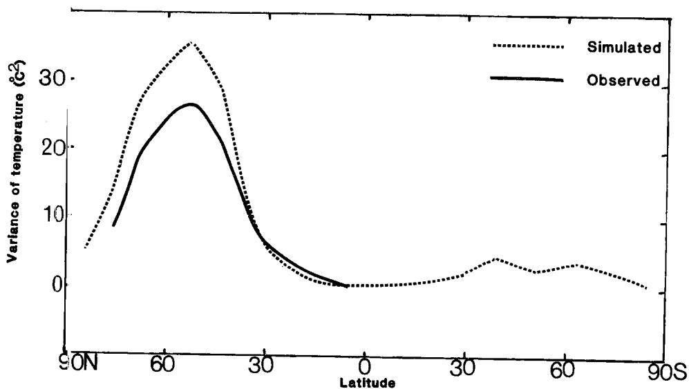
3.13 The tropospheric average of the observed (full line) and simulated (dotted line) zonally averaged variance of temperature ( ^{\circ}\text{C}^2 ) resulting from stationary eddies for January.
