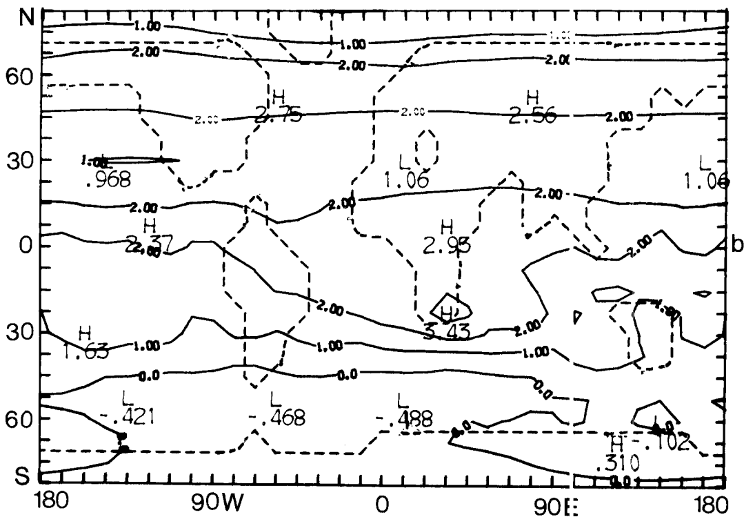
5.27 The temperature difference ( ^{\circ}\text{C} ) between the anomaly (Experiment 5) and control run for February. a) at 750 mb; b) at 250 mb.
