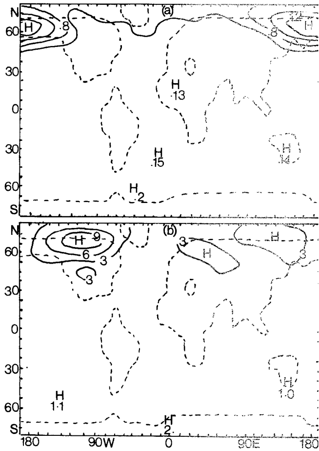
5.33 Geographical distribution of the standard deviations ( St ) ij from five Februaries (the normal February and four ij random perturbations of the normal) simulated by the model. a) 750 mb temperature (°C) b) 750 mb geopotential (m).
