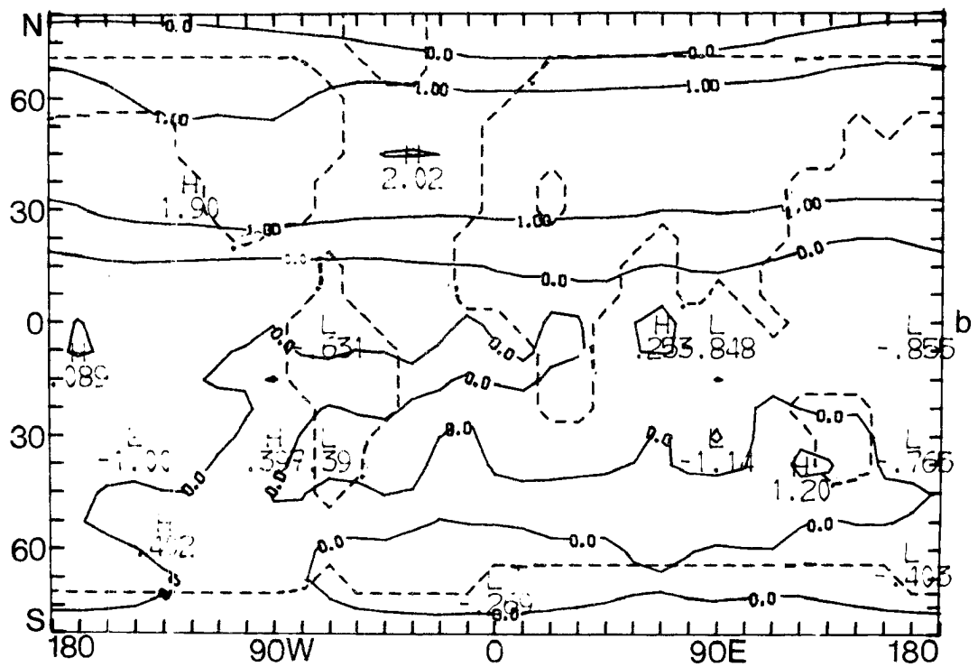
5.2 The temperature difference ( ^{\circ}\text{C} ) between the anomaly (Experiment 1) and control run for February. a) at 750 mb; b) at 250 mb.
