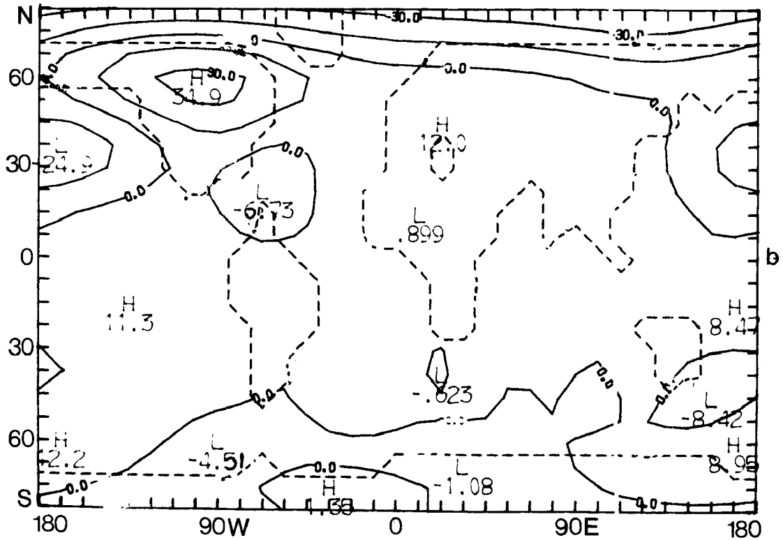
5.15 The geopotential height difference (m) between the anomaly (Experiment 3) and control run for February. a) at 750 mb; b) at 250 mb.
