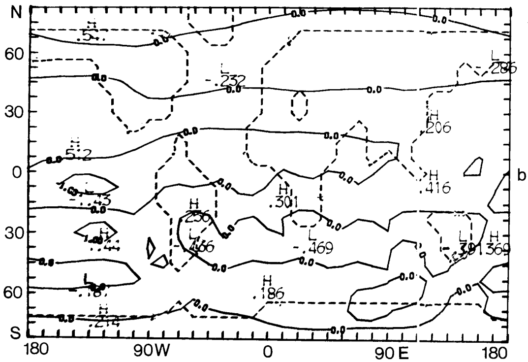
5.8 The temperature difference ( ^{\circ}\text{C} ) between the anomaly (Experiment 2) and control run for February. a) at 750 mb; b) at 250 mb.
