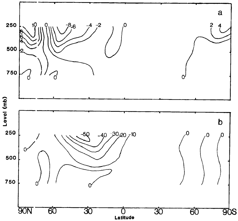
3.34 Vertical cross section of the simulated zonally averaged northward transport of geopotential height ( \text{m}^2 \text{sec}^{-1} ) for January. a) by the transient eddies; b) by the stationary eddies.
