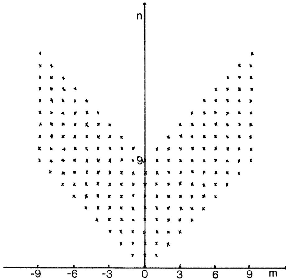
2.1 Schematic representation of the model's rhomboidal spectral resolution, m is the zonal wave number and n is the degree of the spherical harmonic.
