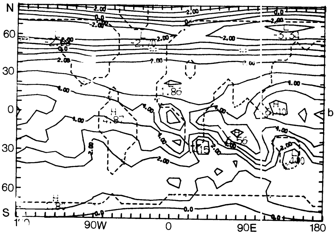
5.21 The temperature difference (°C) between the anomaly (Experiment 4) and control run for February. a) at 750 mb; b) at 250 mb.
