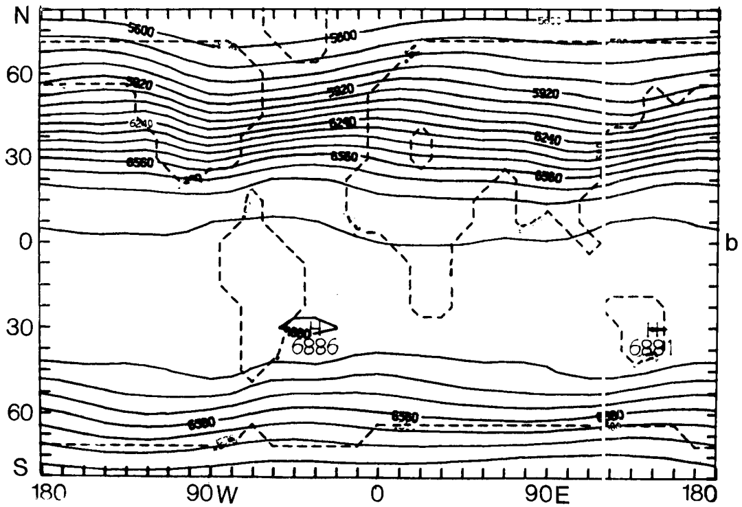
3.17 The geopotential height for January. a) observed ( 10^2\text{m} ) at 400 mb; b) simulated (m) at 500 mb.
