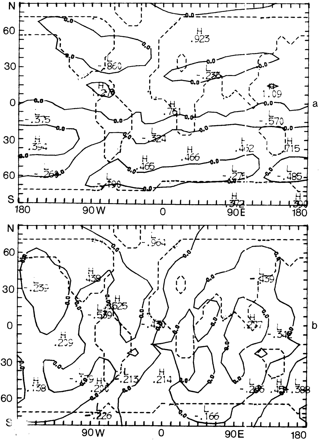
5.7 The horizontal wind difference ( \text{m sec}^{-1} ) at 500 mb between the anomaly (Experiment 2) and control run for January. a) zonal wind; b) meridional wind.
