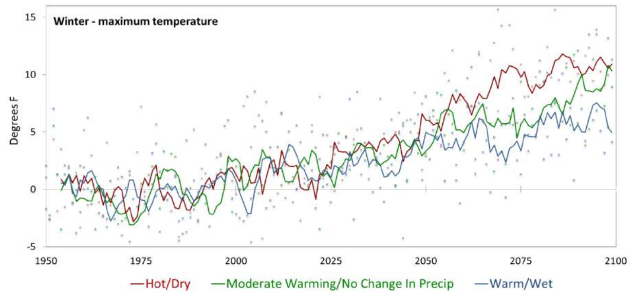
Difference in winter (Dec-Jan-Feb) temperatures compared to 1971-2000 normals.
