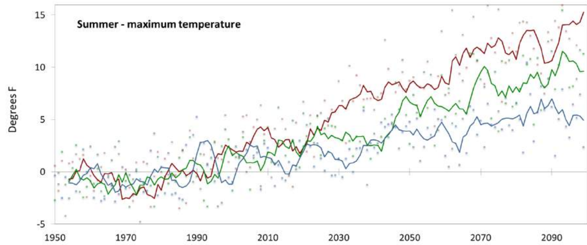
— Hot/Dry — Moderate Warming/No Change In Precip — Warm/Wet Difference in summer (Jun-Jul-Aug) temperatures compared to 1971-2000 normals.
