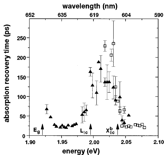
FIG. 1. (a) Variation of the absorption recovery time with excitation energy. \blacktriangle and \square identify the decays obtained by pumping with R6G and DCM, respectively. The arrows mark the energy position of the band gap E_g , and that of L_{1c} and X_{1c}^b with respect to E_g .
