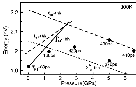
FIG. 3. Lifetime ( \tau_{PL} ) and associated peak energy of PL transitions in \text{In}_{0.48}\text{Ga}_{0.52}\text{P}/\text{In}_{0.5}\text{Al}_{0.5}\text{P} MQWs at high pressures. The straight lines show the pressure dependence of the PL transitions determined from cw PL measurements of Refs. 4 and 5.
