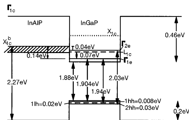
FIG. 2. Band structure of the 85 Å/225 Å \text{In}_{0.48}\text{Ga}_{0.52}\text{P}/\text{In}_{0.5}\text{Al}_{0.5}\text{P} MQWs, showing the separation of the electronic conduction states associated with \Gamma_{1c} , L_{1c} , and X_{1c}^b . The shaded region corresponds to the energy range for which long recovery times are measured.
