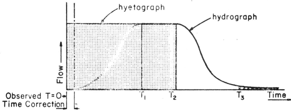
Fig. 3. Typical Equilibrium Hydrograph.
