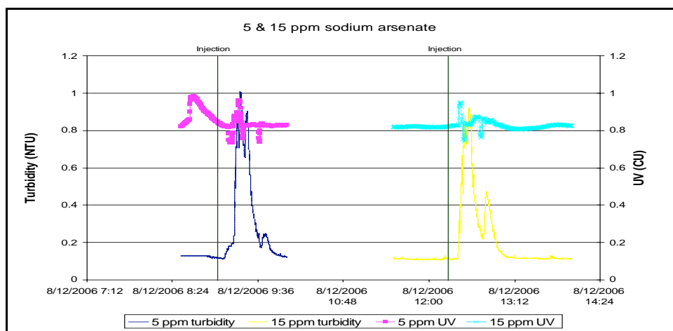
Figure 3-10 Turbidity and UV254 Absorption Response from Biofilm Exposure to Sodium Arsenate
