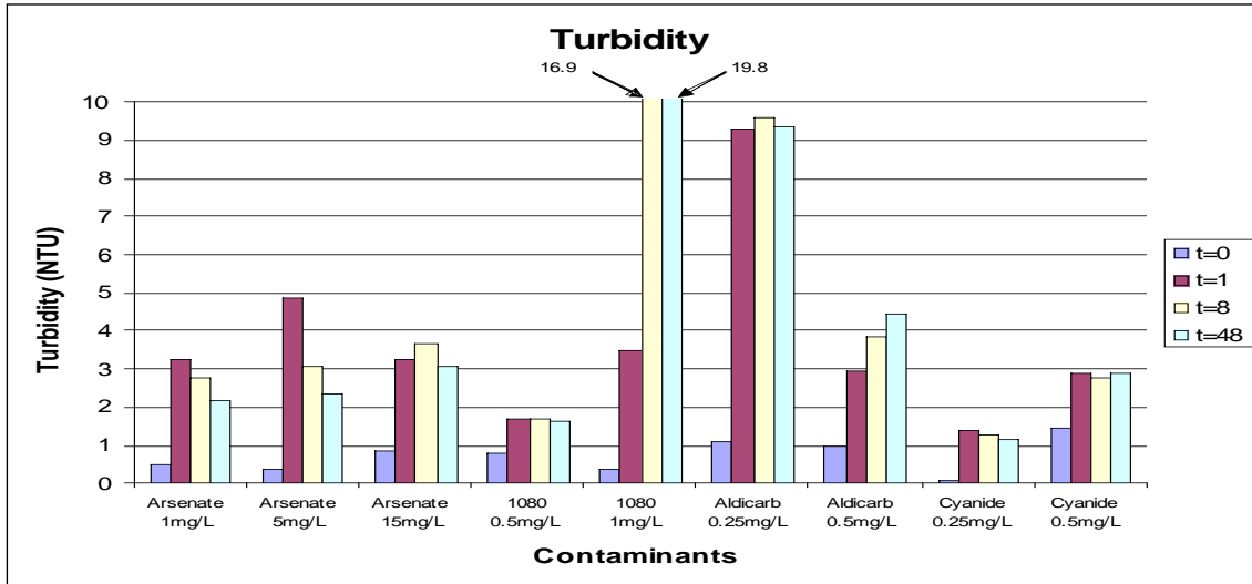
Figure 3-1 Turbidity Response from Biofilm Exposure to Contaminants – RAB
