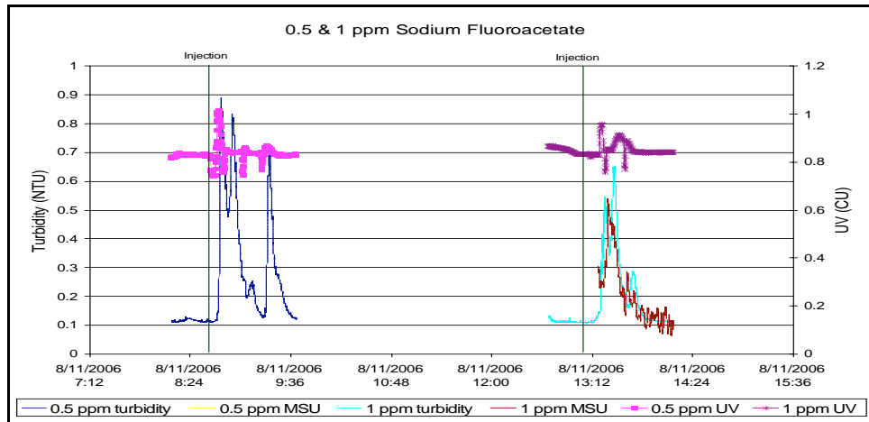
Figure 3-9 Turbidity and UV254 Absorption Response from Biofilm Exposure to Sodium Fluoroacetate
