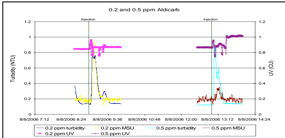
Figure 3-6 Turbidity and UV254 Absorption Response from Biofilm Exposure to Aldicarb
