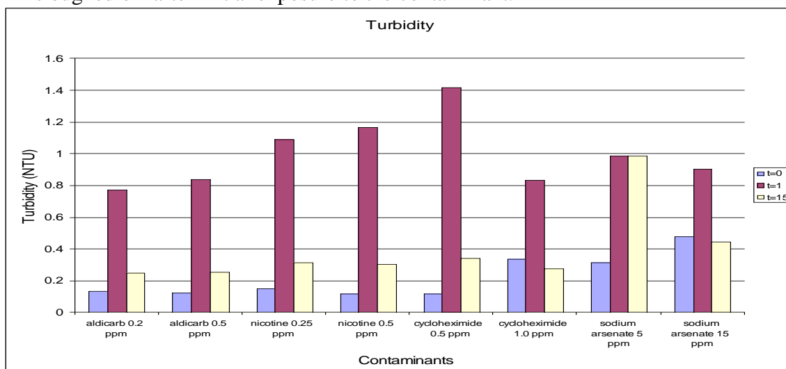
Figure 3-3 Turbidity Response (On-line Turbidimeter) from Biofilm Exposure to Contaminants
