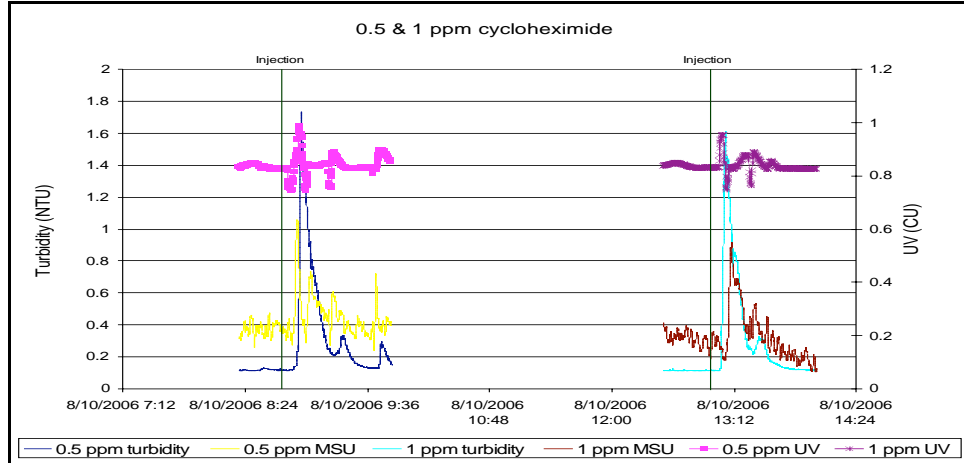
Figure 3-8 Turbidity and UV254 Absorption Response from Biofilm Exposure to Cycloheximide
