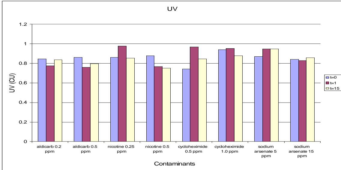
Figure 3-4 UV Response from Biofilm Exposure to Contaminants
