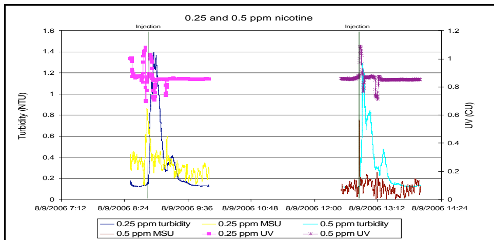
Figure 3-7 Turbidity and UV254 Absorption Response from Biofilm Exposure to Nicotine
