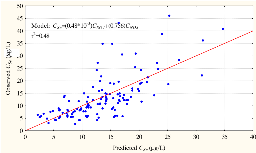
Figure 12. Observed Se concentrations in surface water compared to concentrations predicted by a multivariate relationship with SO 4 and NO 3 concentrations.
