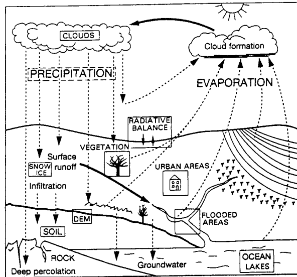
Figure 2. The hydrological cycle. (Based on WMO, 1994, altered by PORTMANN, 1997)
