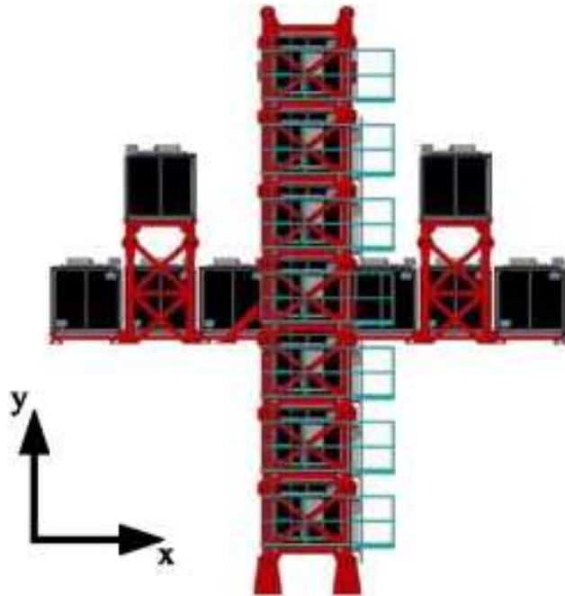
Figure 2.18: A schematic of the INGRID detector showing the arrangement of the tracking scintillating modules. There are 16 identical modules total with seven in the vertical row, seven in the horizontal row, and two at off-axis positions. With the vertical row upstream of the horizontal row, the designed beam center intersects each row's center module [28].
