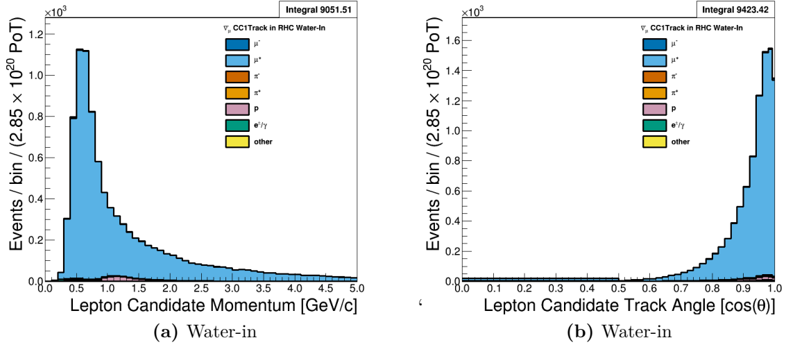
Figure 4.14: Reconstructed kinematics of the \bar{\nu}_\mu in RHC Mode CC 1-Track selection categorized by the true particle matched to the main track. The figures use the PØD water-in MC and are normalized to the RHC water-in mode POT. Also a single bin is used in the range of 0 \leq \cos \theta < 0.5 in figure (b).
