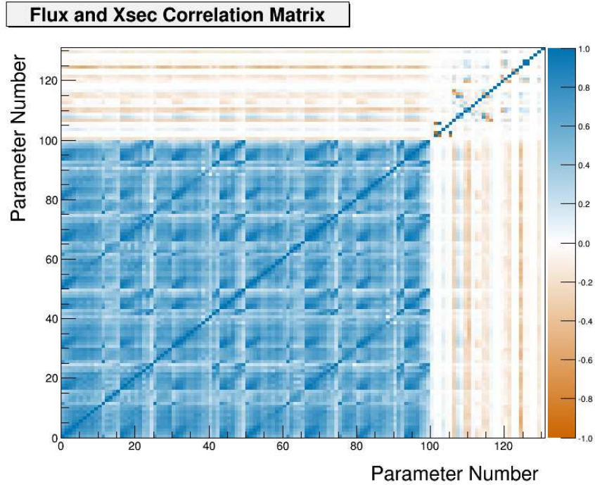
Figure 6.8: Flux and cross section postfit correlation matrix for the Asimov data fit. The parameters from 1-100 are the flux parameters and all parameters after are the cross section.
