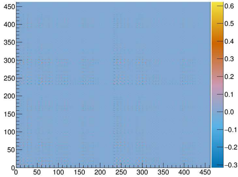
Updated Covariance
