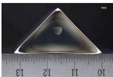
Figure 2.25: A cross section of a PØD scintillating bar. The base and height is 33 mm long and 17 mm high. The wavelength shifting fiber is inserted in the bored hole which is half-way between the base and tip.
