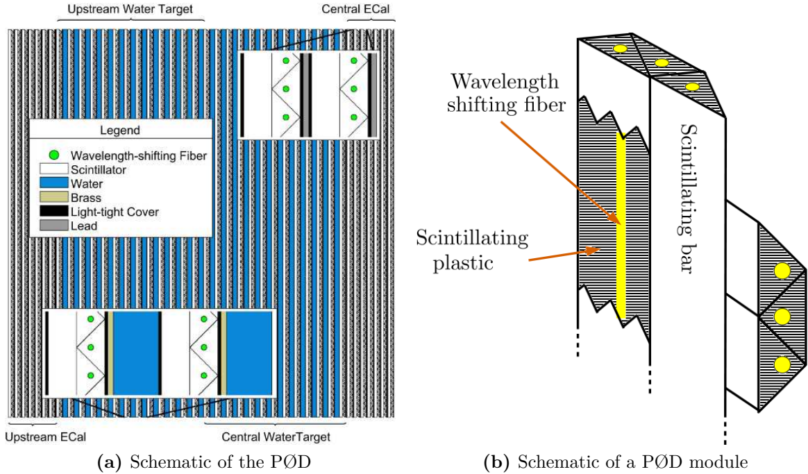
Figure 2.24: Schematics of the PØD. Left: insets detail the Water Target and ECal layers. Right: A view of a PØD module illustrating the orthogonal layout of the scintillating planes. Both: the neutrino beam is coming from the left.
