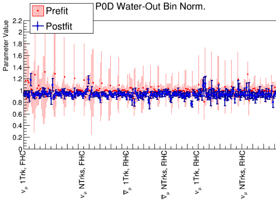
(b) Water-Out
