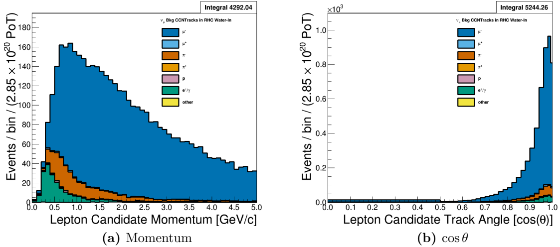
Figure 4.26: Reconstructed kinematics of the \nu_\mu Background in RHC Mode CC 1-Track selection categorized by the true particle matched to the main track. The figures use the PØD water-in MC and are normalized to the RHC water-in mode POT. Also a single bin is used in the range of 0 \leq \cos \theta < 0.5 in figure (b).
