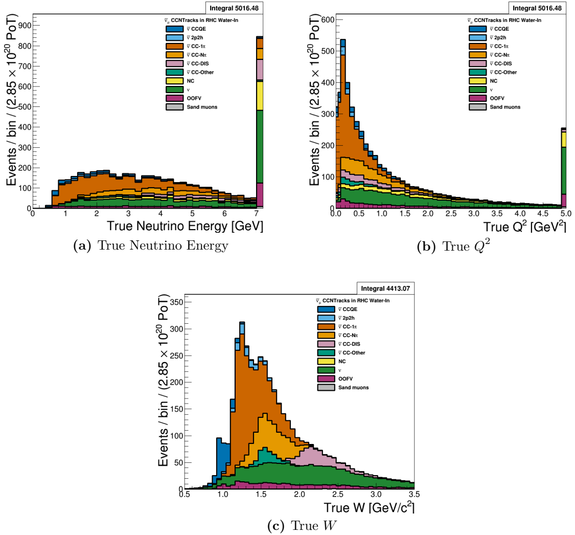
Figure 4.20: True kinematics of the \bar{\nu}_\mu in RHC Mode CC N-Tracks selection. The last bin shown in (a) and (b) is used as overflow. The figures use the PØD water-in MC and are normalized to the RHC water-in mode POT.
