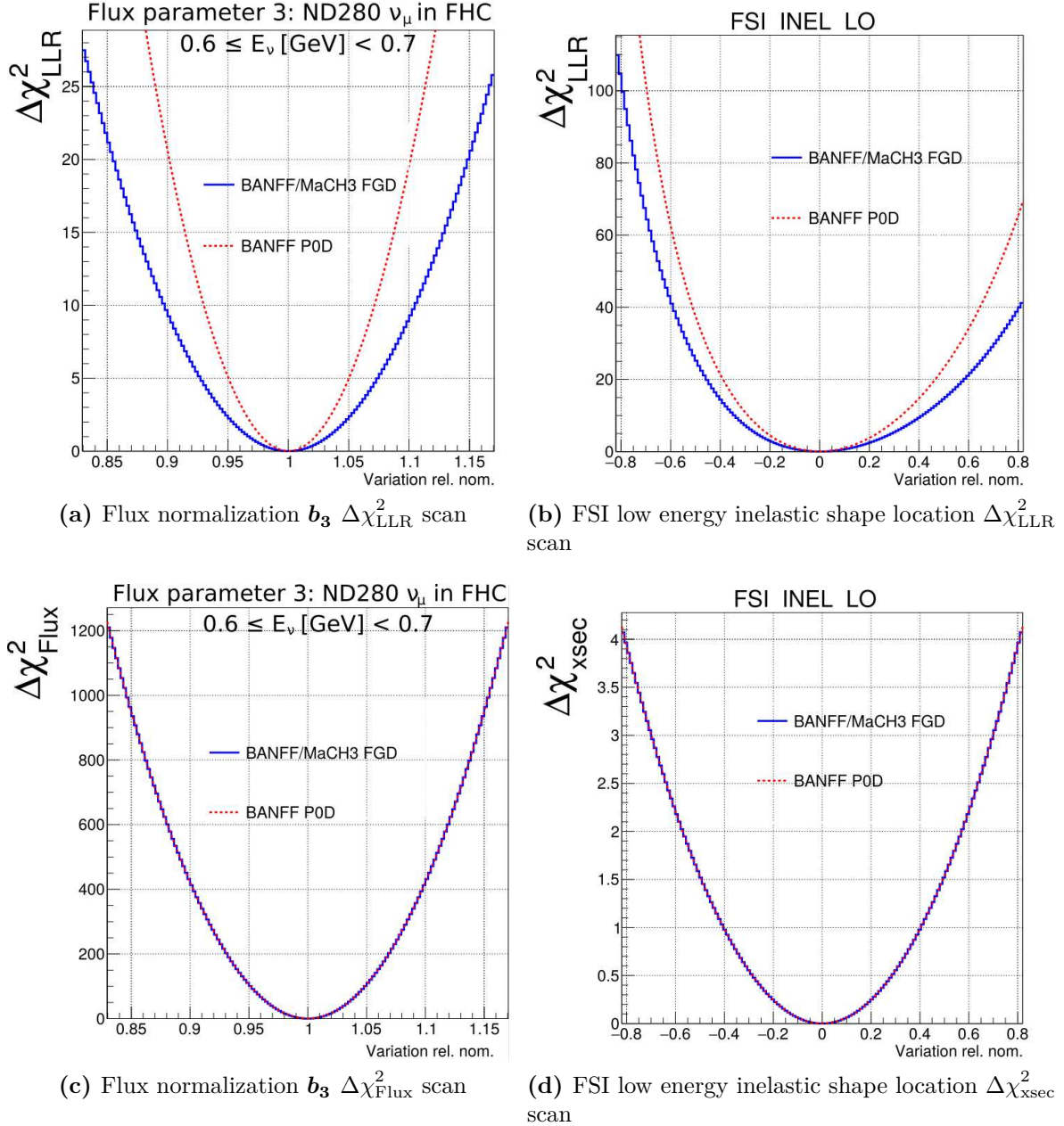
Figure 6.2: Comparison of \Delta\chi^2 scans for variations in fit parameters in the Asimov set. Two parameters are varied: parameter 3 (left) corresponding to a flux bin normalization and 562 (right) corresponding to a FSI shape location parameter. The top panel shows the change in the LLR test statistic \Delta\chi_{\text{LLR}}^2 while the bottom panel shows the penalty terms. In all sub-figures are comparisons between the BANFF/MaCH3 FGD 2017 results [31] against the BANFF P0D-only results. Special thanks goes to Clarence Wret (c.wret@rochester.edu) of the University of Rochester for generating the plots.
