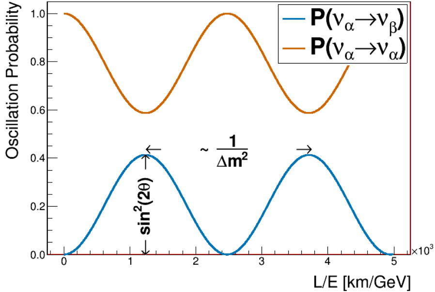
Figure 2.7: Two flavor oscillation probability as a function L/E is shown using \theta = 20^\circ and \Delta m^2 = 10^{-3} \text{ eV}^2/c^4 . The spacing between adjacent peaks/troughs is proportional to the inverse of \Delta m^2 . Note that \mathcal{P}(\nu_\alpha \rightarrow \nu_\alpha) = 1 - \mathcal{P}(\nu_\alpha \rightarrow \nu_\beta) since the oscillation probability must always sum to 1.
