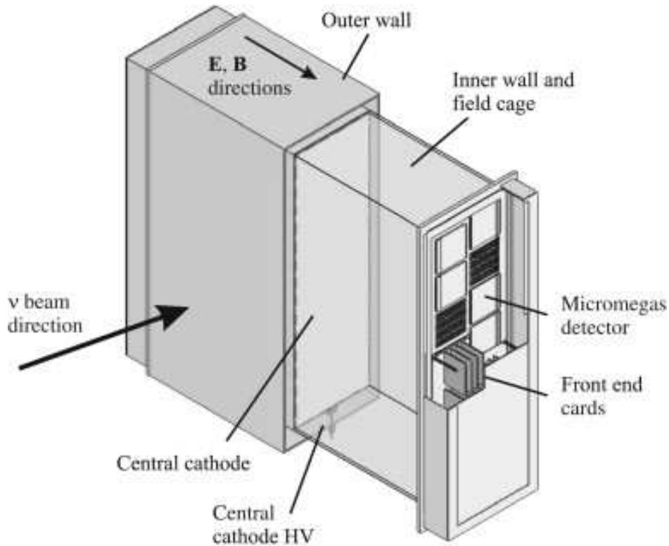
Figure 2.26: Cut-away drawing of a TPC volume in ND280 [19].
