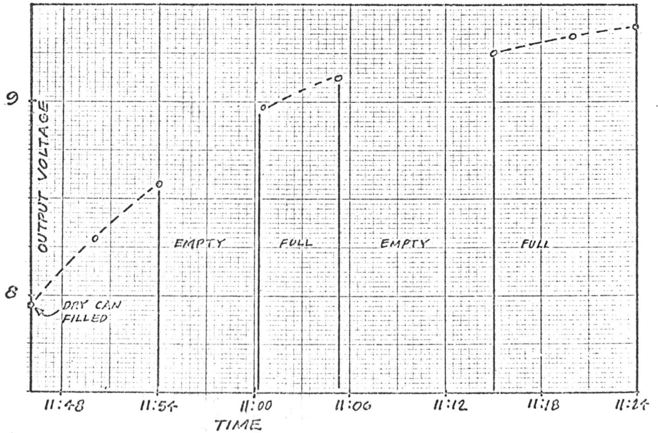
Figure 21 Typical Drift of Enameled Wire Probes
