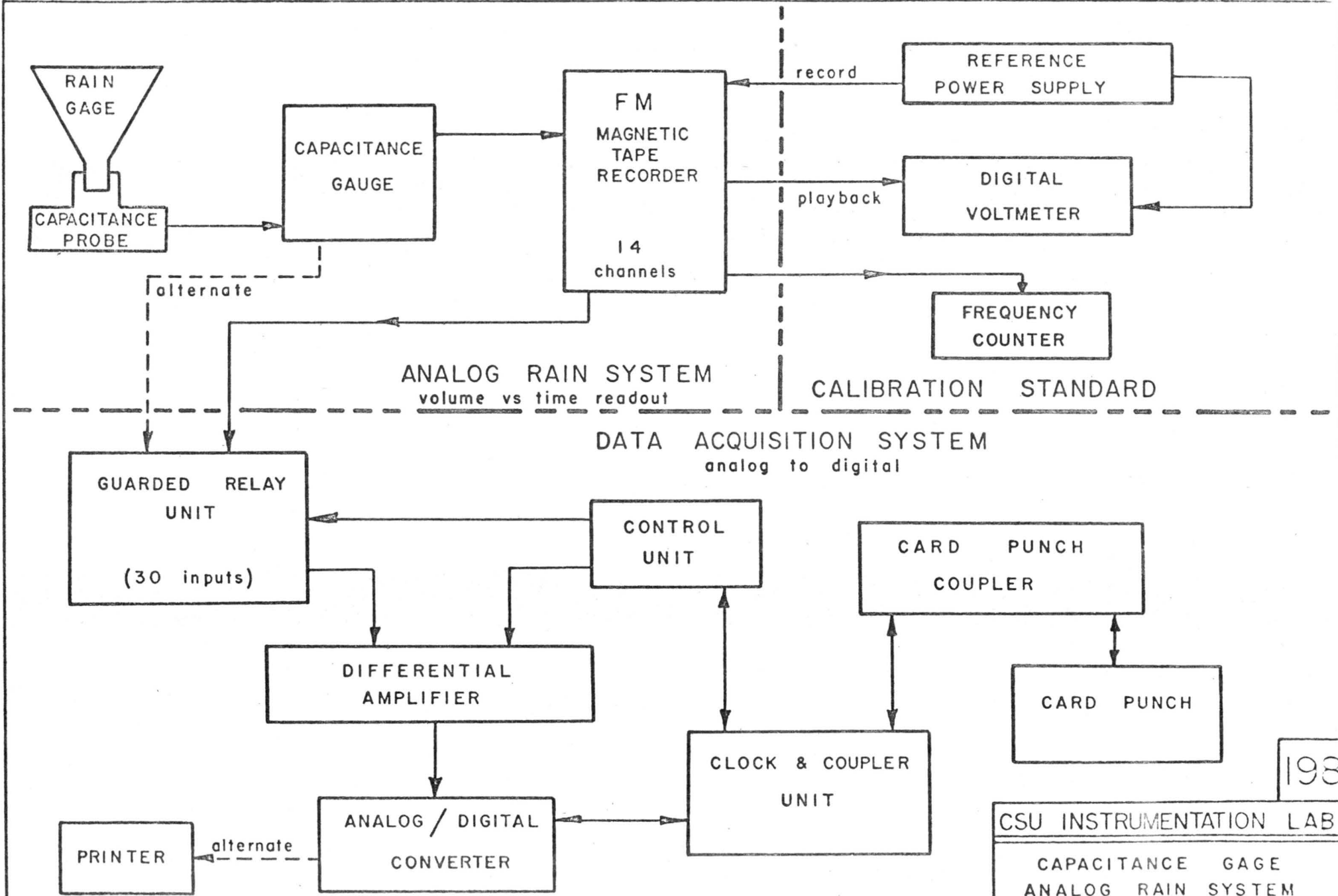
Figure 18 Capacitance Rainage Block Diagram
