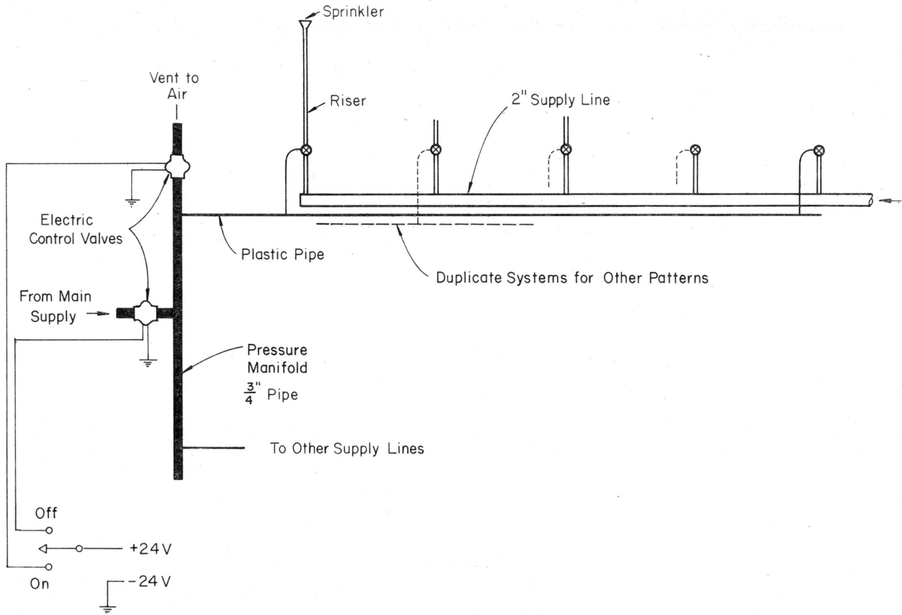
Figure 16 Schematic of Hydraulic Control System for Sprinklers
