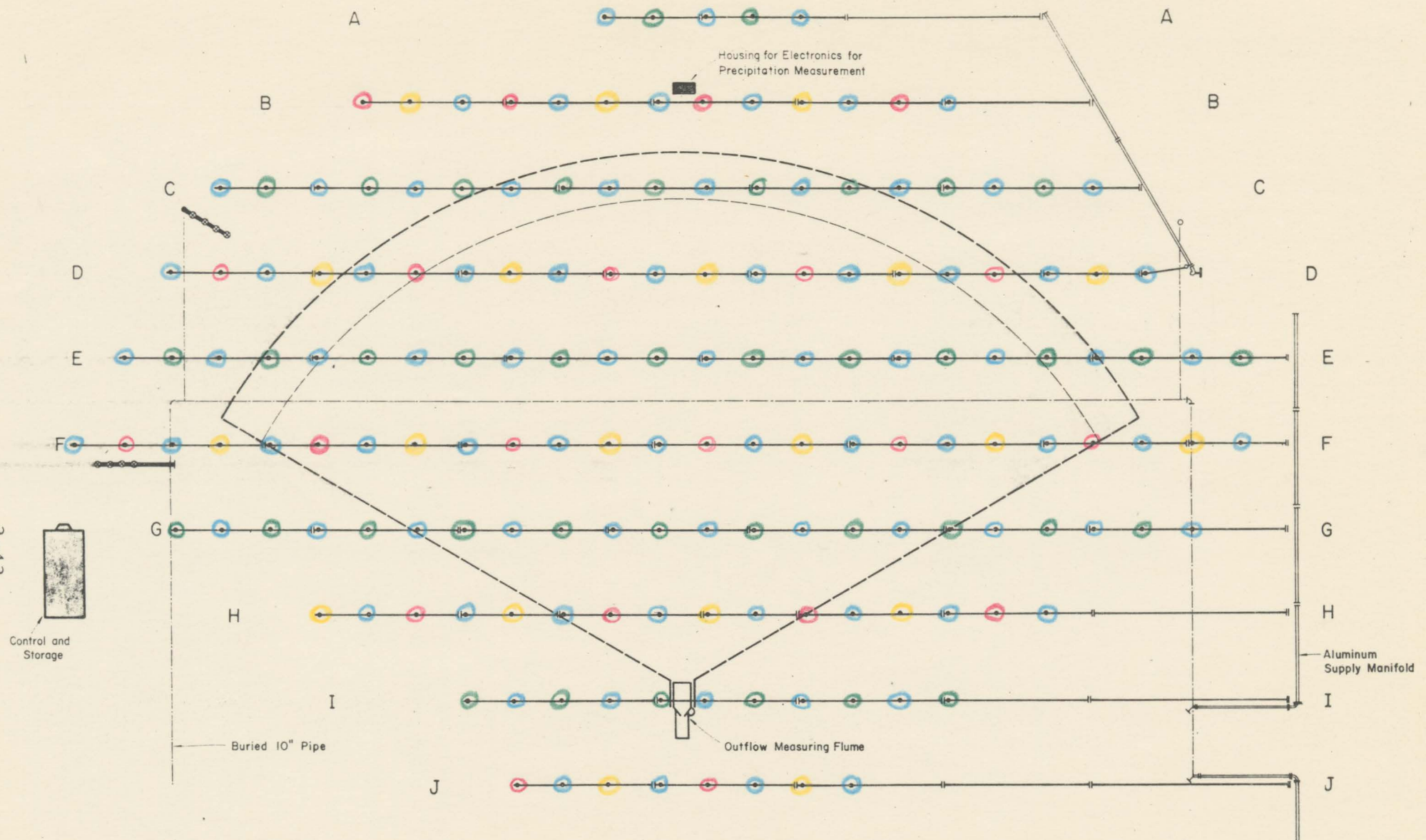
Figure 17 RAINFALL-RUNOFF EXPERIMENTAL FACILITY
