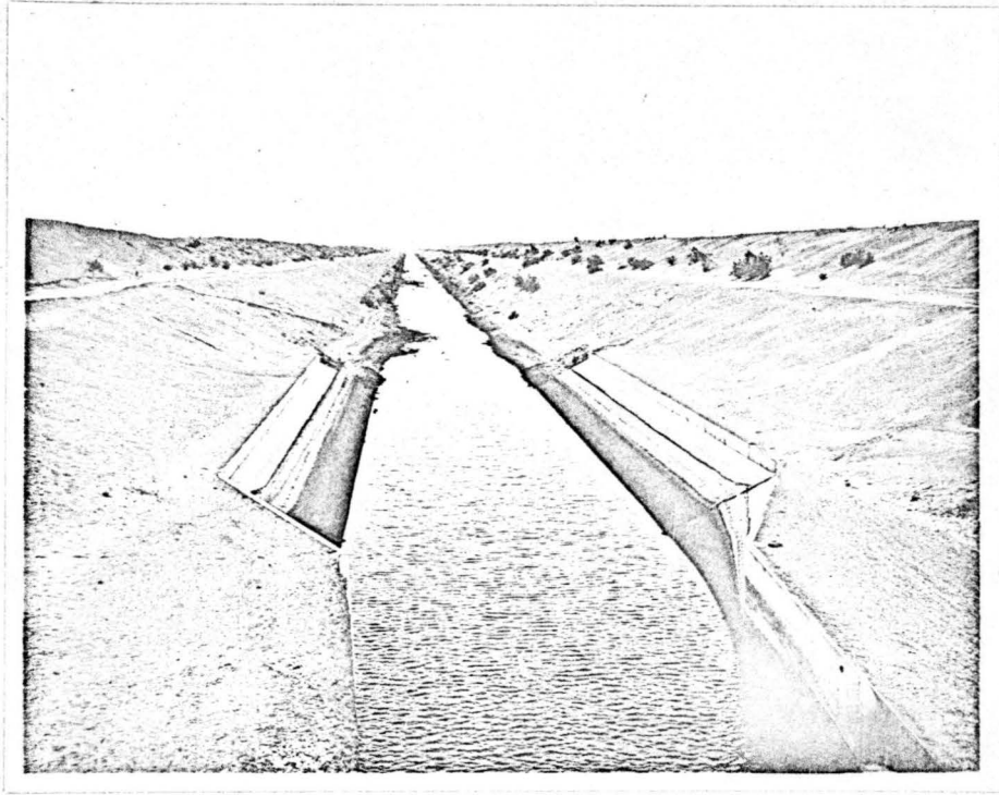
Fig. 2 View downstream from drop at Sta. 228+15
