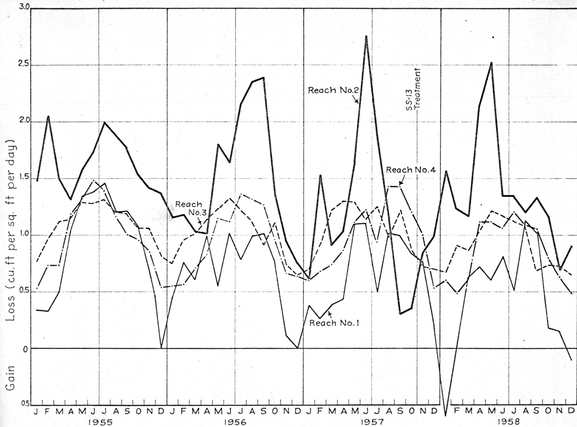
Fig. 16 Superimposed plot of losses by reaches
