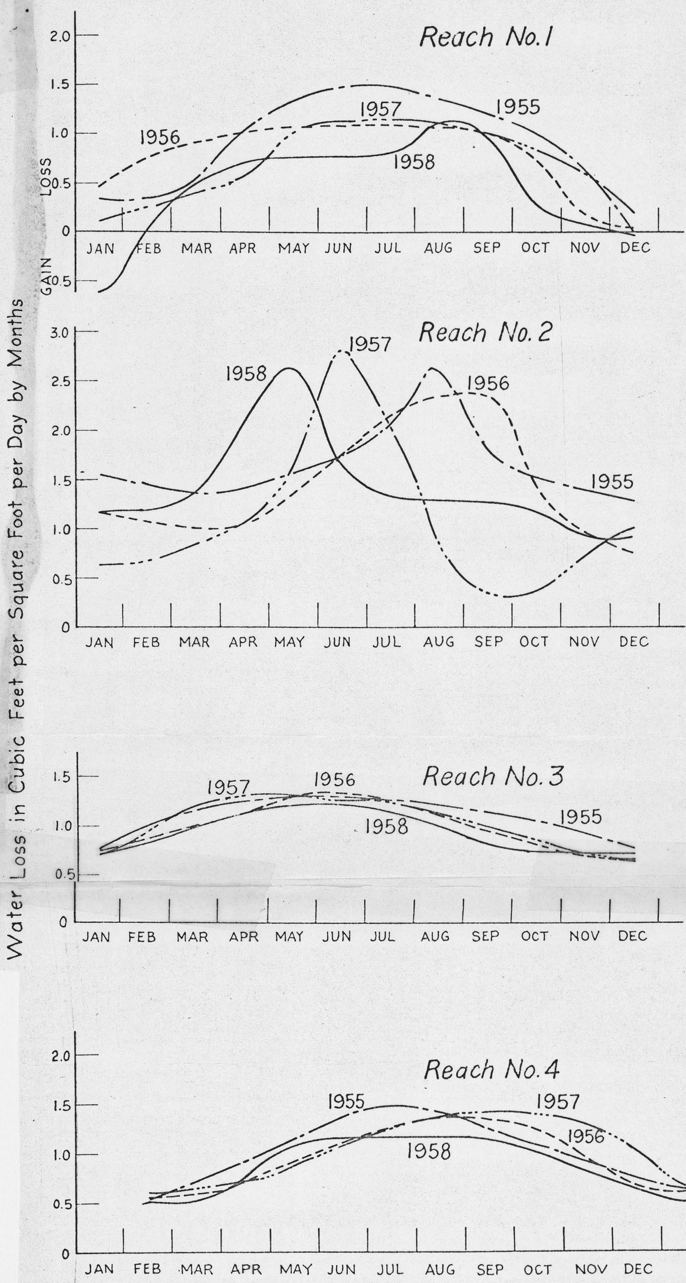
Fig. 17 Separated plots of losses by reaches
