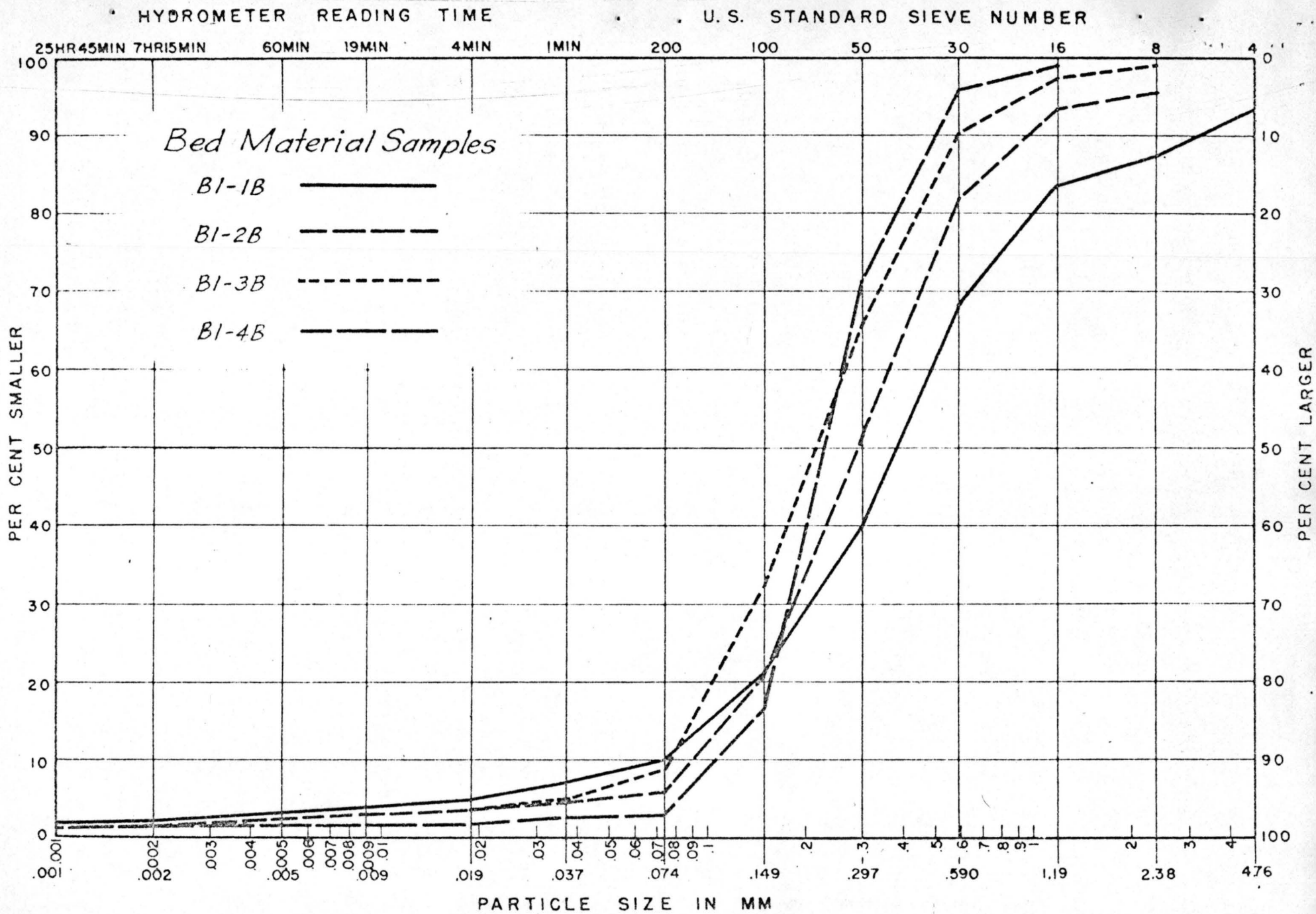
Fig. 4 Size distribution curves for bed material samples
