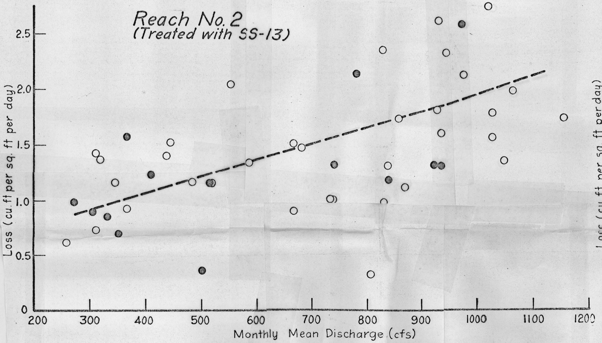
Fig. 18 Plot of monthly loss by reaches
