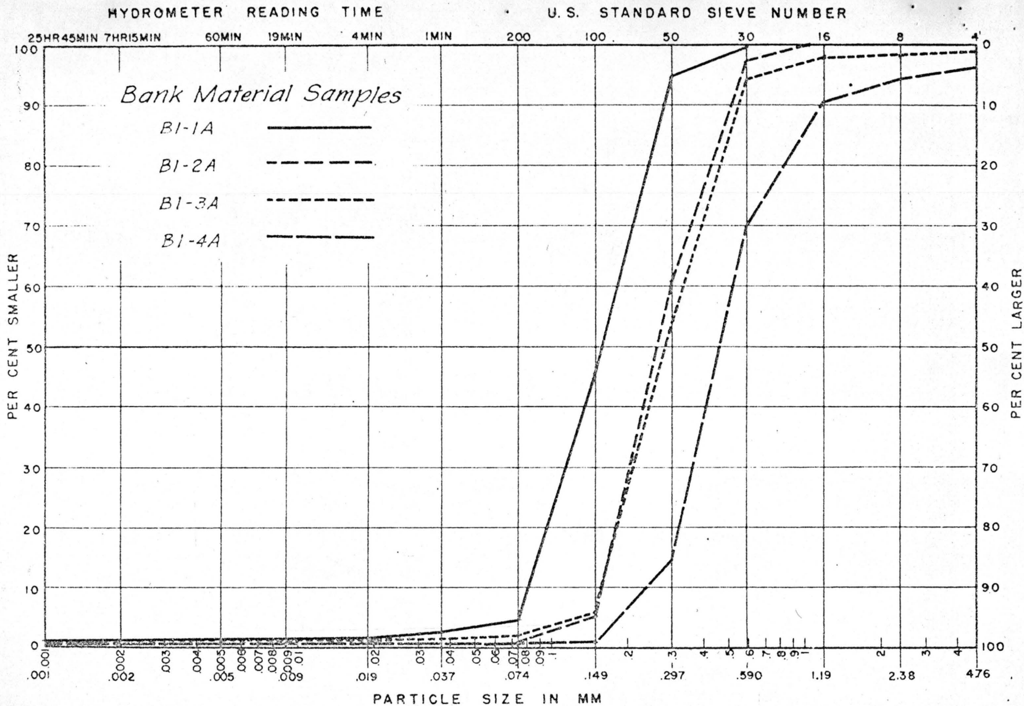
Fig.5 Size distribution curves for bank material samples
