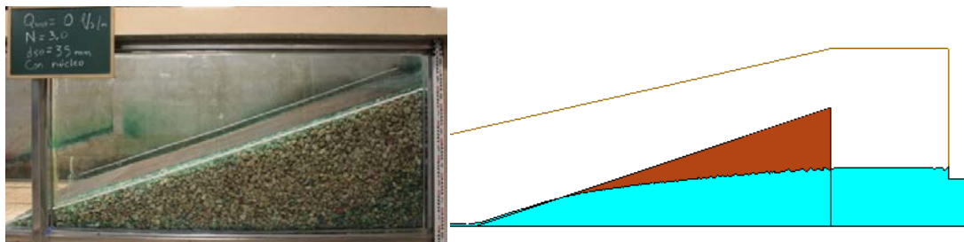
Figure 3. Example of physical and numerical models used by San Mauro et al. (2015) for the experimental assessment of a and b .
