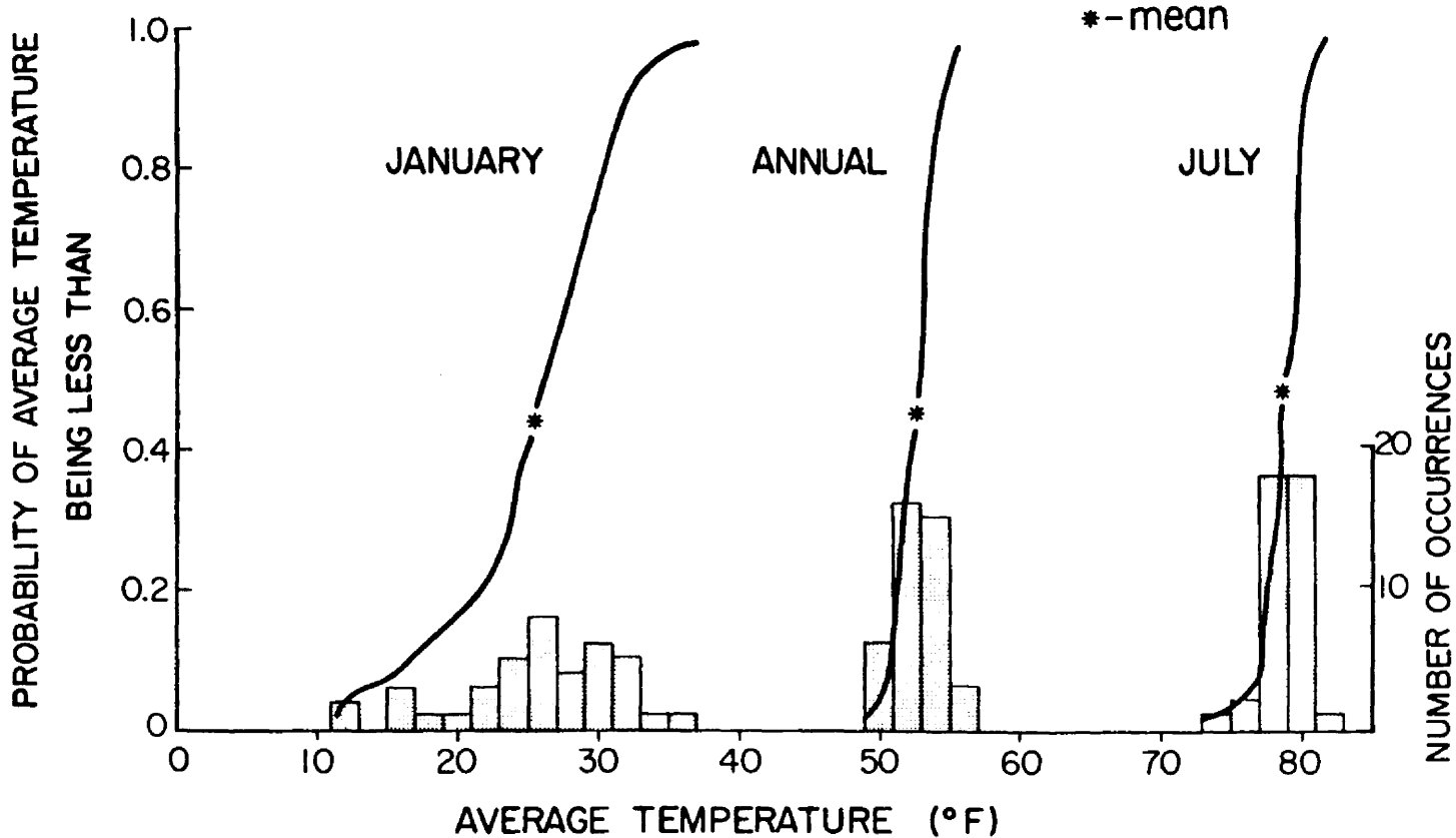
Figure 5. Distribution of January, July, and annual average temperatures for Grand Junction, Colorado, 1940-1979. Number of occurrences of monthly and annual average temperatures within specified 2-degree Fahrenheit intervals are shown in histogram form. The same information is then shown in terms of probability distributions (Cumulative Distribution Functions).
