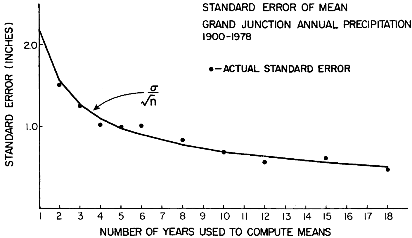
Figure 6. Comparison of actual standard error (dot's on graph) and theoretical standard error (solid line) as a function of record length. Annual precipitation data from Grand Junction, Colorado, 1900-1978, is used for this example.
