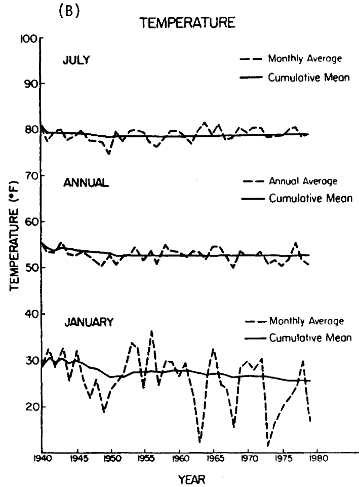
Figure 4. Time series of January, July, and annual precipitation (A) and average temperatures (B) for Grand Junction, Colorado, 1940-1979. Solid line is the cumulative mean for each time series.
