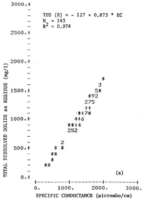
Figure A-2. Total dissolved solids - specific conductance data used in regression analysis, St. Vrain Creek near Platteville.
