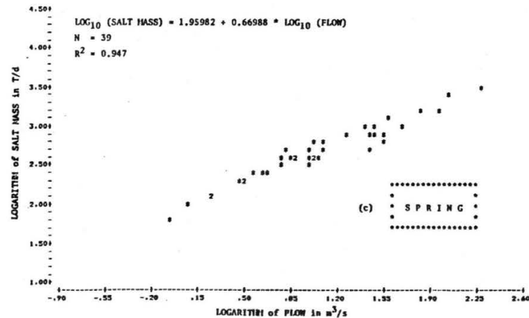
Figure B-1. Salinity mass - flow data used in regression analysis, South Platte River at Henderson.
