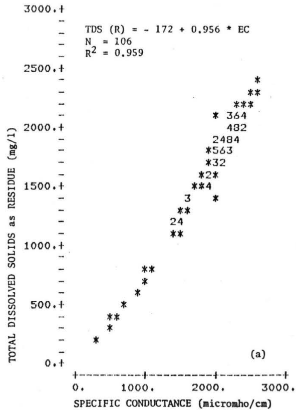
Figure A-3. Total dissolved solids - specific conductance data used in regression analysis, Big Thompson River near La Salle.
