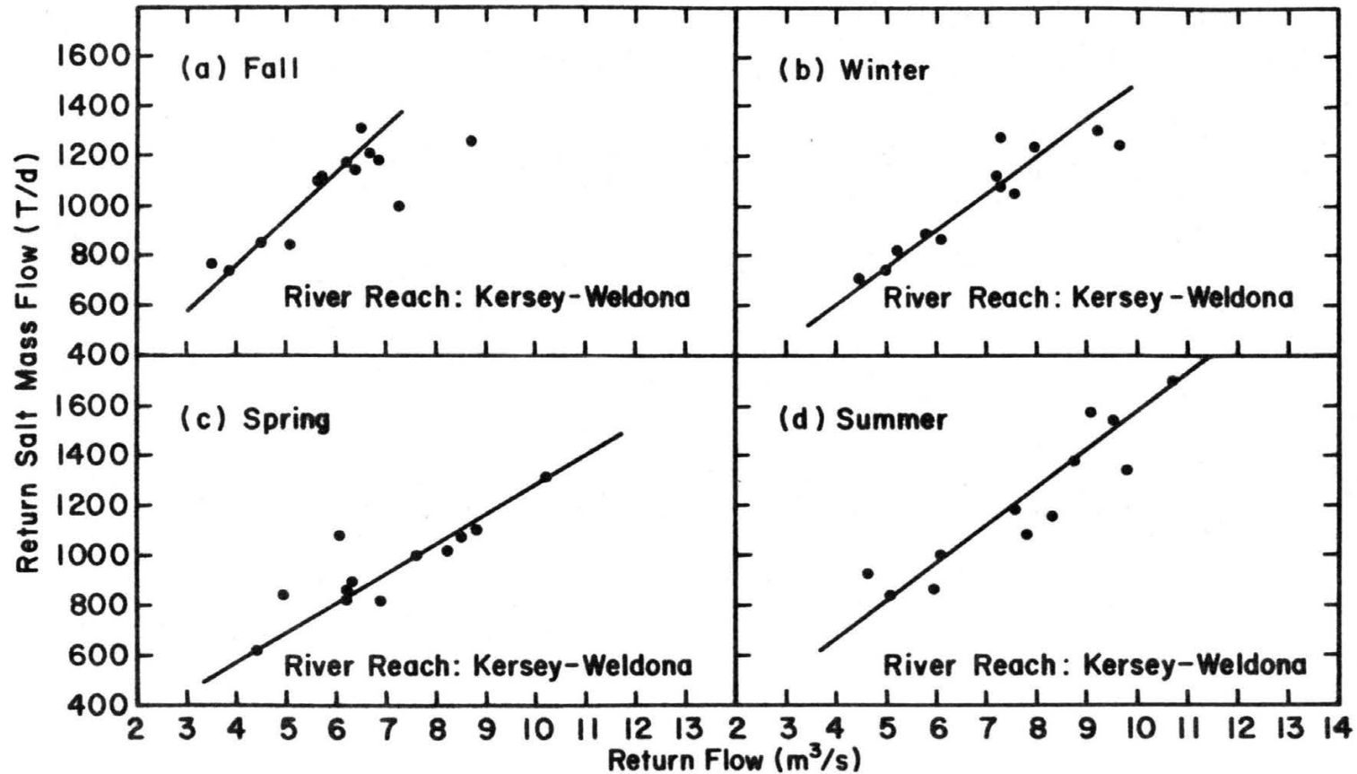
Figure 4-19. Computed return salt mass flow averaged by season associated with computed return flows, South Platte River between Kersey and Weldona, water years 1965-77 (based on modified data contained in Table F-4).
