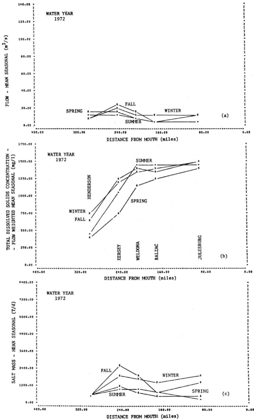
Figure D-8. Distance profiles of flow, salt concentration and salt mass flow averaged by season, South Platte River, water year 1972.
