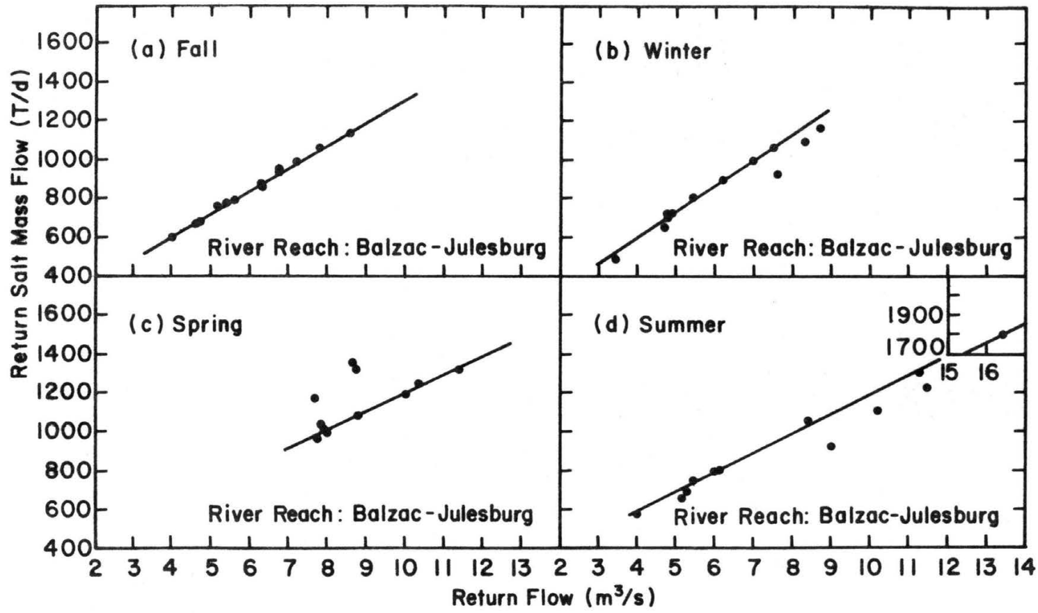
Figure 4-21. Computed return salt mass flows averaged by season associated with computed return flows, South Platte River between Balzac and Julesburg, water years 1965-77.
