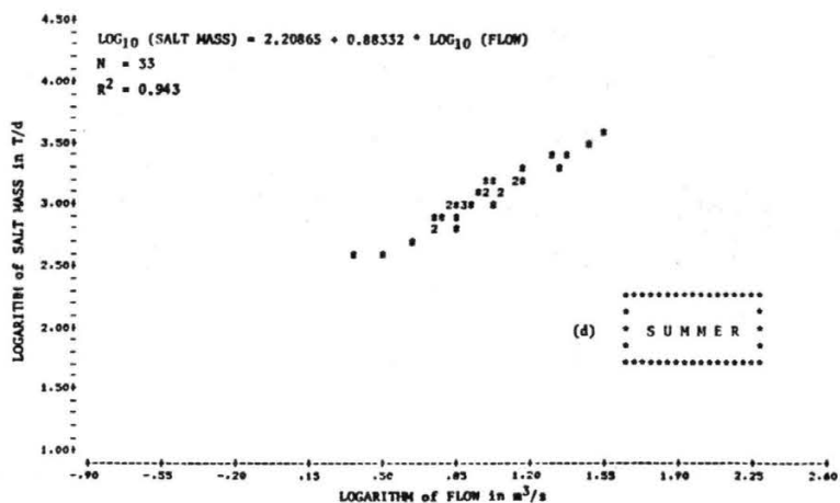
Figure B-6. Salinity mass - flow data used in regression analysis, South Platte River near Weldona.
