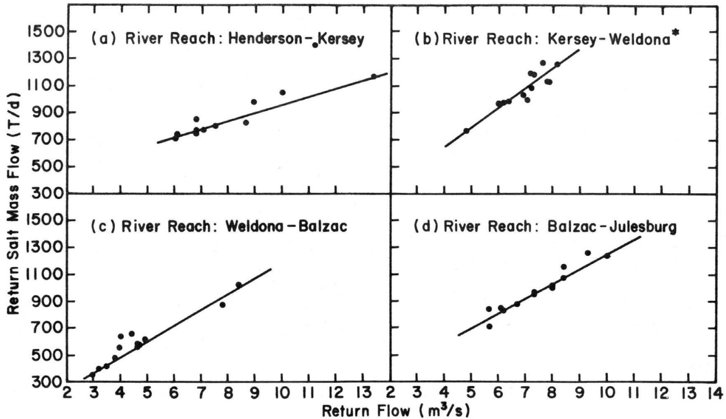
Figure 4-17. Computed return salt mass flow averaged by year associated with computed return flows in four river reaches, South Platte River between Henderson and Julesburg, water years 1965-77 (*based on modified data included in Table F-4).
