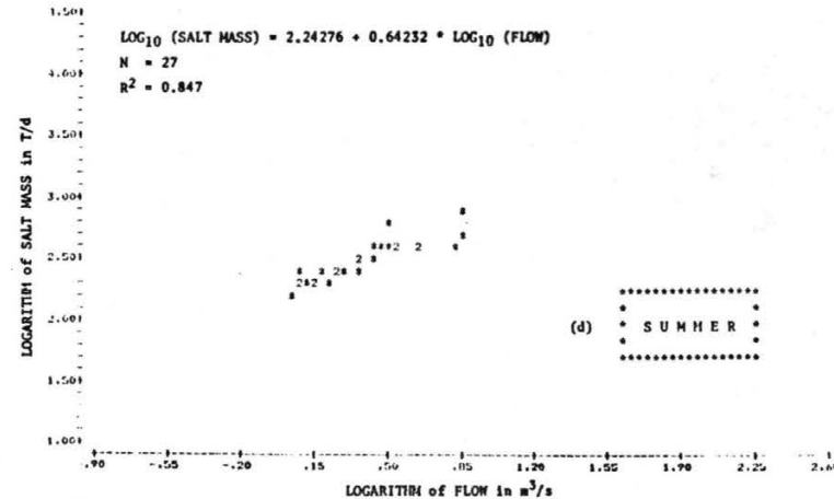
Figure B-3. Salinity mass - flow data used in regression analysis, Big Thompson River near La Salle.
