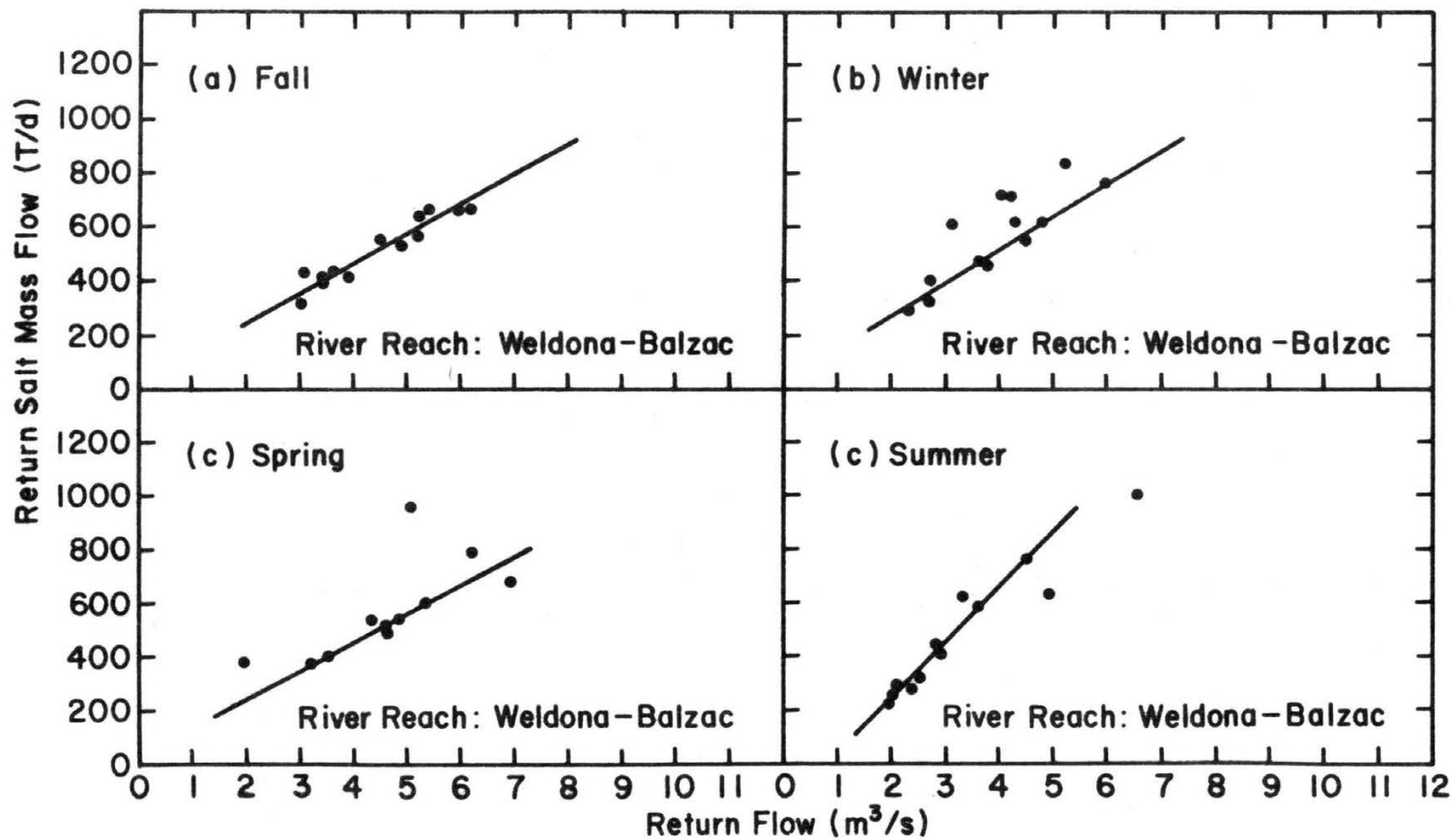
Figure 4-20. Computed return salt mass flows averaged by season associated with computed return flows, South Platte River between Weldona and Balzac, water years 1965-77.
