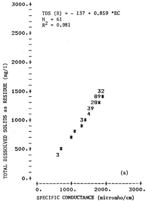
Figure A-5. Total dissolved solids - specific conductance data used in regression analysis, South Platte River near Kersey.
