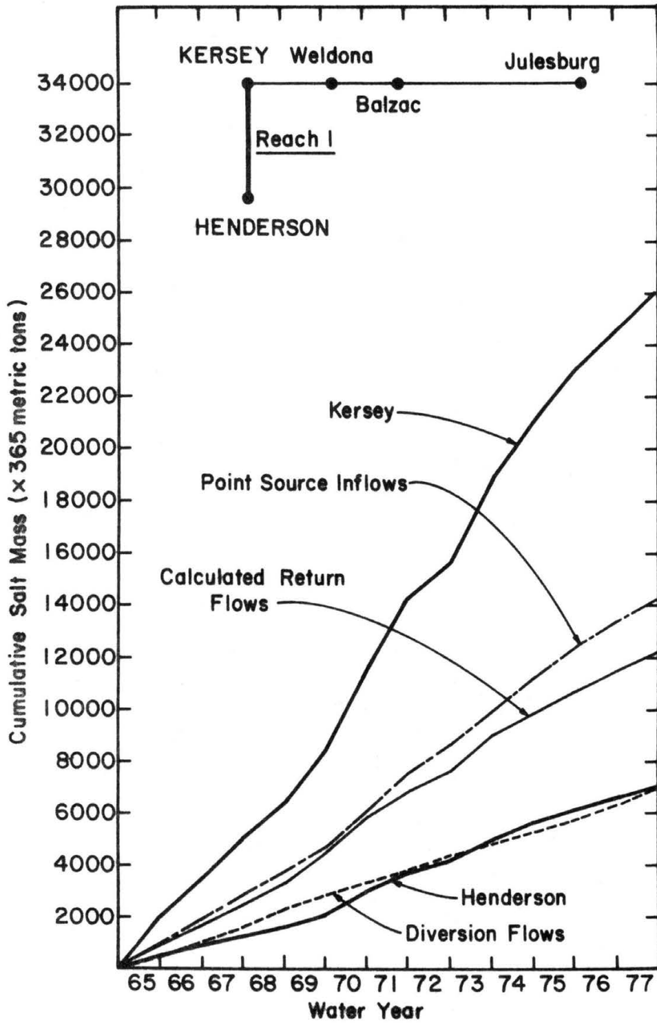
Figure 4-10. Cumulative salt mass to and from Henderson-Kersey reach, South Platte River, water years 1965-77.
