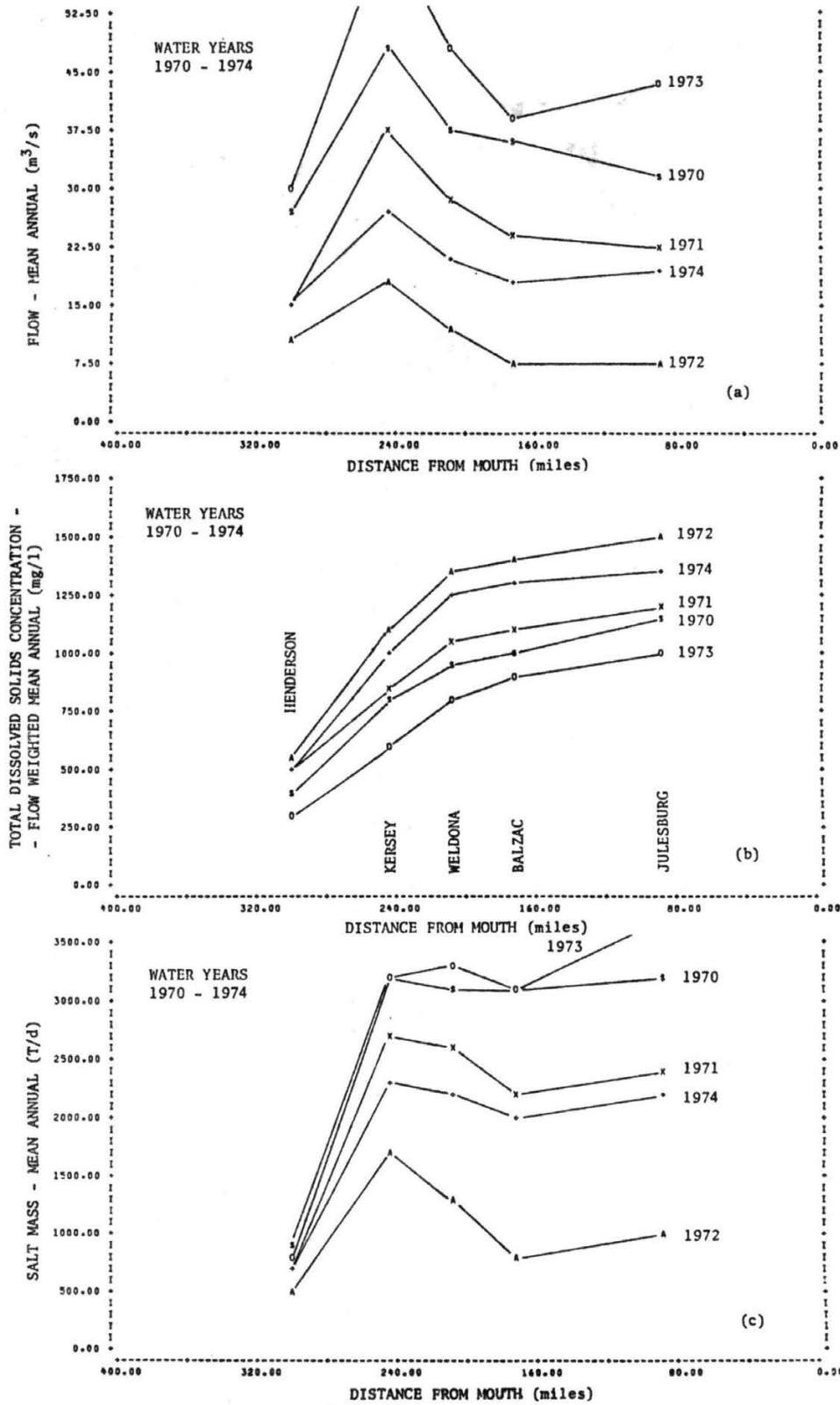
Figure 4-5. Distance profiles of flow, salt concentration, and salt mass flow, averaged by year, 1970-74, South Platte River.
