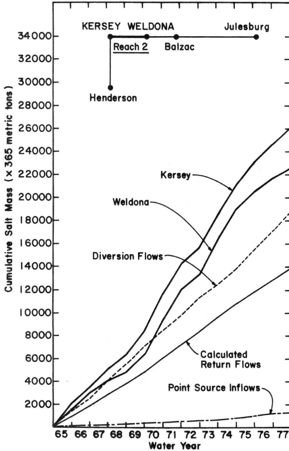
Figure 4-12. Cumulative salt mass to and from Kersey-Weldona reach, South Platte River, water years 1965-77.
