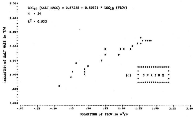
Figure B-9. Salinity mass - flow data used in regression analysis, Cache La Poudre River at mouth of canyon.
