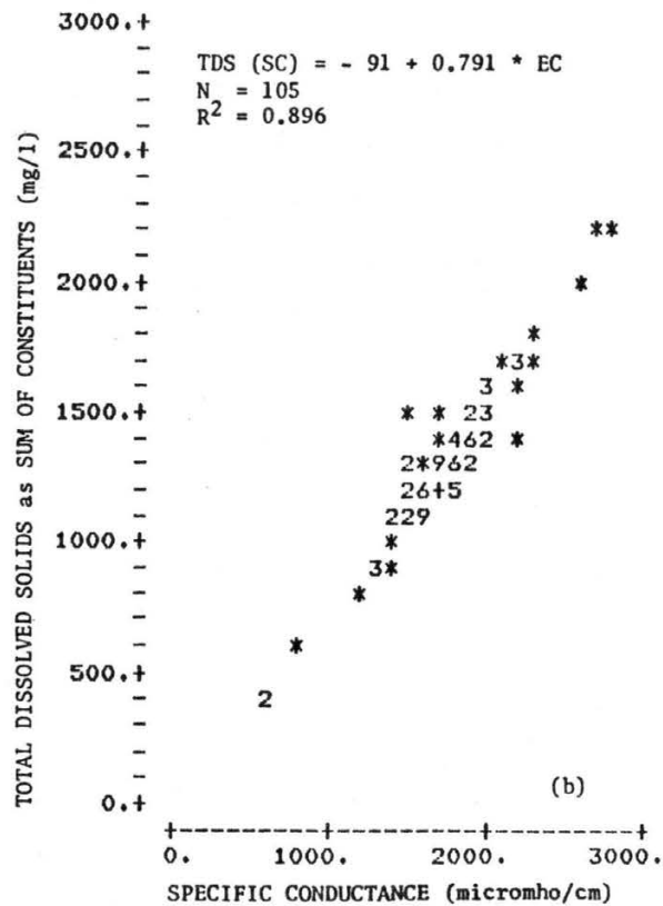
Figure A-6. Total dissolved solids - specific conductance data used in regression analysis, South Platte River near Weldona.
