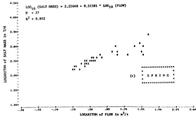
Figure B-2. Salinity mass - flow data used in regression analysis, St. Vrain Creek near Platteville.
