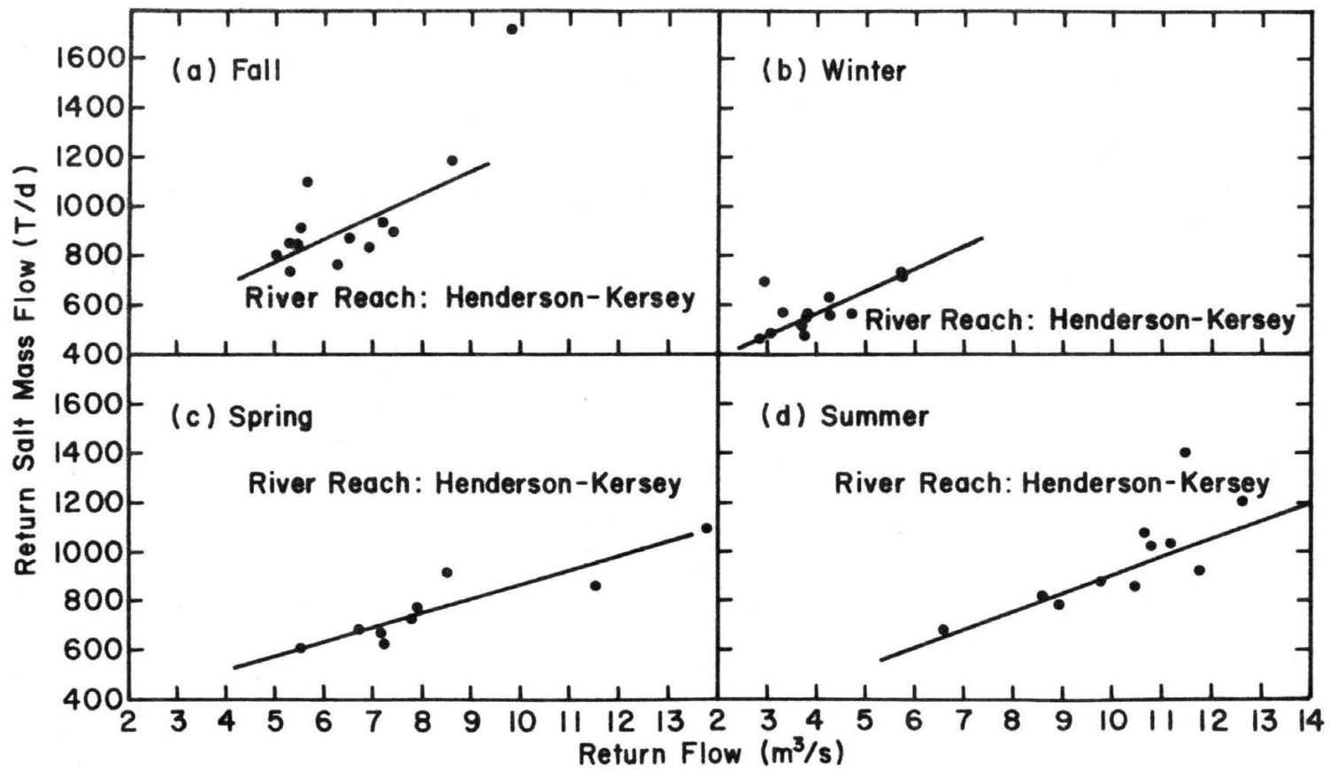
Figure 4-18. Computed return salt mass flows averaged by season associated with computed return flows, South Platte River between Henderson and Kersey, water years 1965-77.
