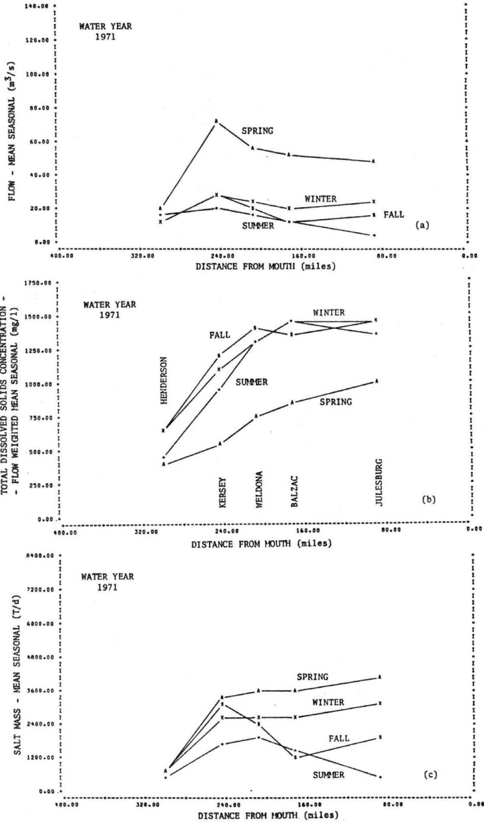
Figure D-7. Distance profiles of flow, salt concentration and salt mass flow averaged by season, South Platte River, water year 1971.
