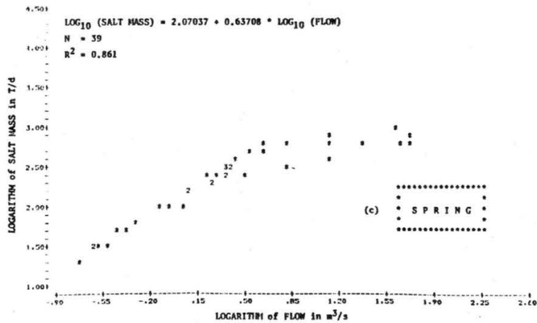
Figure B-4. Salinity mass - flow data used in regression analysis, Cache La Poudre River near Greeley.
