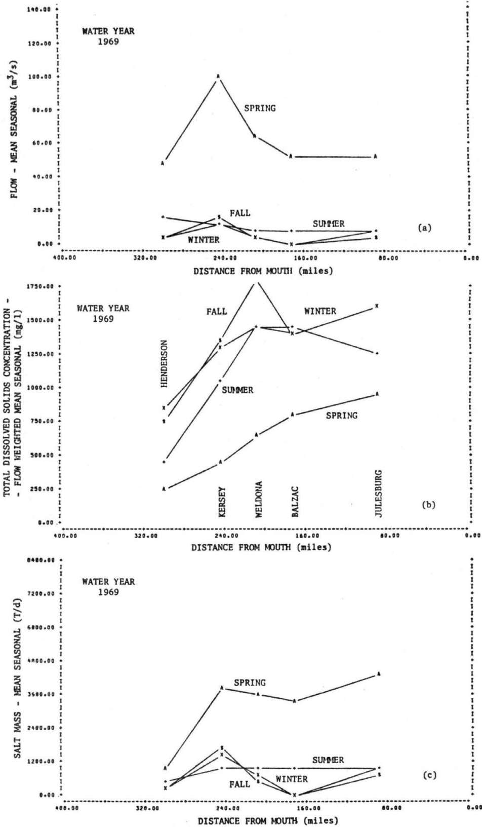
Figure D-5. Distance profiles of flow, salt concentration and salt mass flow averaged by season, South Platte River, water year 1969.
