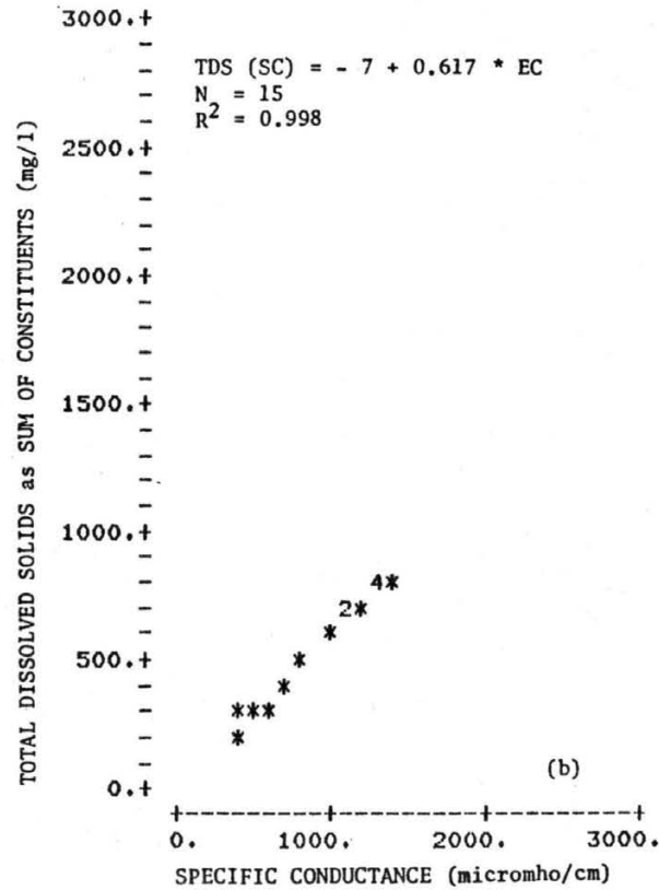
Figure A-1. Total dissolved solids - specific conductance data used in regression analysis, South Platte River at Henderson.
