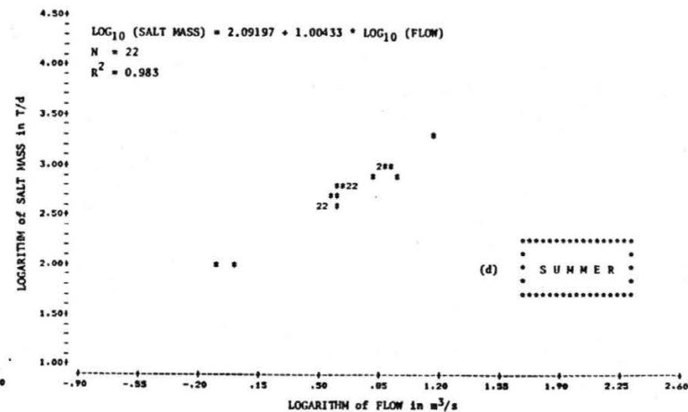
Figure B-7. Salinity mass - flow data used in regression analysis, South Platte River at Balzac.
