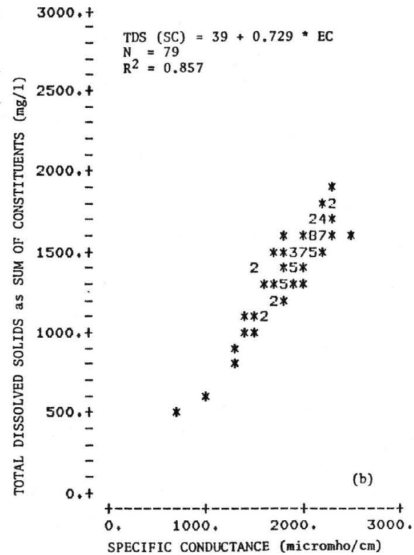
Figure A-8. Total dissolved solids - specific conductance data used in regression analysis, South Platte River at Julesburg.
