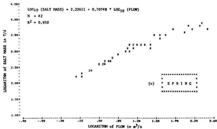
Figure B-5. Salinity mass - flow data used in regression analysis, South Platte River near Kersey.
