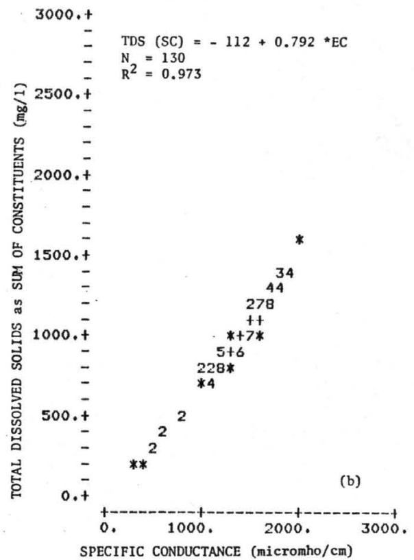
Figure A-2. Total dissolved solids - specific conductance data used in regression analysis, St. Vrain Creek near Platteville.
