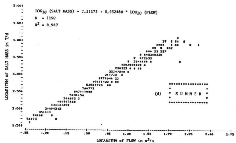
Figure 4-1. Salinity mass-flow, daily data used in regression analysis, water years 1965-79, South Platte River at Julesburg.
