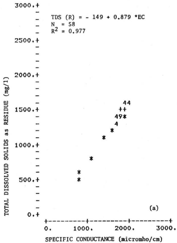
Figure A-7. Total dissolved solids - specific conductance data used in regression analysis, South Platte River at Balzac.
