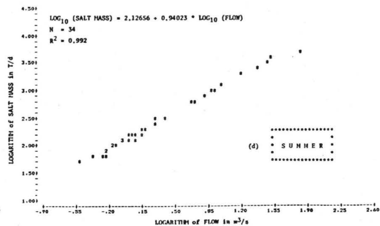
Figure B-8. Salinity mass - flow data used in regression analysis, South Platte River at Julesburg.
