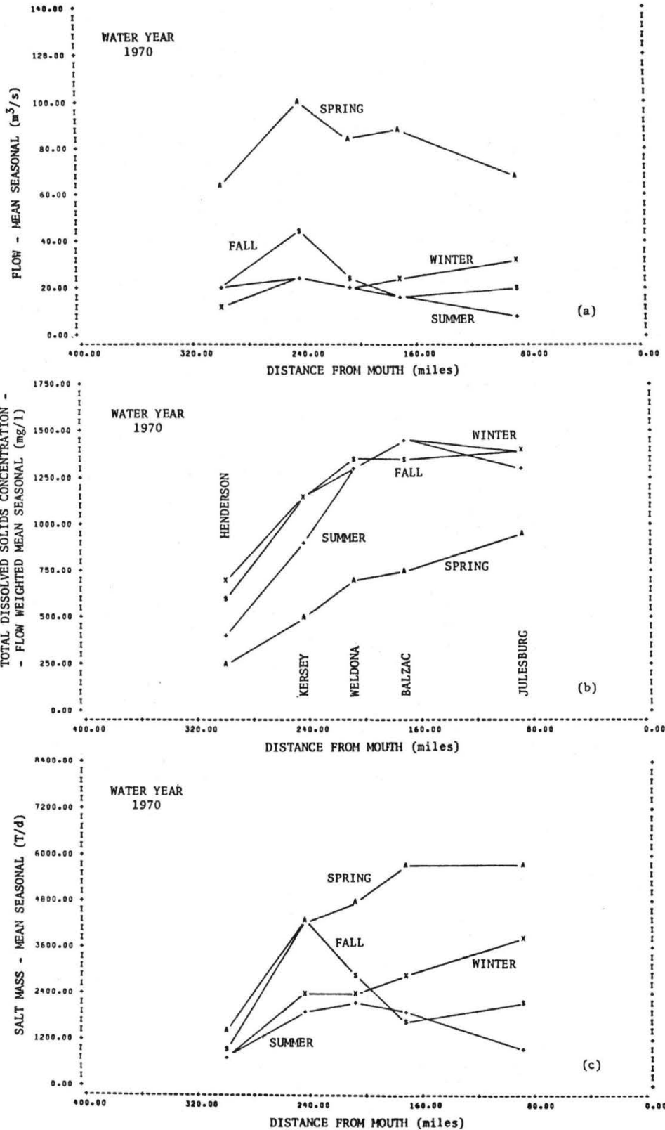
Figure D-6. Distance profiles of flow, salt concentration and salt mass flow averaged by season, South Platte River, water year 1970.
