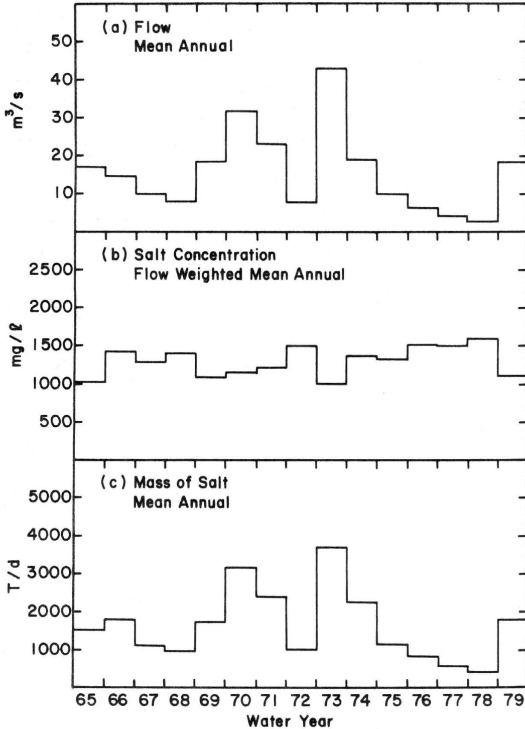
Figure 4-2. Flow, salt concentration, and salt mass flow averaged by year, water years 1965-79, South Platte River at Julesburg.
