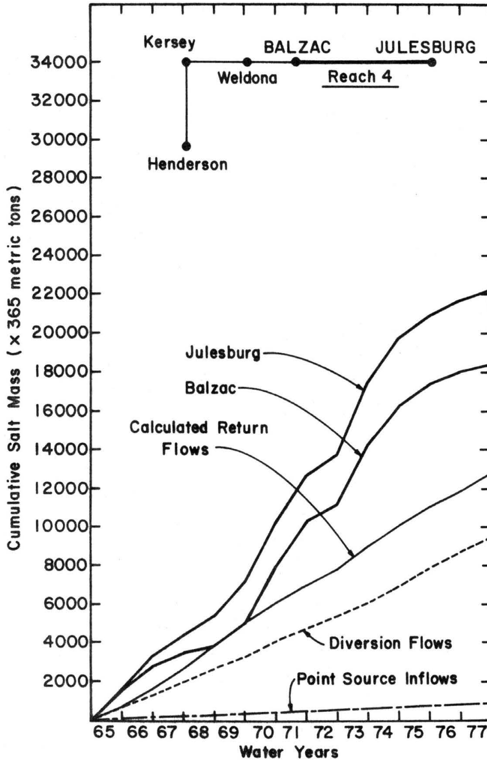
Figure 4-16. Cumulative salt mass to and from Balzac-Julesburg reach, South Platte River, water years 1965-77.
