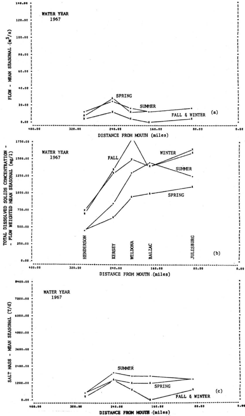
Figure D-3. Distance profiles of flow, salt concentration and salt mass flow averaged by season, South Platte River, water year 1967.
