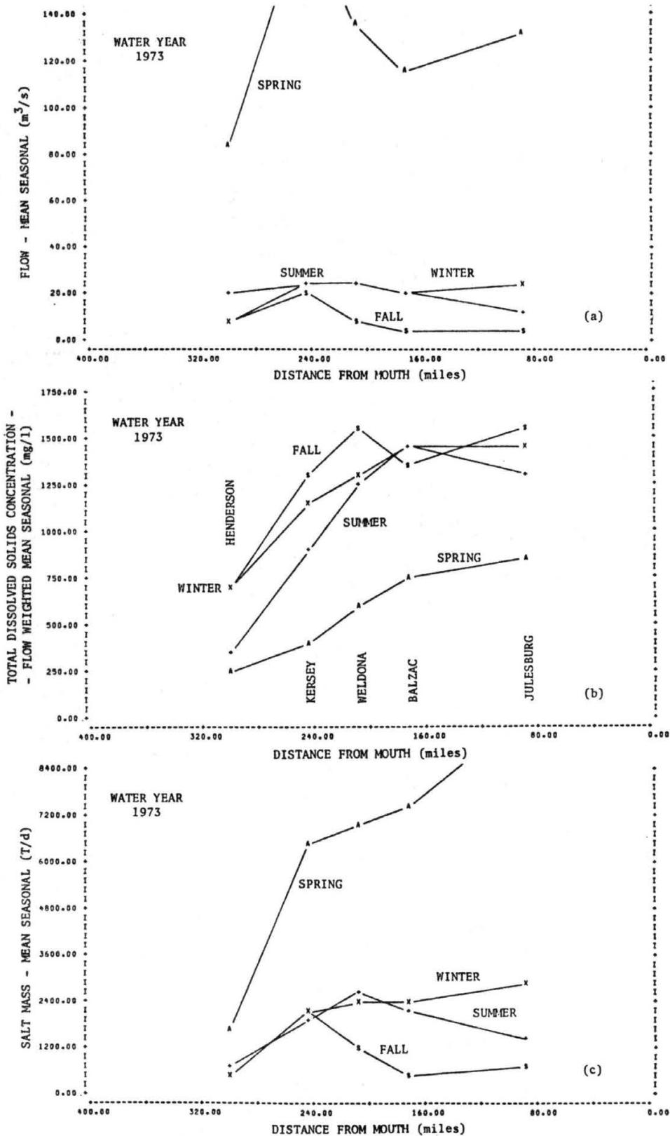
Figure D-9. Distance profiles of flow, salt concentration and salt mass flow averaged by season, South Platte River, water year 1973.
