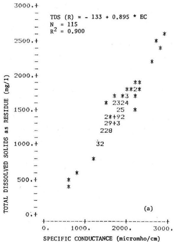
Figure A-6. Total dissolved solids - specific conductance data used in regression analysis, South Platte River near Weldona.
