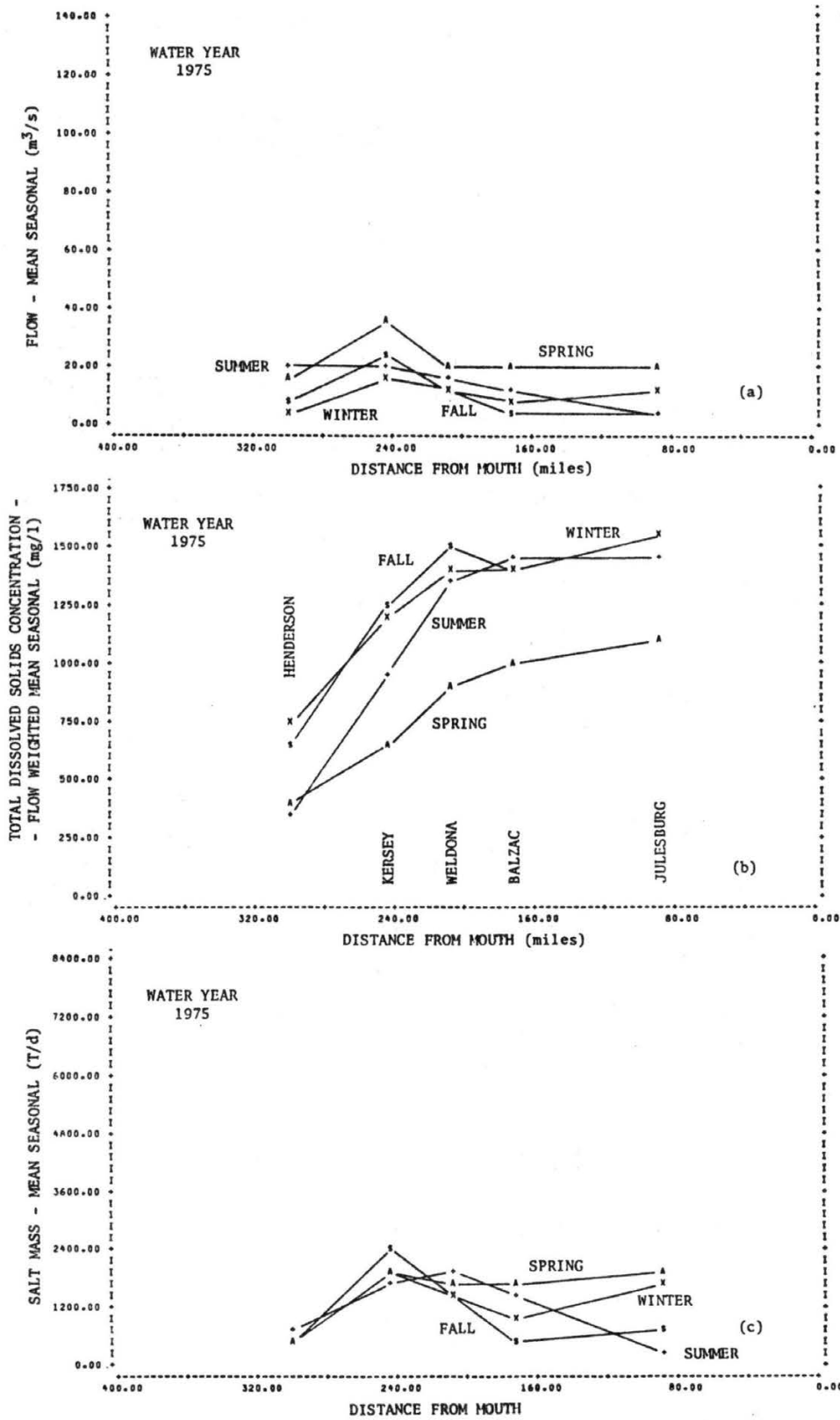
Figure D-11. Distance profiles of flow, salt concentration and salt mass flow averaged by season, South Platte River, water year 1975.
