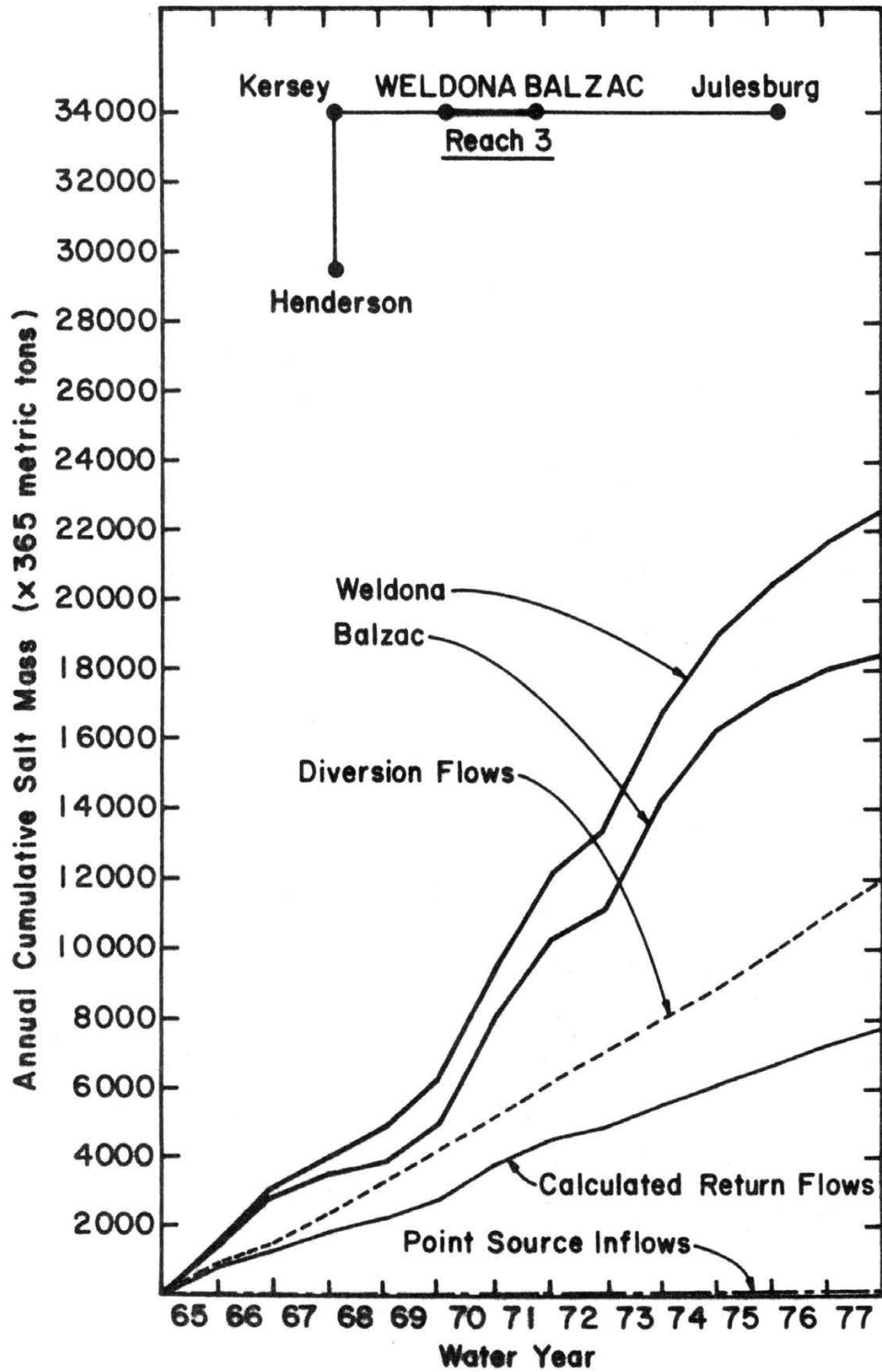
Figure 4-14. Cumulative salt mass to and from Weldon-Balzac reach, South Platte River, water years 1965-77.
