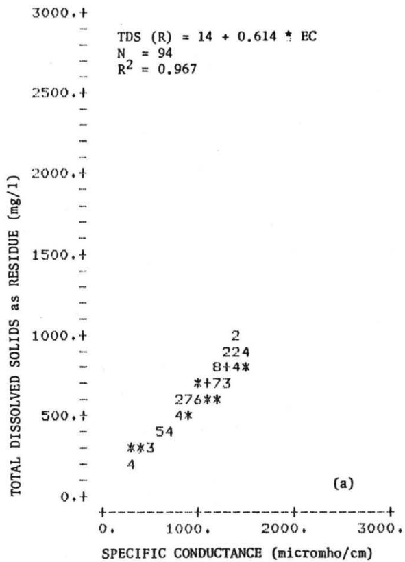
Figure A-1. Total dissolved solids - specific conductance data used in regression analysis, South Platte River at Henderson.
