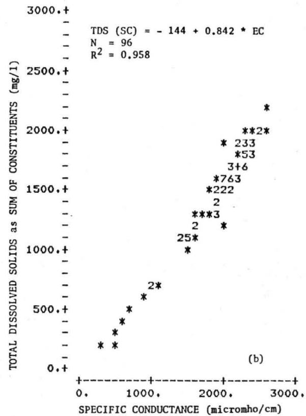
Figure A-3. Total dissolved solids - specific conductance data used in regression analysis, Big Thompson River near La Salle.
