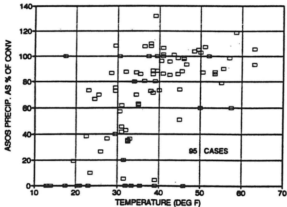
Figure 5. ASOS precipitation as a percent of CONV precipitation plotted as a function of temperature for each storm event, November 1993 through March 1994, with at least 0.10" of CONV precipitation within 36 hours for all 13 commissioned CDCP sites in the Central U.S.
