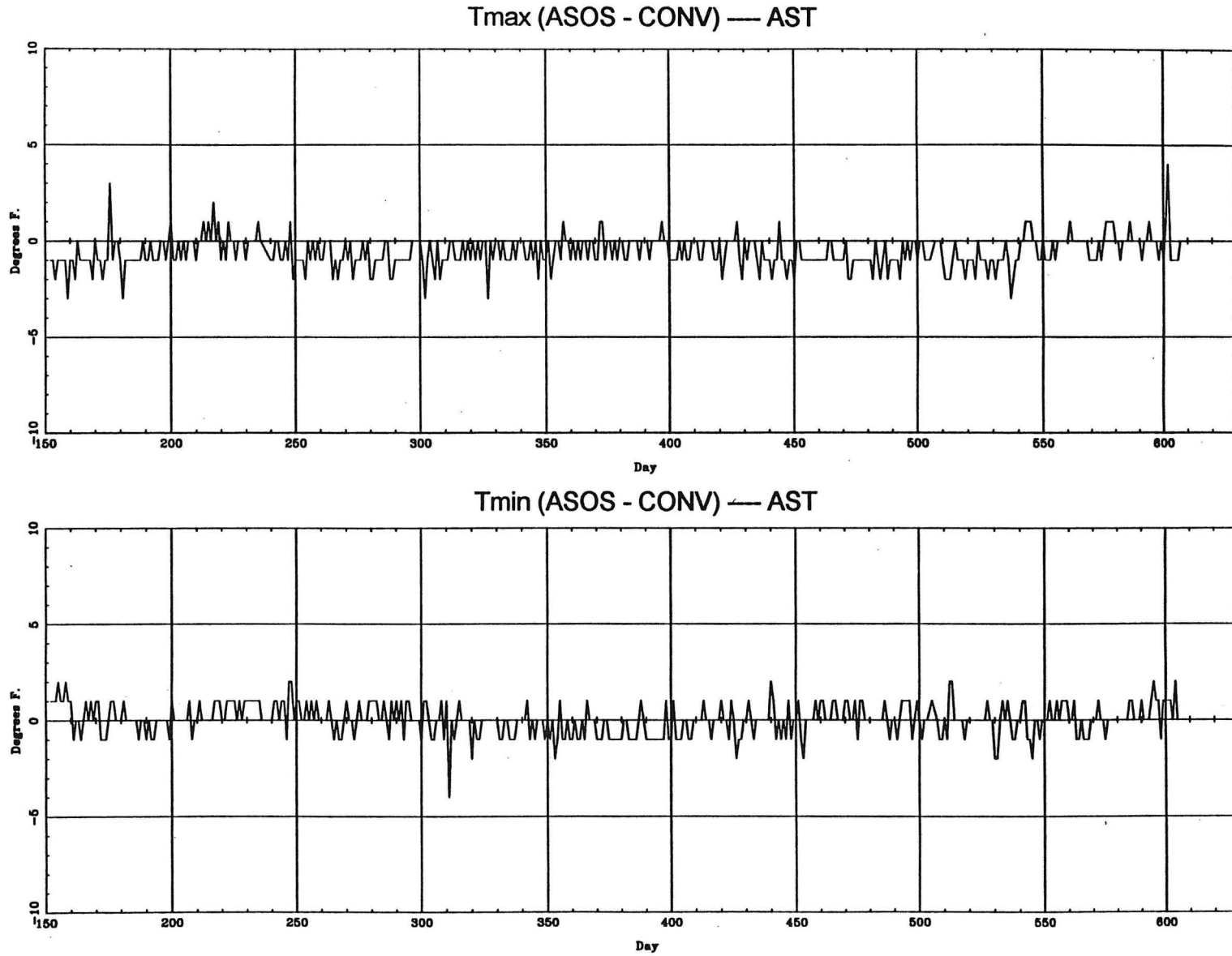
Figure 11b. Temperature time series of ASOS-CONV for maximum and minimum from June 1994 through August 1995 for AST.
