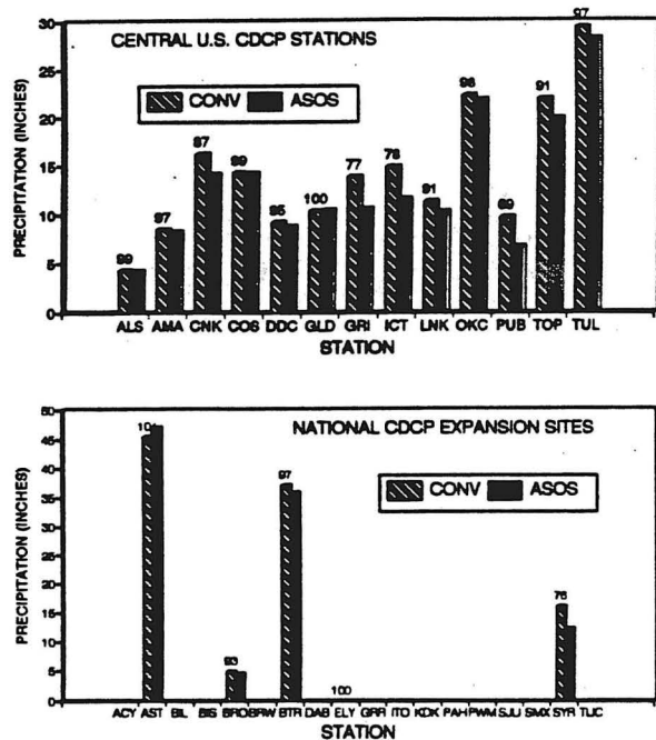
Figure 4. Comparison of total cumulative CONV and ASOS precipitation from September 1993 or date of commissioning (if after Sep. 1993) through June 1994 for each CDCP site in the Central U.S. (top) and national expansion sites (bottom). The number above the bars shows ASOS precipitation as a percent of CONV for each site.
