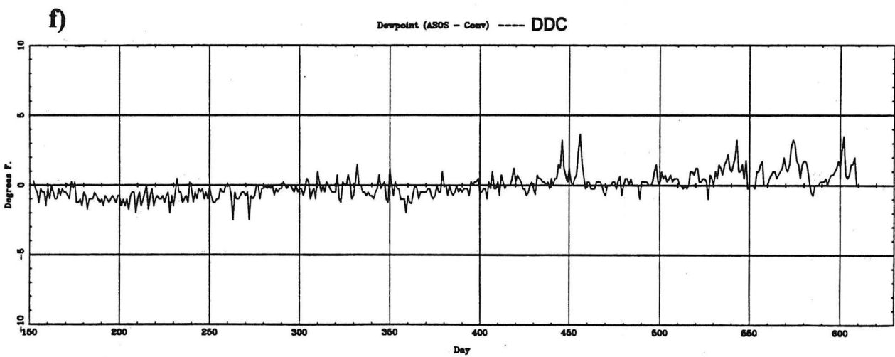
Figure 13d-e. Dewpoint temperature time series for daily average of 6 hourly ASOS-CONV observation for June 1994 through August 1995 for d) BTR, e) COS , f) DDC.
