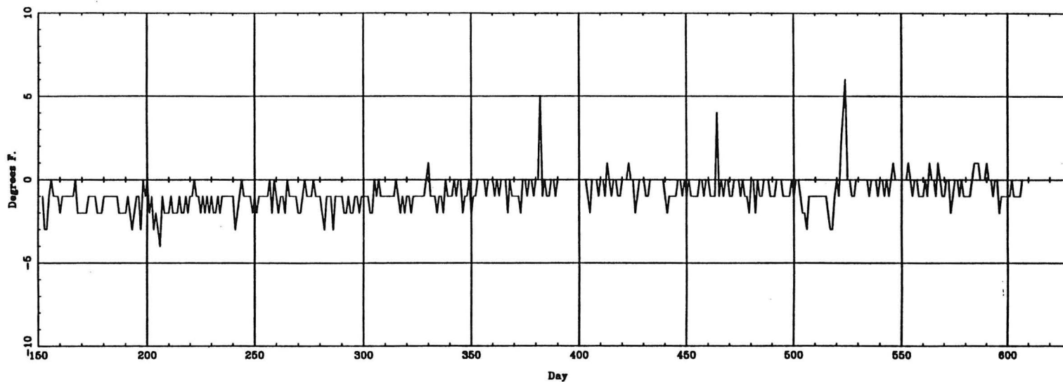
Tmin (ASOS - CONV) — ICT
