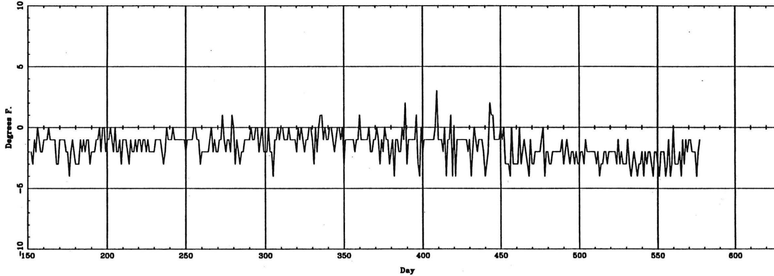
Tmin (ASOS - CONV) — TUL
