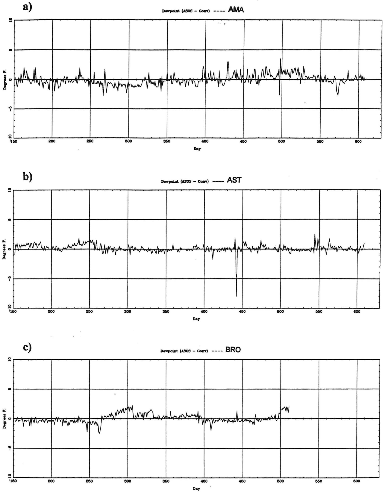
Figure 13a-c. Dewpoint temperature time series for daily average of 6 hourly ASOS-CONV observation for June 1994 through August 1995 for a) AMA, b) AST, c) BRO.
