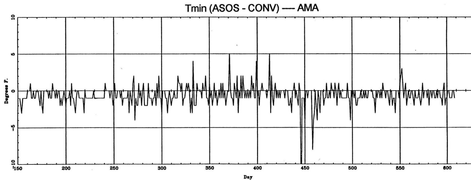
Figure 11a. Temperature time series of ASOS-CONV for maximum and minimum from June 1994 through August 1995 for AMA.
