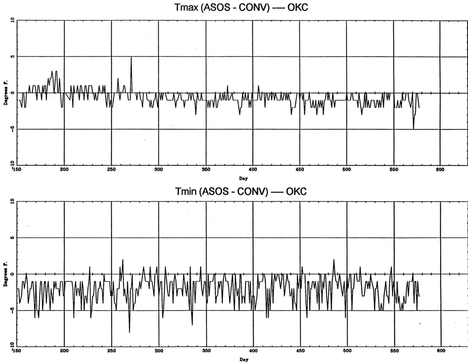
Figure 11k. Temperature time series of ASOS-CONV for maximum and minimum from June 1994 through August 1995 for OKC.
