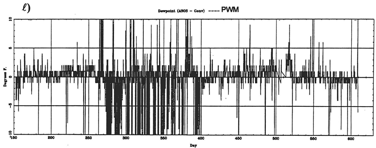
Figure 12j-l. Dewpoint temperature time series for 6 hourly ASOS-CONV observations for June 1994 through August 1995 for j) LNK, k) OKC, l) PWM.
