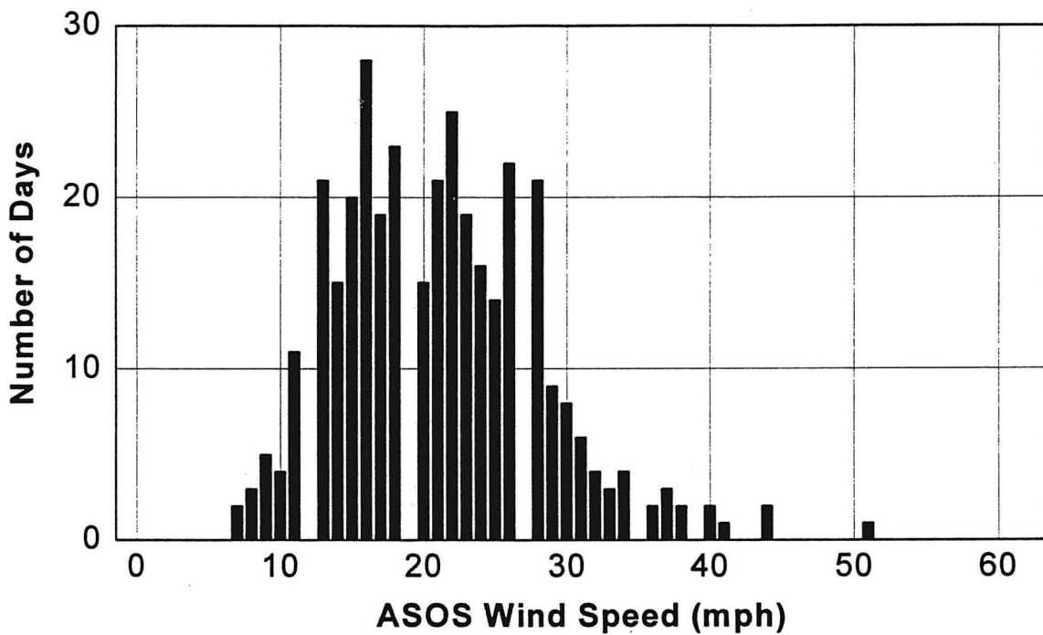
Figure 6 Maximum 2-Minute Average at Billings (9/94-8/95)
