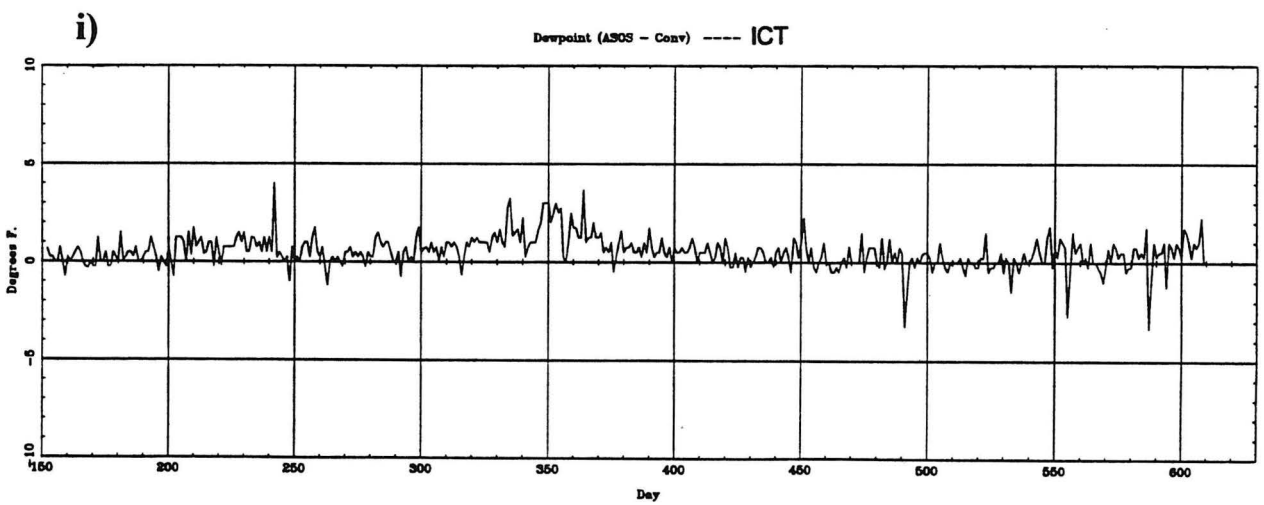
Figure 13g-i. Dewpoint temperature time series for daily average of 6 hourly ASOS-CONV observation for June 1994 through August 1995 for g) GLD, h) GRI, i) ICT.
