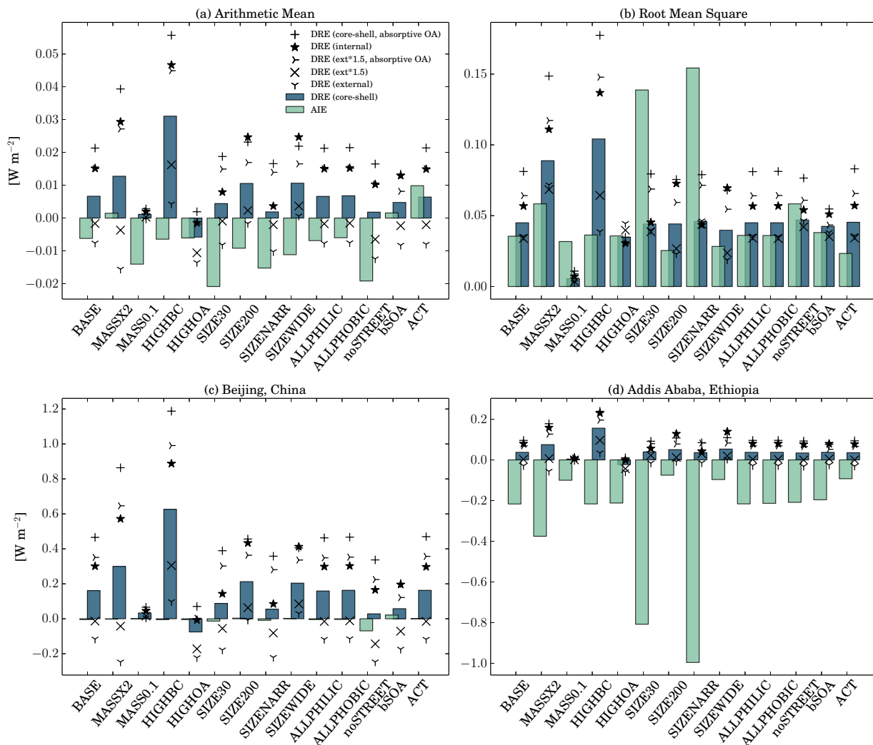
FIGURE 1.2. The DRE and AIE of biofuel aerosol (relative to a NOBIOF simulation) for each simulation as (a) a global arithmetic mean, (b) global root mean square, (c) the value over Beijing, China, (d) the value over Addis Ababa, Ethiopia. The various symbols show alternate mixing state assumptions.
