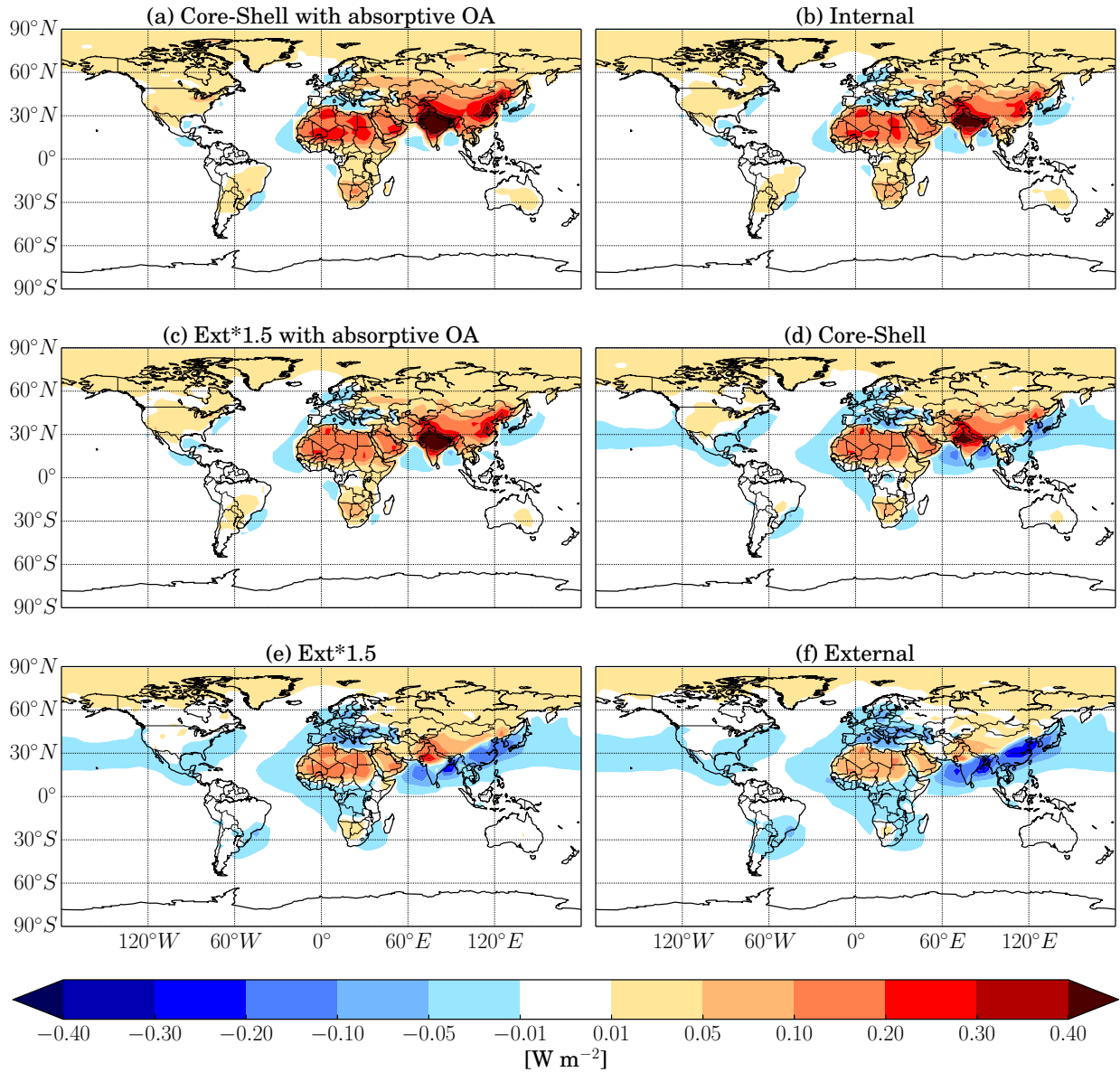
FIGURE 1.6. The DRE for the BASE-NOBIOF comparison assuming a core-shell with absorptive (a) OA (mean: 0.021 \text{ W m}^{-2} ), (b) internal (mean: 0.015 \text{ W m}^{-2} ), (c) ext*1.5 with absorptive OA (mean: 0.015 \text{ W m}^{-2} ), (d) core-shell (mean: 0.007 \text{ W m}^{-2} ), (e) ext*1.5 (mean: -0.002 \text{ W m}^{-2} ), and (f) external (mean: -0.008 \text{ W m}^{-2} ) mixing state.
