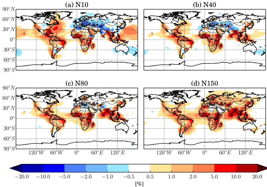
FIGURE 1.4. The annual-mean percent change in boundary layer (a) N10, (b) N40, (c) N80, and (d) N150 for the BASE-NOBIOF comparison.
