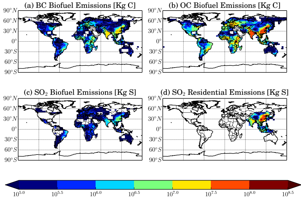
FIGURE 1.1. Annual emissions of (a) biofuel black carbon (BC) and (b) organic carbon (OC) emissions [Kg C] from Bond et al., (2007), (c) biofuel sulfur-dioxide (SO 2 ) emissions [Kg S] from EDGAR, and (d) residential SO 2 over Asia (in Kg S) from Street’s inventory.
