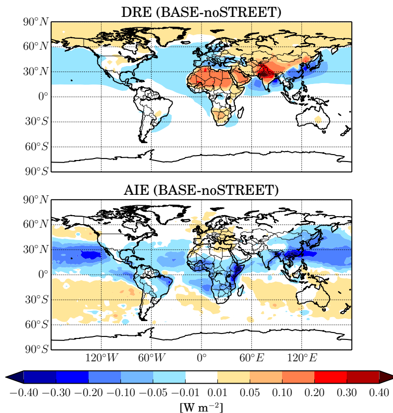
FIGURE 1.10. The DRE assuming a core-shell morphology (top, mean: 0.002 \text{ W m}^{-2} ) and the AIE (bottom, mean: -0.019 \text{ W m}^{-2} ) for the BASE-noSTREET comparison.
