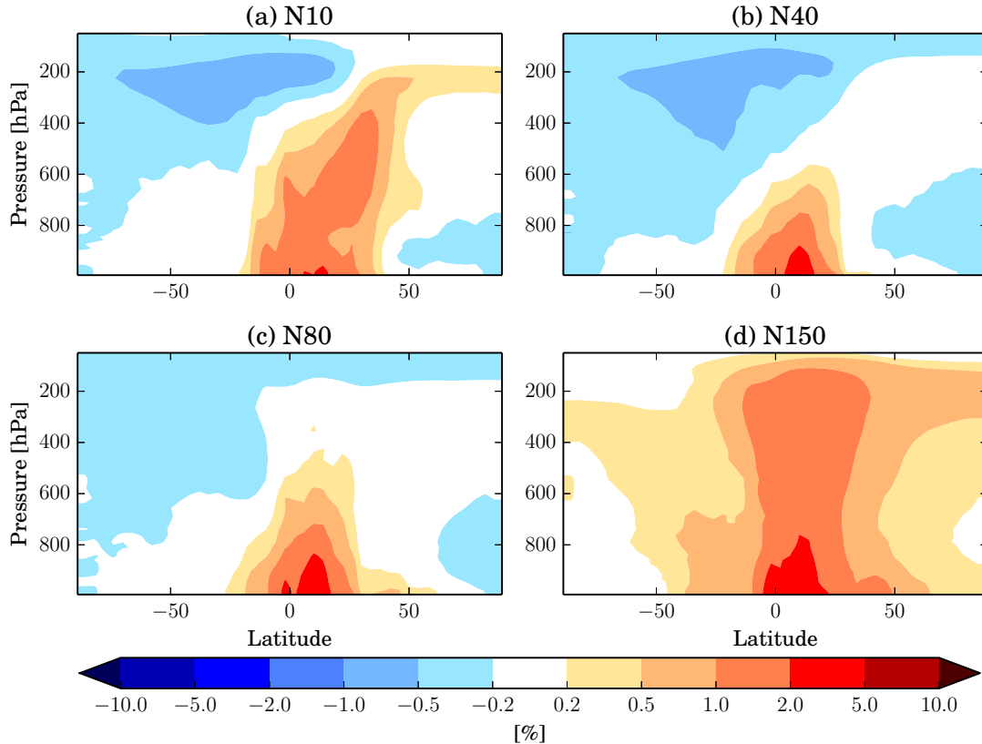
FIGURE 1.5. The annually and zonally averaged percent change throughout the troposphere for (a) N10, (b) N40, (c) N80, and (d) N150 for the BASE-NOBIOF comparison.
