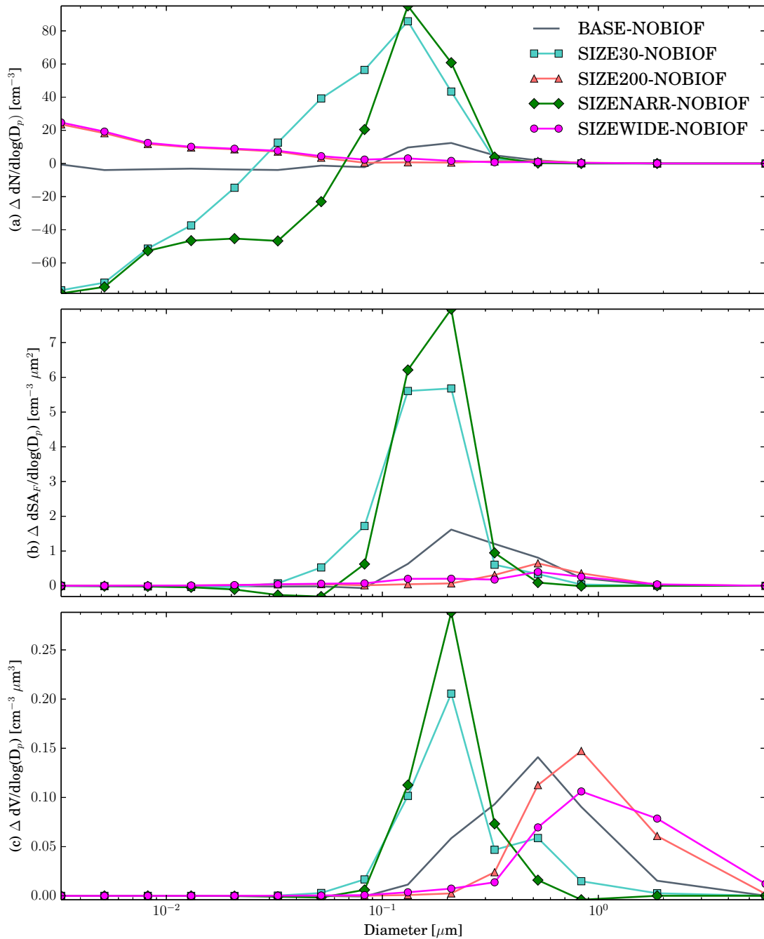
FIGURE 1.9. Globally averaged (a) change in number distribution, (b) change in Fuchs surface area distribution, and (c) change volume distribution for BASE-NOBIOF, SIZE30-NOBIOF, SIZE200-NOBIOF, SIZENARR-NOBIOF, SIZEWIDE-NOBIOF comparisons. The subtractions isolate the contributions of biofuel emissions to each distribution.
