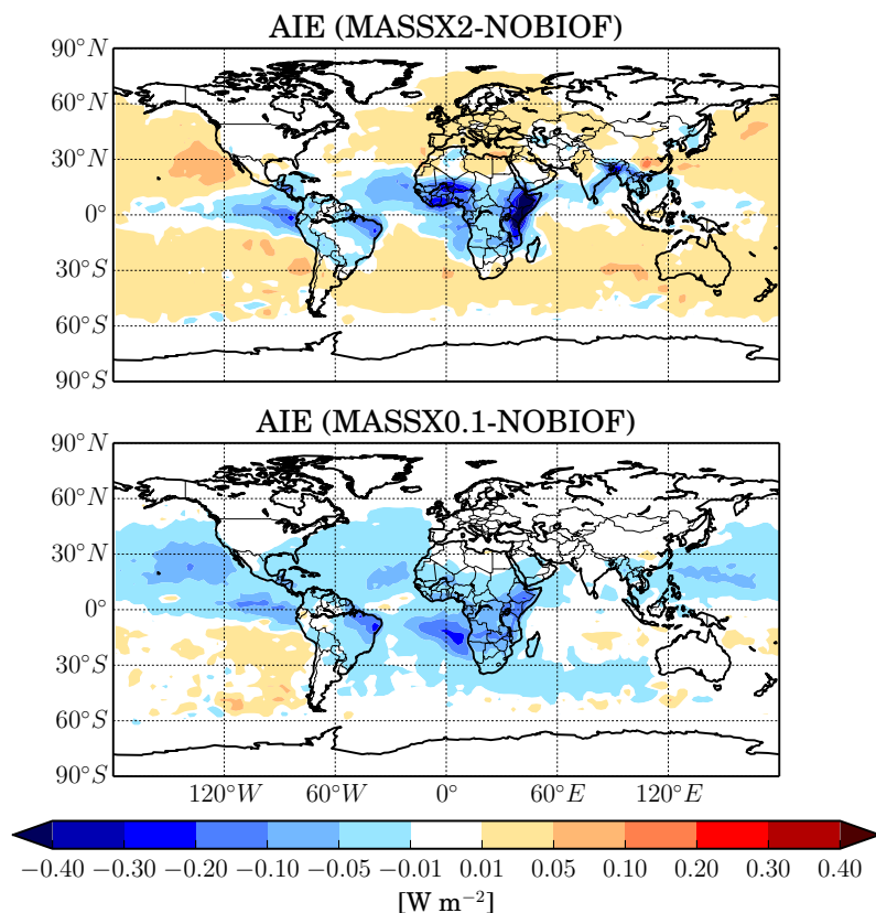
FIGURE 1.8. The AIE for the MASSX2-NOBIOF comparison (top, mean: +0.002 \text{ W m}^{-2} ) and MASSX0.1-NOBIOF comparison (bottom, mean: -0.014 \text{ W m}^{-2} ).
