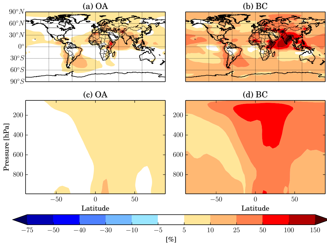
FIGURE 1.3. The percent change in boundary-layer (a) OA and (b) BC mass and (c and d) zonally-averaged with pressure for the BASE-NOBIOF comparison.
