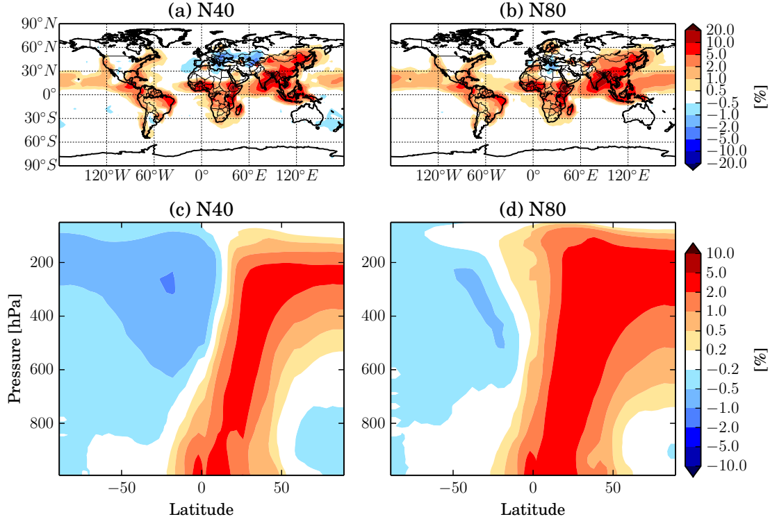
FIGURE 1.11. The percent change for the BASE-noSTREET comparison in boundary layer (a) N40 and (b) N80 and (c and d) zonally-averaged with height.
