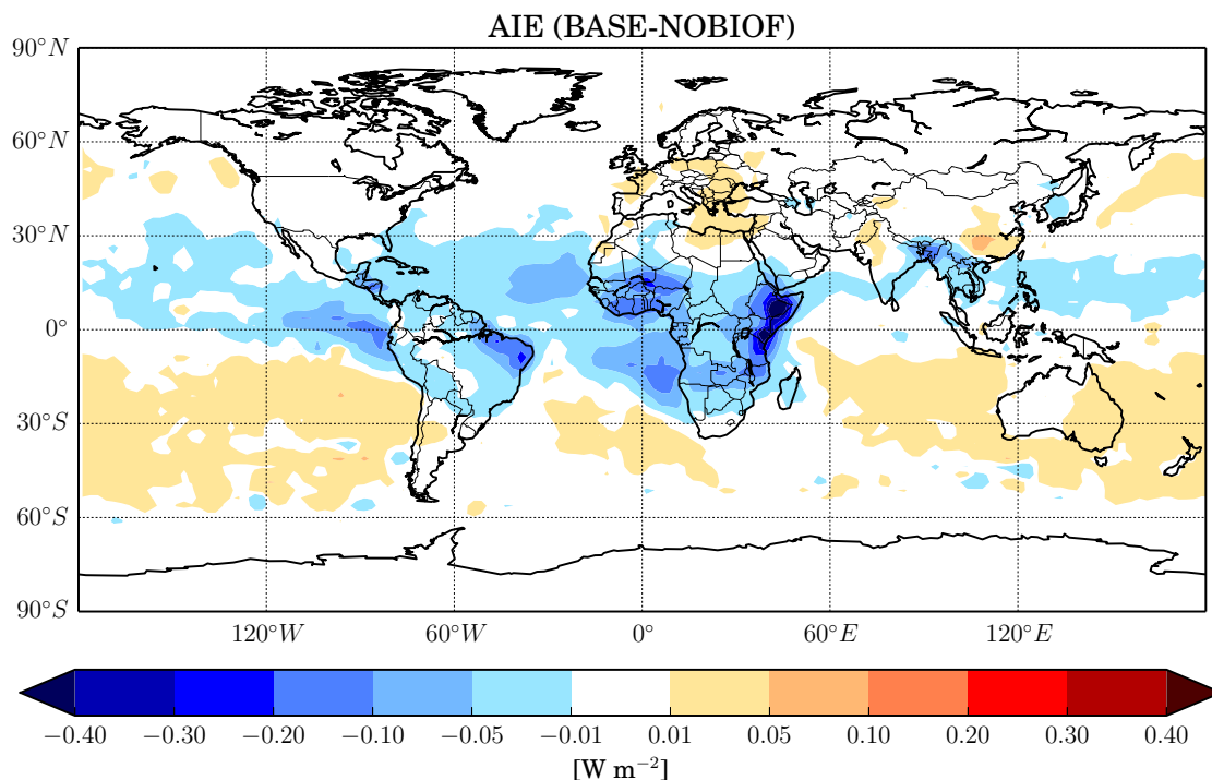
FIGURE 1.7. The cloud-albedo AIE for the BASE-NOBIOF comparison (mean: -0.006 \text{ W m}^{-2} ).
