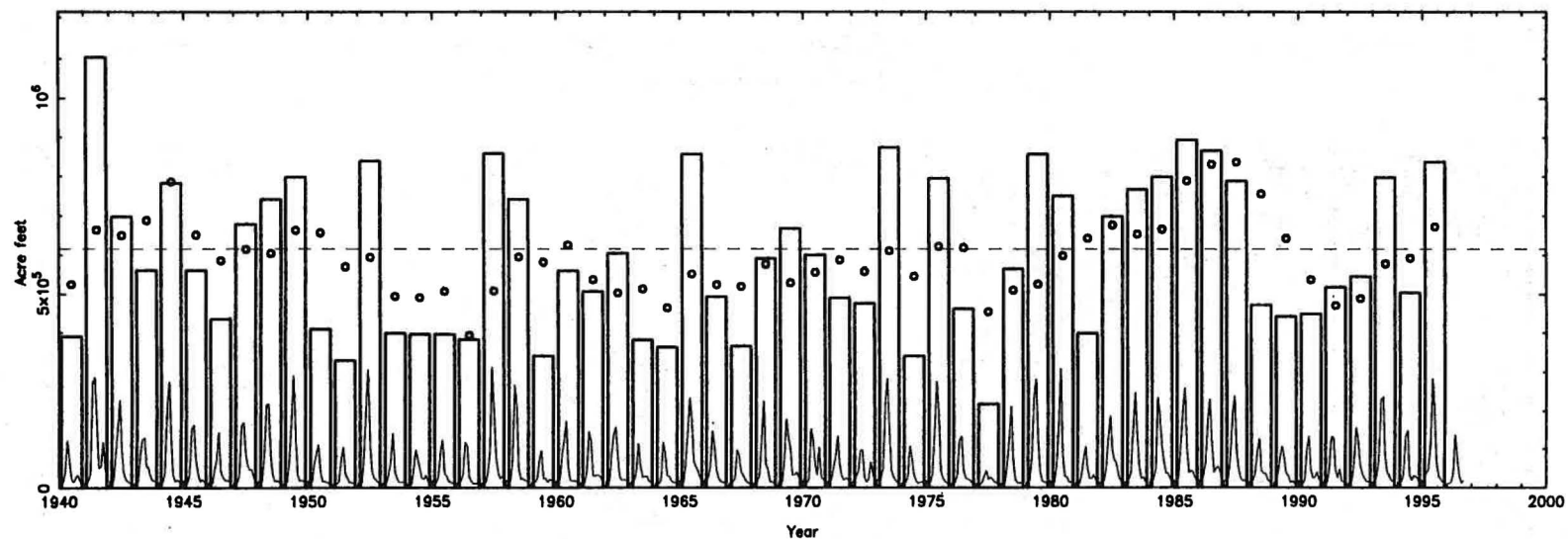
Animas River At Durango, Co.
