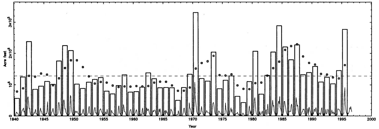
Figure 13j. Observed streamflow for South Platte river below Cheesman, Colorado.
