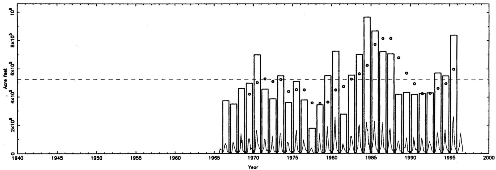
Figure 13ℓ. Observed streamflow for Arkansas river above Pueblo, Colorado.
