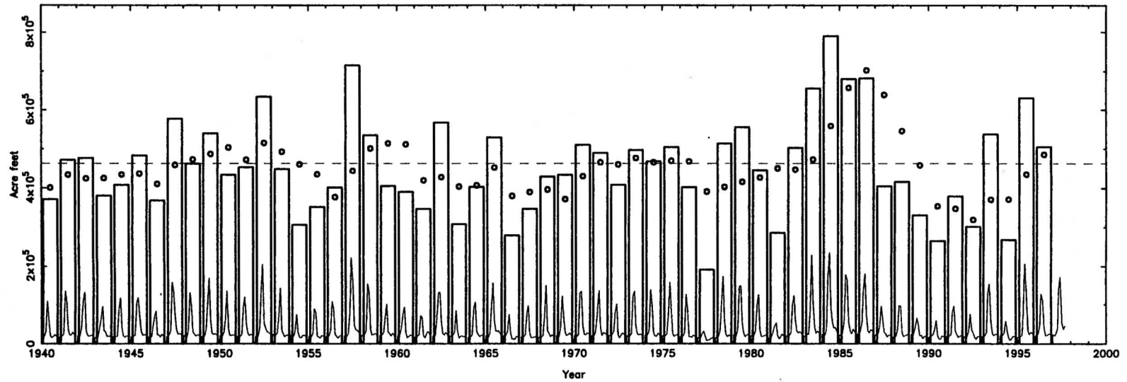
Figure 13b. Observed streamflow for White river near Meeker, Colorado.
