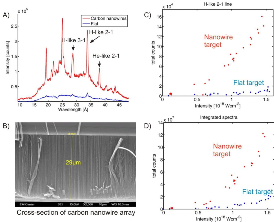
Figure 14. Soft X-ray results from vertically aligned Carbon nanowires irradiated by 350mJ pulses. A) Emission spectra obtained from laser irradiation of Carbon nanowires (red) that is compared to Carbon graphite (blue). B) SEM cross-section image of the nanowire array. Nanowires are 30nm in diameter and 29µm in length. C) A plot showing the H-like signal as a function of laser intensity for the nanowire array (red) compared to the graphite target (blue). A rapid increase in H-like production from the nanowire array can be observed as the laser intensity is increased beyond 5 \times 10^{17} \text{ Wcm}^{-2} . D) The total integrated emission in the band of 15-45nm as a function of laser intensity.
