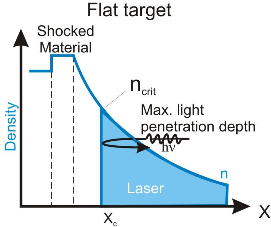
Figure 3. 1D profile of the electron density in the direction normal to a solid target surface. Light is absorption is limited to the plasma critical density, n_{crit} , where it is reflected back through the plasma. Although in most plasmas the laser light is absorbed in lower density regions and only a fraction reaches this surface. This limitation prevents directly depositing laser pulse energy into supra-critical density material.
