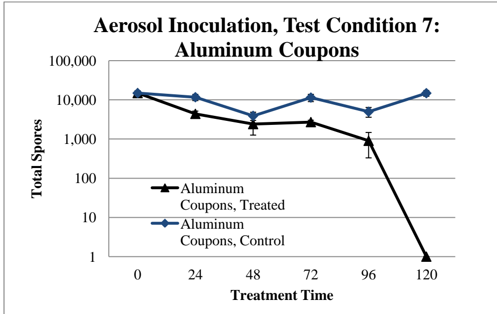
Figure 3- 10 – Decontamination tests, aerosol deposition, test condition 7
