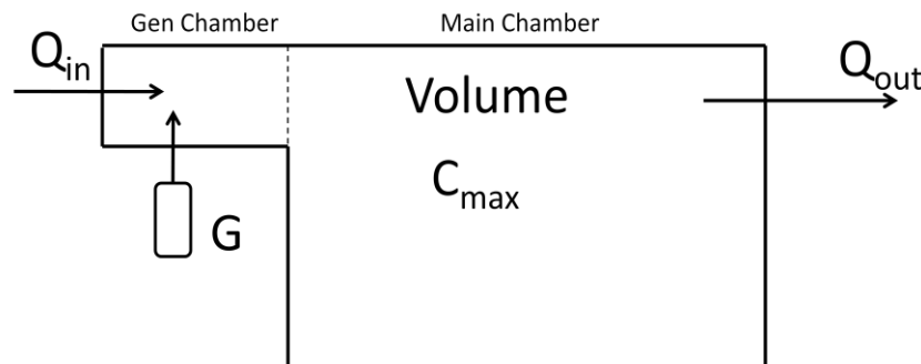
Figure 3- 1 – Test chamber deposition model
