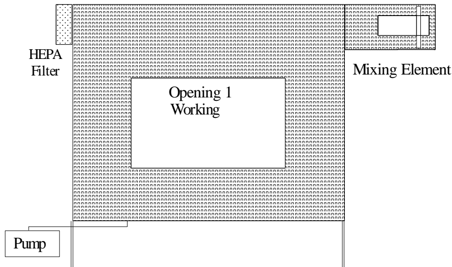
Figure 2- 1 – Test chamber, working side
