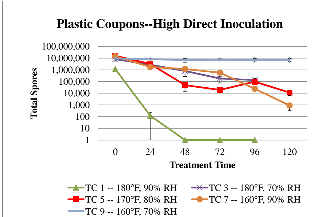
Figure 4- 2 – Decontamination tests, high direct inoculation
