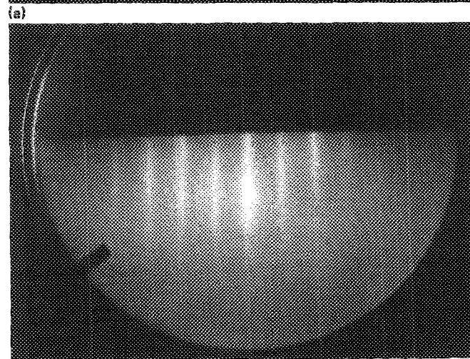
FIG. 3. RHEED patterns for \text{FeSi}_2 grown by deposition of 100 \text{ \AA} of iron at 450^\circ\text{C} with the incident electron beam along (a) \text{Si}(110) and (b) \text{Si}(100) .
