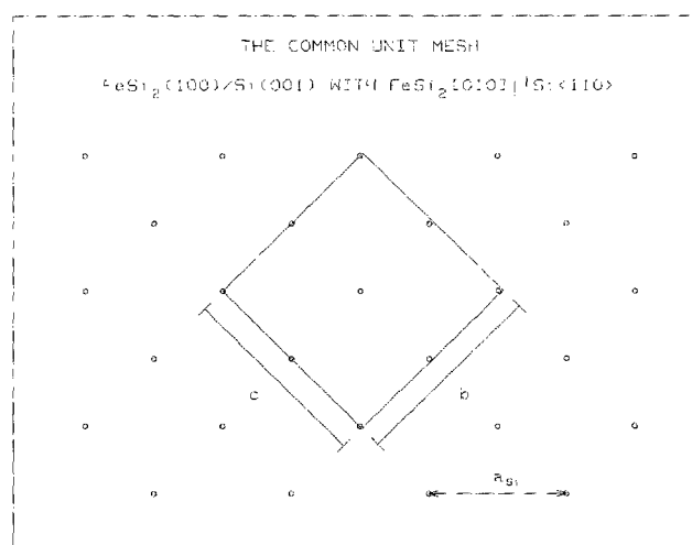
FIG. 1. Proposed heteroepitaxial relationship and common unit mesh for beta- \text{FeSi}_2 and the (001) silicon face. It is the relative orientation that is suggested; the relative position is merely assumed.
