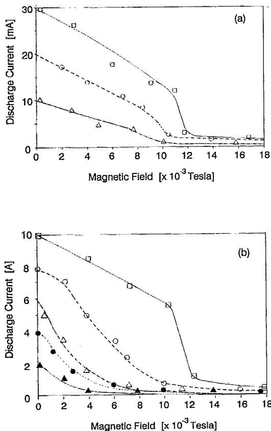
FIG. 3. Variation of the dc (a) and pulsed (b) discharge current as a function of the applied magnetic field for several initial values of the discharge current. The helium pressure was 1.3 and 2.4 Torr, respectively.
