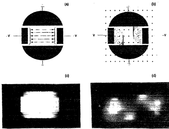
FIG. 1. Cross-sectional view of the HCD schematically illustrating the trajectory of the beam electrons: (a) without, and (b) with magnetic field applied; (c) and (d) are end-on photographs of the glow discharge for H=0 and H=0.018 T, respectively. The helium pressure was 1.2 Torr and the voltage drop across the discharge with the field applied was 1.96 kV.
