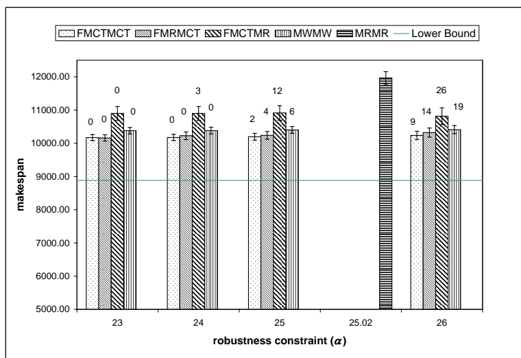
Fig. 3 Simulation results of makespan for different values of robustness constraint ( \alpha ) for pseudo-batch mode heuristics for HIHI heterogeneity.
