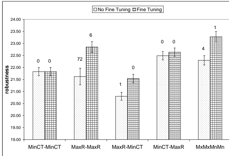
Fig. 6 Average robustness value (over all mapping events) for the LOLO case with \gamma = 12500 .
