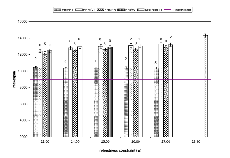
Fig. 1 Simulation results of makespan for different values of robustness constraint ( \alpha ) for immediate mode heuristics for HHH heterogeneity.
