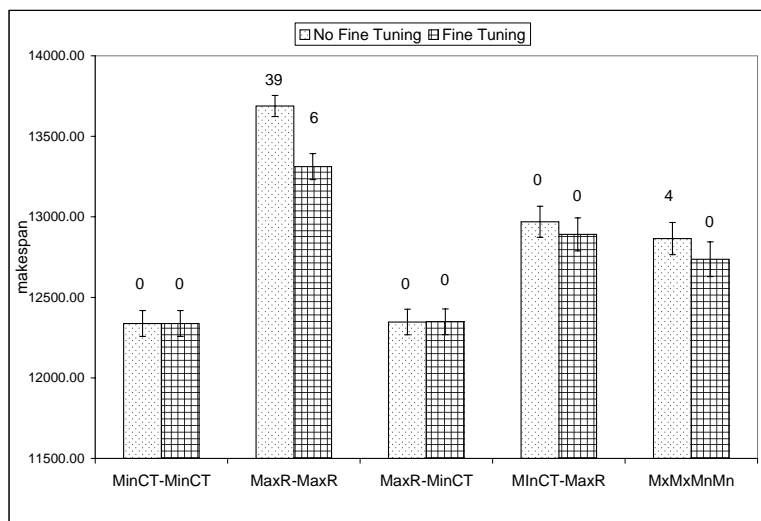
Fig. 7 Average makespan for the HIHI case with \gamma = 14000 .
