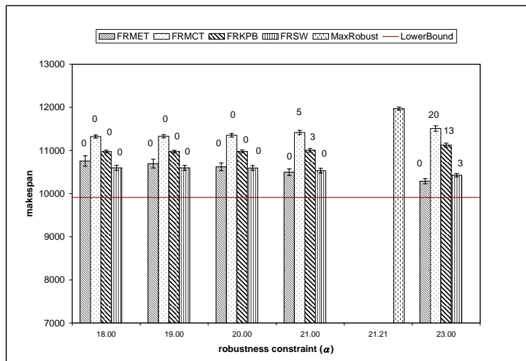
Fig. 2 Simulation results of makespan for different values of robustness constraint ( \alpha ) for immediate mode heuristics for LOLO heterogeneity.
