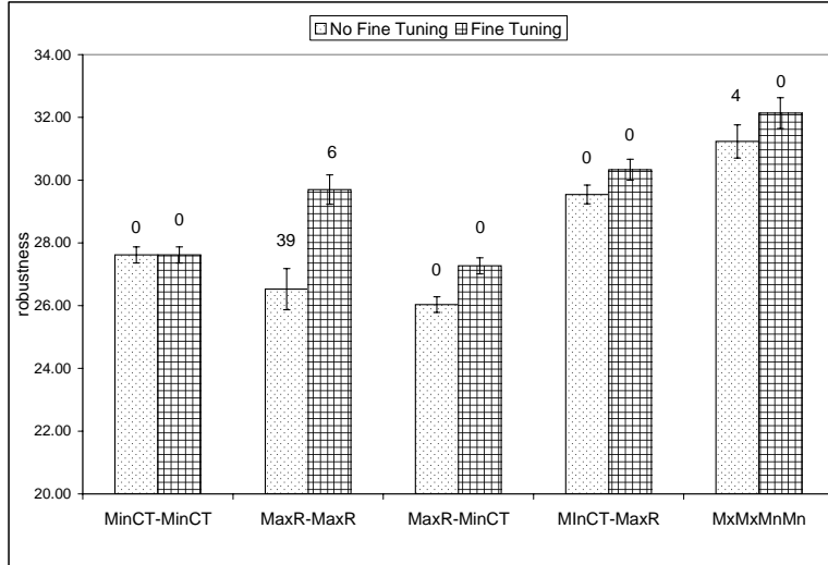
Fig. 5 Average robustness value (over all mapping events) for the HIHI case with \gamma = 14000 .
