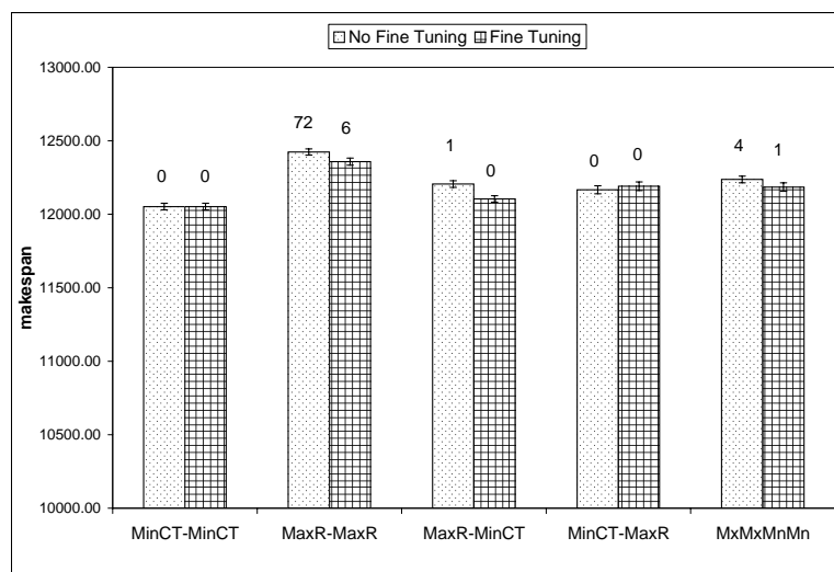
Fig. 8 Average makespan for the LOLO case with \gamma = 12500 .
