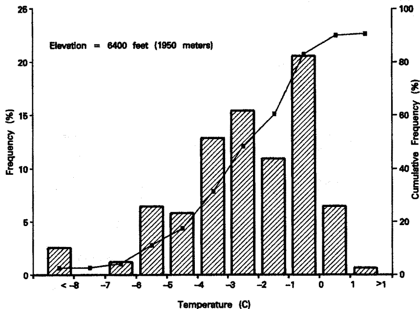
Figure 2. TEMPERATURE DISTRIBUTION
