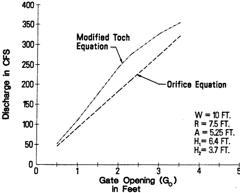
Fig. 5. Flow Equation Comparison
