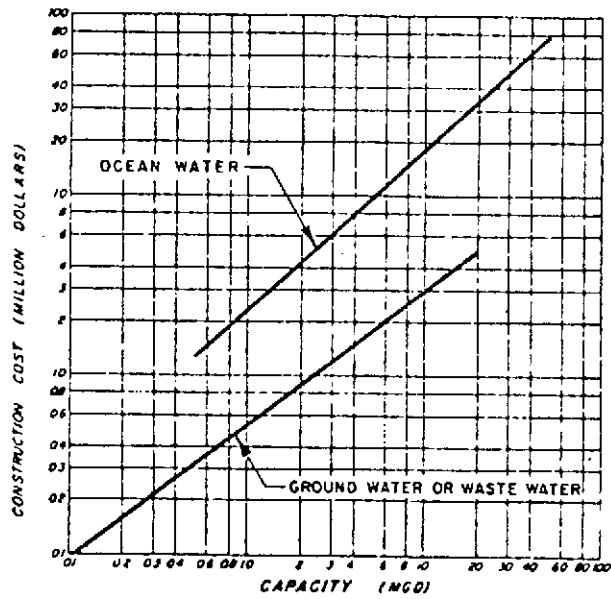
Figure D-4. Construction Cost of Demineralization (ENR=2000) 6
