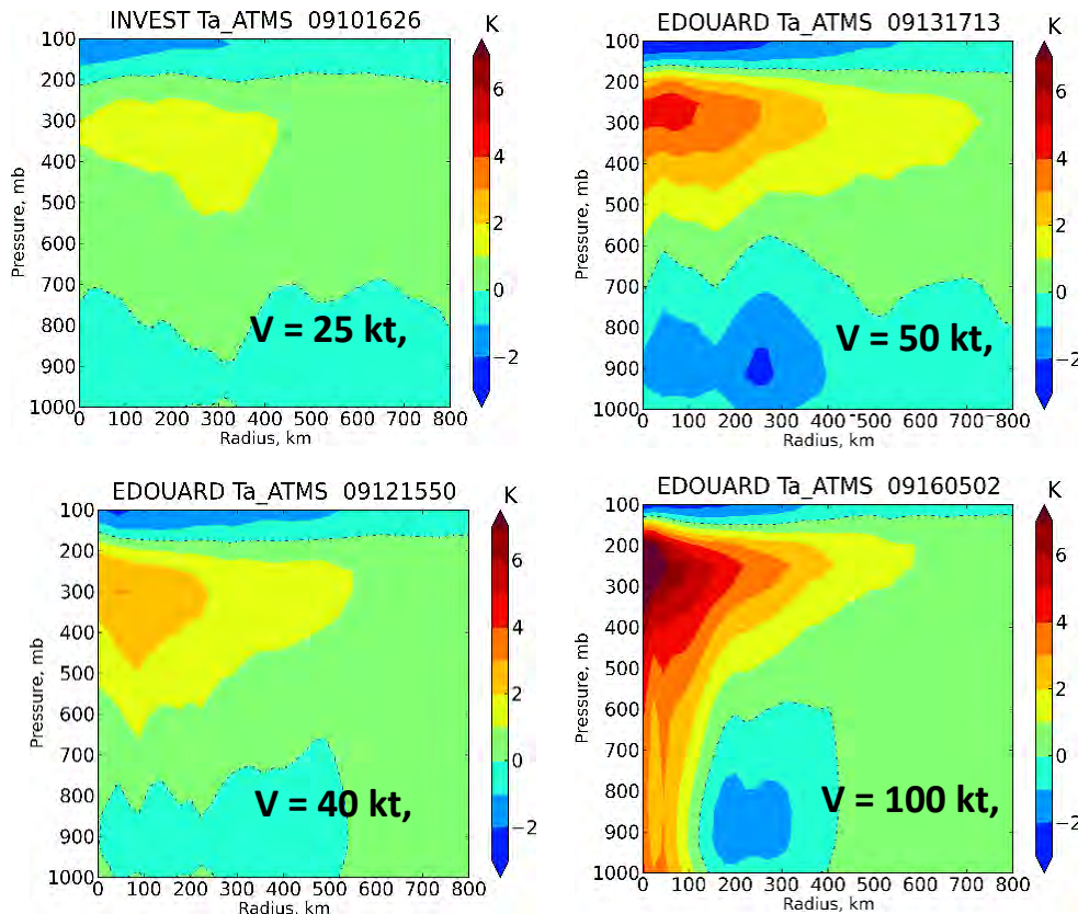
Figure 13. Azimuthally-averaged vertical temperature cross-section for Hurricane Edouard, a062014 for four different times, and the corresponding intensity change from the ATCF Best Track.
