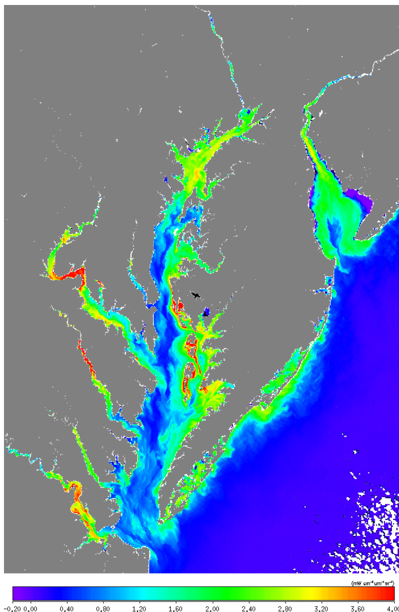
Figure 1. VIIRS I1 band normalized water-leaving radiance nLw(638) in Delmarva region on April 3, 2016 at 18:01 UTC.
