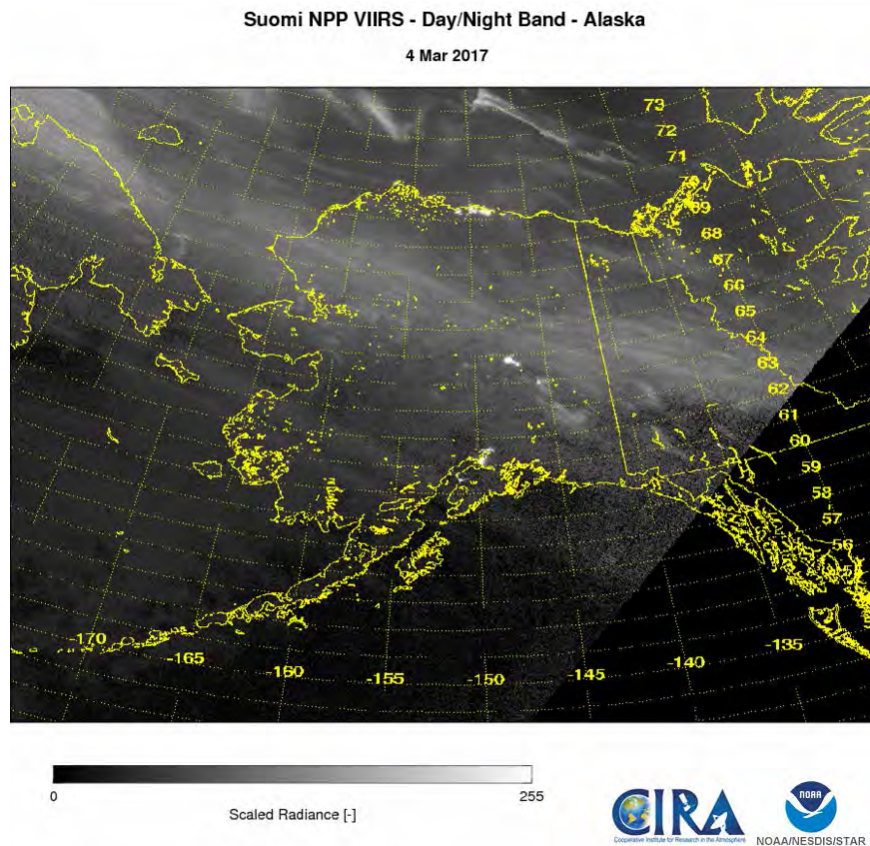
Figure 2. Example DNB image provided to the STAR JPSS LTM website (4 March 2017).
