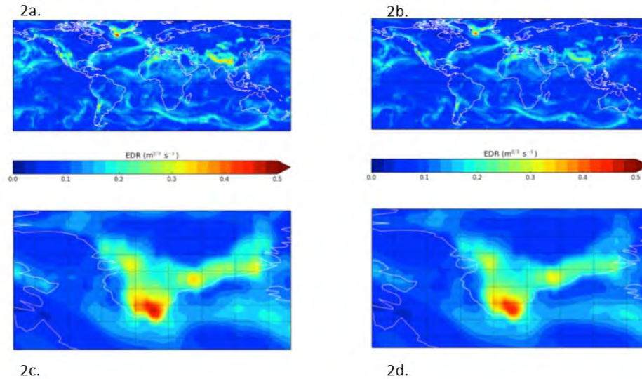
Figure 2. Global (2 a,b) and regional (2 c,d; zoomed in Greenland area) for the blended maximum (2 a,c) and mean (2 b,d) EDR from GFS GTG and UM GTG valid at 18 UTC 6 Jan 2016.
