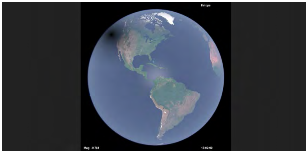
Figure 1. Simulated view of the central portion of the moon's shadow off the northwest US coastline during this summer's solar eclipse.
