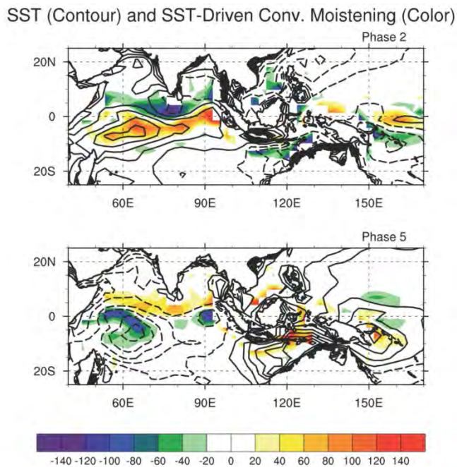
Figure 6. SST anomalies (contours) and SST-driven moisture convergence anomalies (colors) for Phases 2 and 5 of the MJO in the SPCCSM. The SST contour interval is 0.05^{\circ}C , and the units of convergence anomalies are W m^{-2} . Note that the convergence anomalies have been converted to energy units to reflect latent heat convergence.
