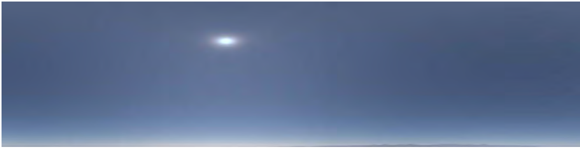
Figure 4. Simulated clear sky
