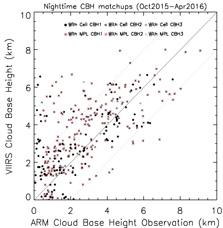
Figure 7. Initial evaluation results for nighttime CBH algorithm performance using ARM ceilometer data from the NSA site. The brown/red symbols represent comparisons with ARM MPL CBHs and black/gray circles are ARM ceilometer CBHs (black for the first layer and gray for the second layer). CBH measurements are considered only when CTHs from MPL and VIIRS are within 2-km error range.
