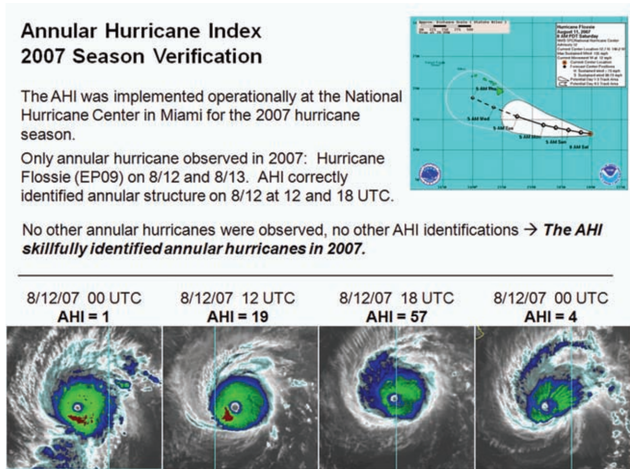
Figure 3. Slide showing the performance of the Annular Hurricane Index (AHI) during Hurricane Flossie (2007). The track of Flossie is shown in the upper right. Individual IR images are shown with the valid time and the AHI value. The AHI can range from 0 (not an annular hurricane) to 100 (the highest probability of being an annular hurricane).
