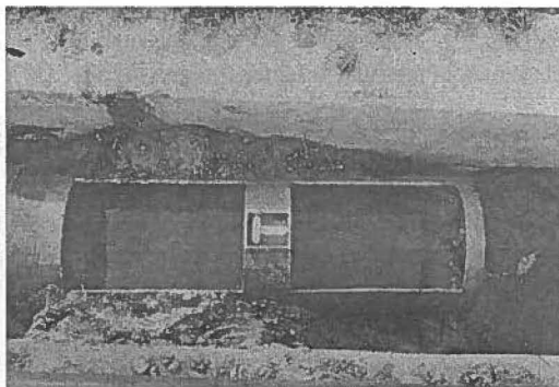
Figure 10. Portable Flume Constructed in a Section of Circular Pipe.
