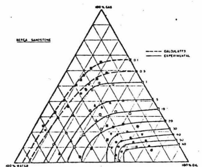
FIG. 4—OIL ISOPERMS.
