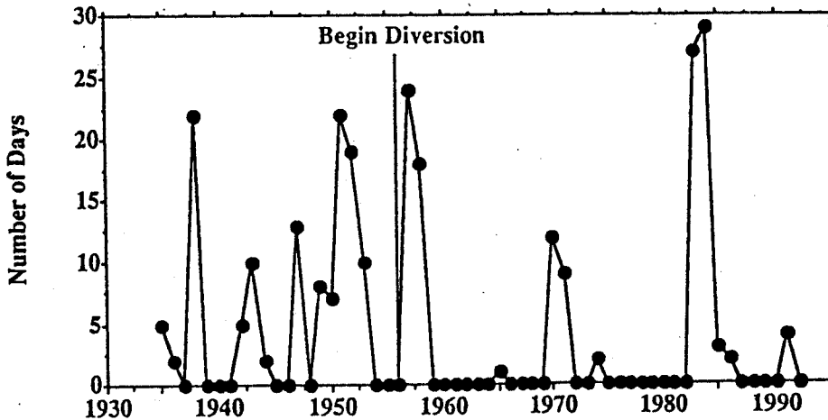
Figure 5. Change in total number of consecutive days bankfull flow reached or exceeded at St. Louis Creek. Bankfull estimated using 1.5 year return interval of 6.4 m³ s⁻¹. Average number of days exceeded in unaltered period is 5.95.
