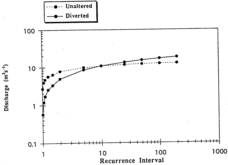
Figure 4. Flood frequency curves calculated using unaltered and diverted flow data from USGS gage at St. Louis Creek (09026500).
